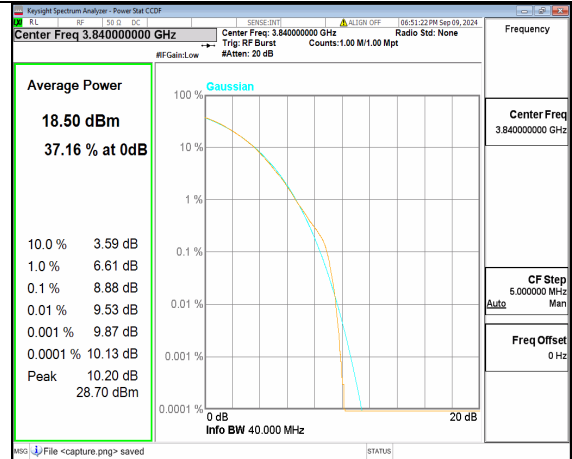
n77(3700-3980MHz) 40M CP-OFDM 256QAM Outer_Full Mid
