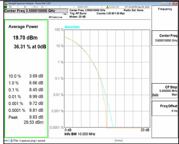
n78(3450-3550MHz) 10M CP-OFDM 256QAM Outer_Full Mid
