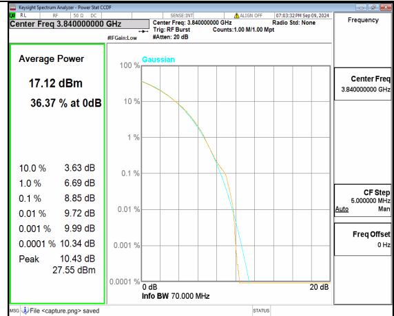
n77(3700-3980MHz) 70M CP-OFDM 256QAM Outer_Full Mid
