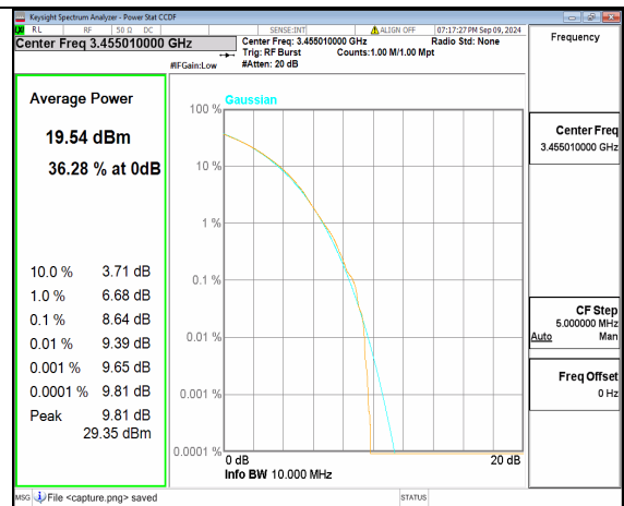
n78(3450-3550MHz) 10M CP-OFDM 256QAM Outer_Full Low
