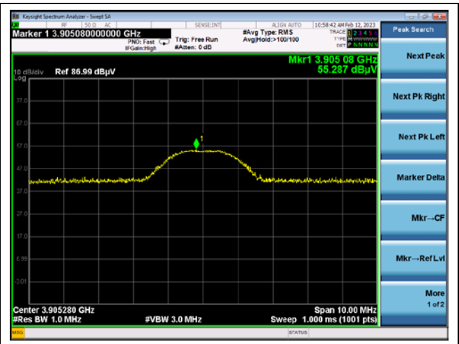
9 th harmonic
