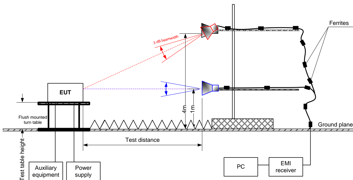
Figure 8.2.2 Setup for radiated emission measurements in 1000 – 2300 MHz range, table-top EUT
