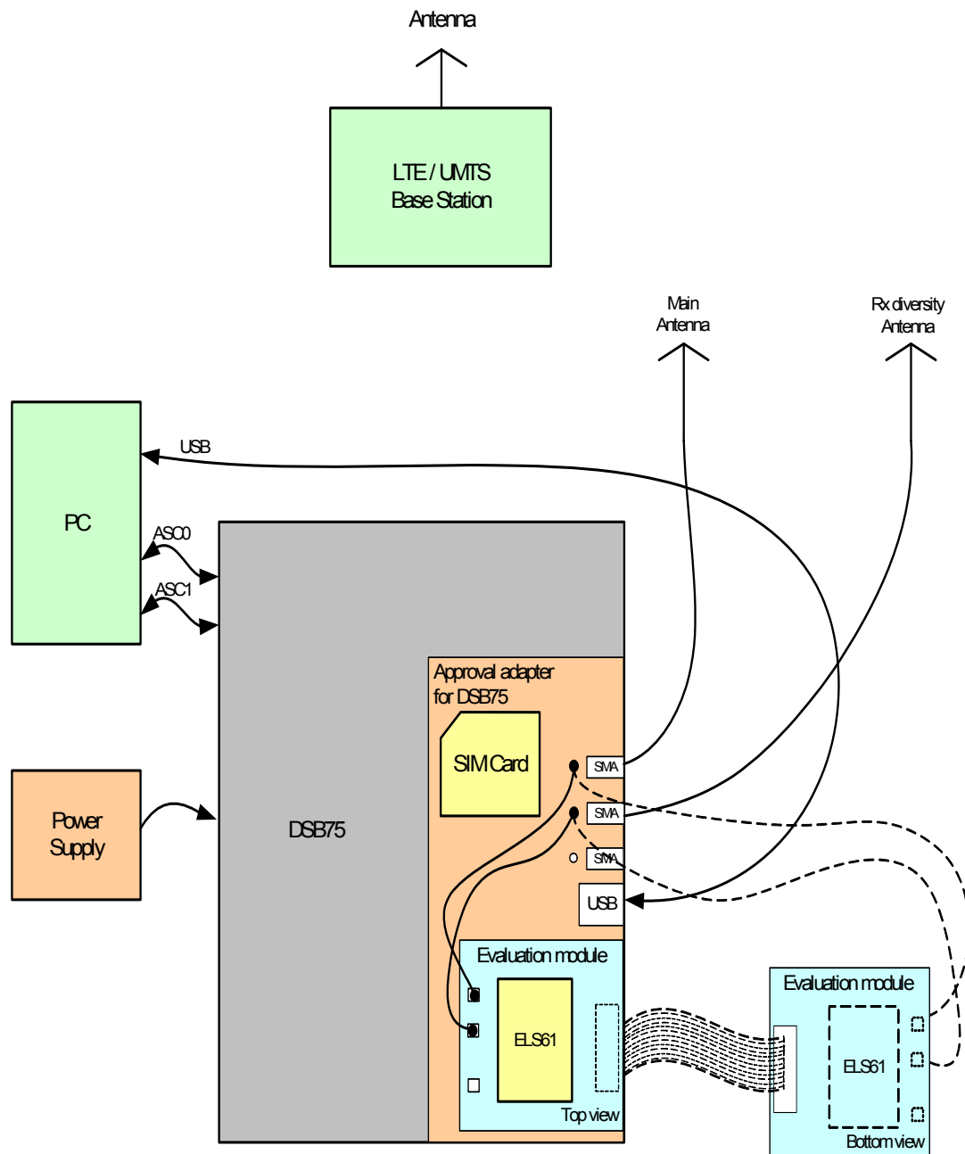
Figure 9: Reference equipment for Type Approval
