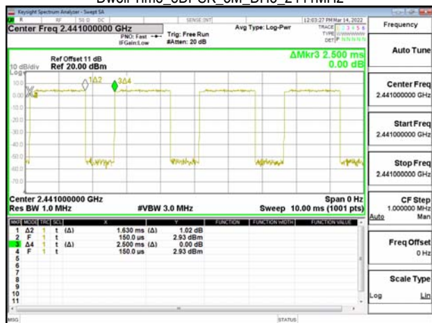
Dwell Time_8DPSK_3M_DH5_2441MHz
