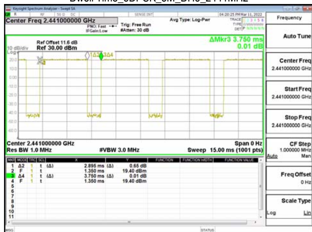
Dwell Time_8DPSK_3M_DH5_2441MHz
