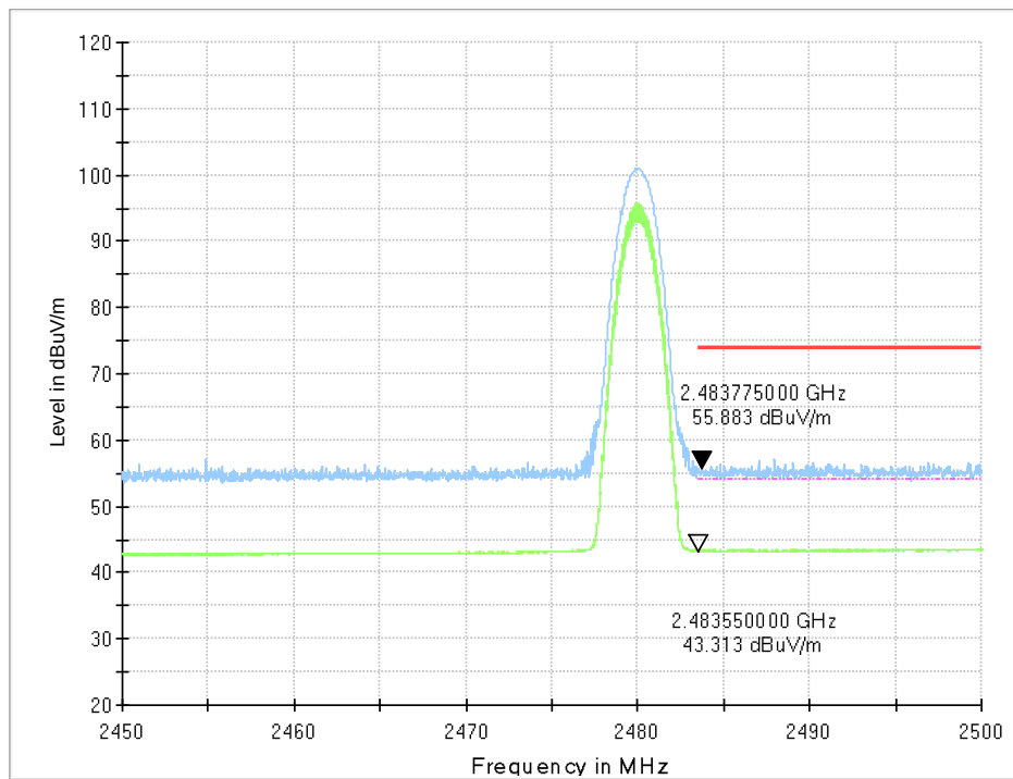
Fig.63. Frequency Band Edges: 8DPSK, Channel 78, 2.45 GHz - 2.50GHz
