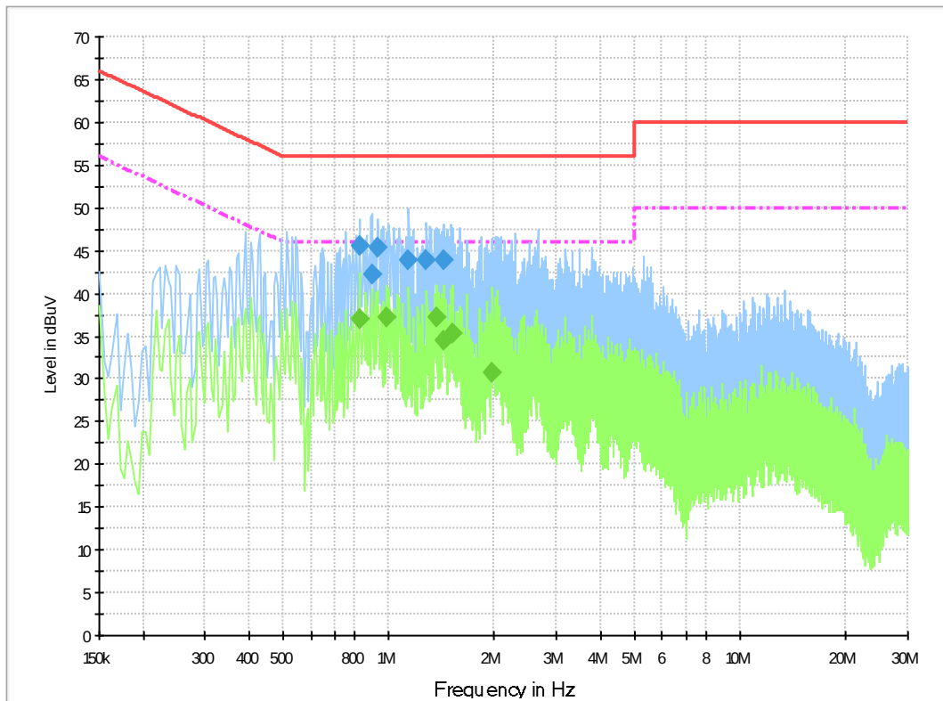
Fig.B.10.2 AC Powerline Conducted Emission-Idle
