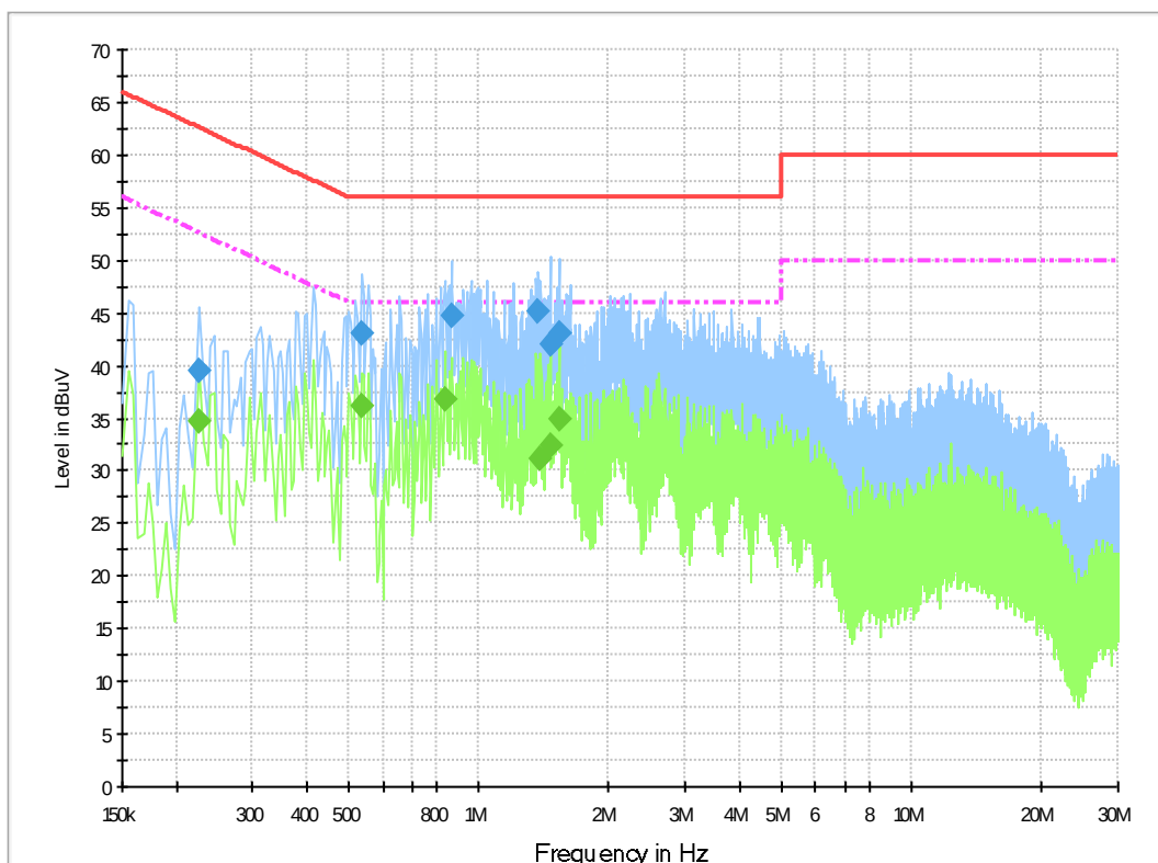
Fig.B.10.1 AC Powerline Conducted Emission- bluetooth
