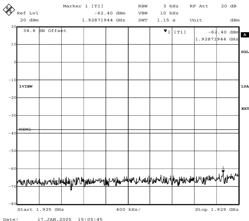
Fig. 27 – Spurious emissions in the frequency range 1925 MHz–1929 MHz (8PSK modulation). Limit: -13dBm–25.2dB–38.2dBm
