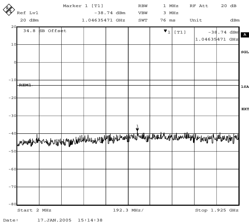
Fig. 39 – Spurious emissions in the frequency range 2 MHz – 1925 MHz (8PSK modulation).
