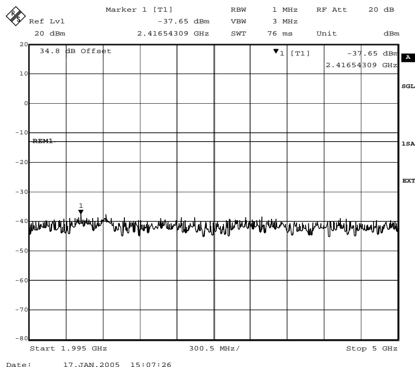
Fig. 35 – Spurious emissions in the frequency range 1995 MHz – 5000 MHz (8PSK modulation).
