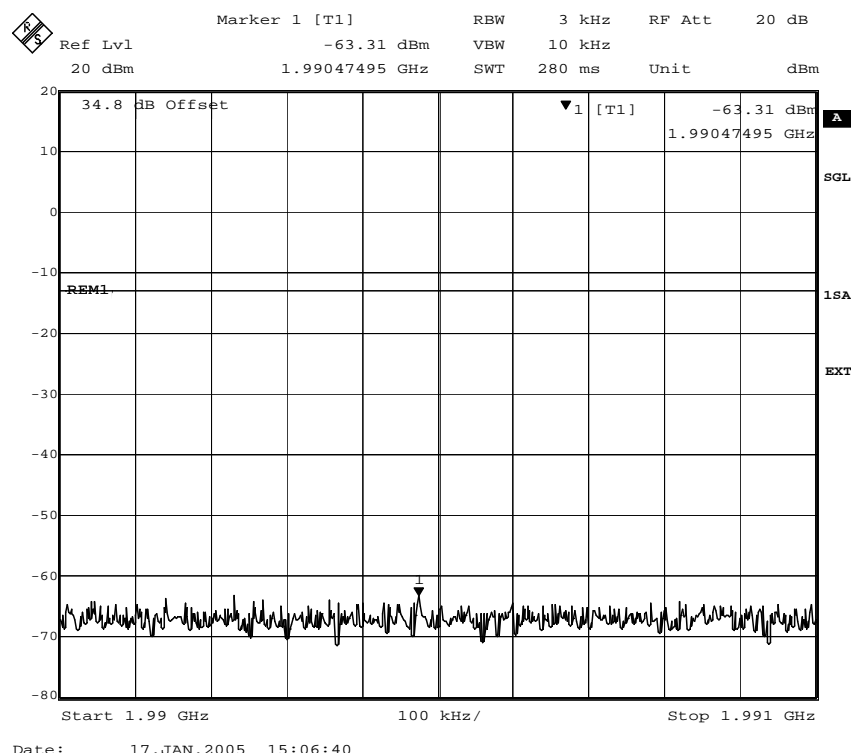
Fig. 31 – Spurious emissions in the frequency range 1990 MHz – 1991 MHz (8PSK modulation).
