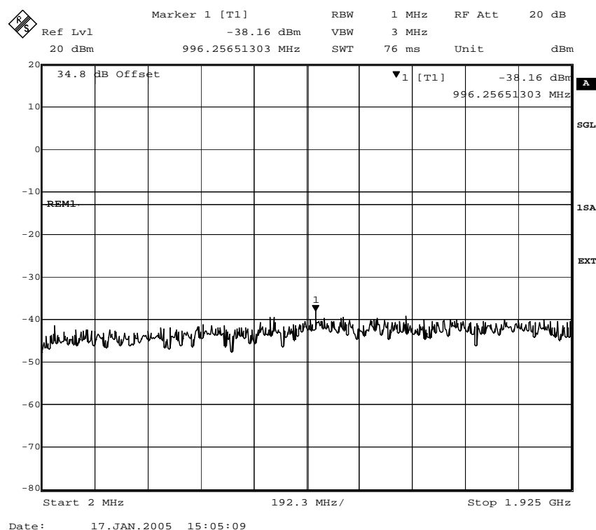
Fig. 25 – Spurious emissions in the frequency range 2 MHz – 1925 MHz (8PSK modulation).
