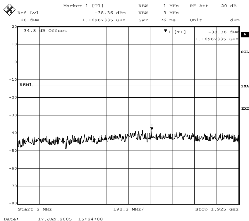
Fig. 53 – Spurious emissions in the frequency range 2 MHz – 1925 MHz (8PSK modulation).
