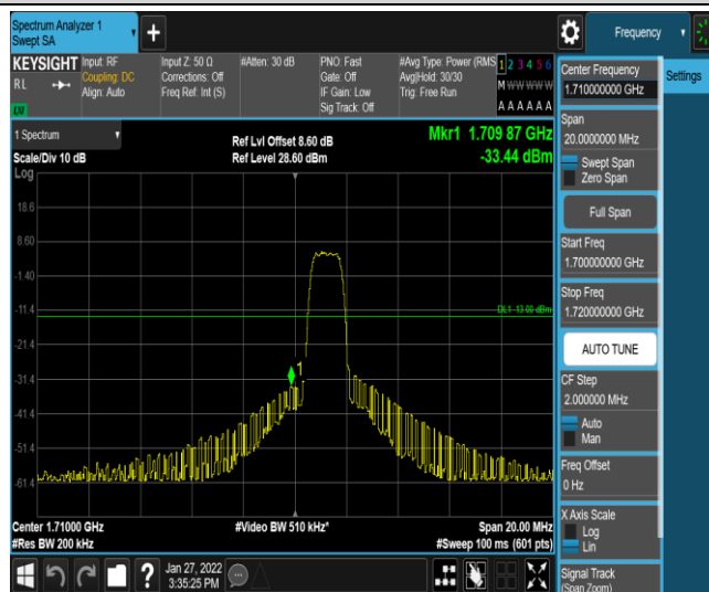
Band4-10MHz-QPSK-20000-6-0-Low--33.44-PASS
