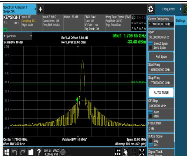
Band4-15MHz-QPSK-20025-1-0-Low--33.48-PASS
