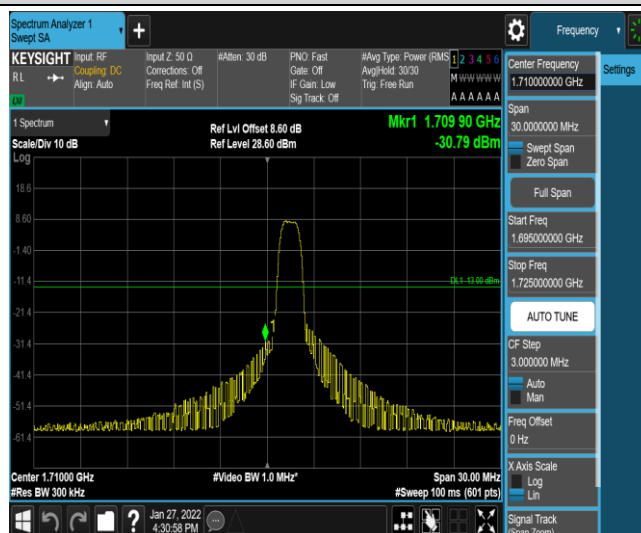
Band4-15MHz-QPSK-20025-6-0-Low--30.79-PASS
