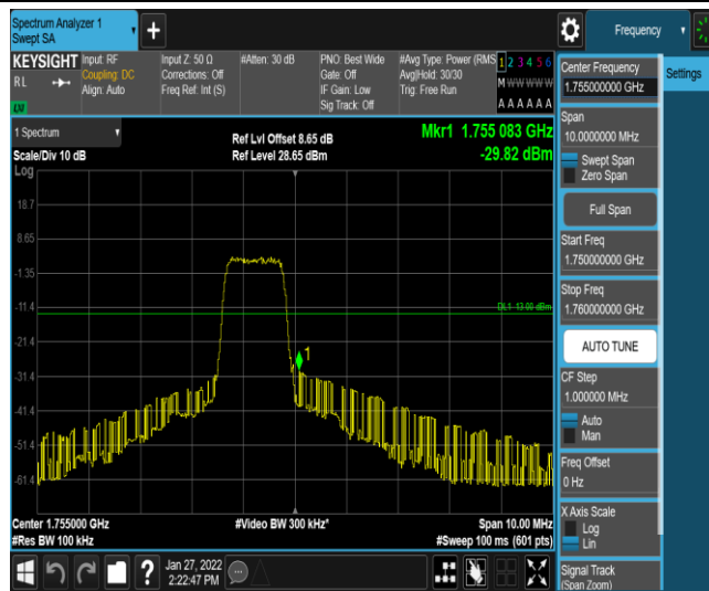
Band4-5MHz-16QAM-20375-6-0-High--29.82-PASS
