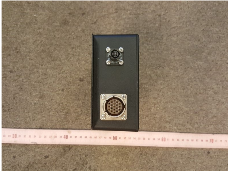
Cable Interface_ Antenna Port Side
