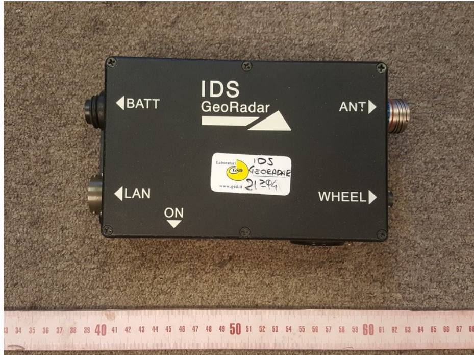
Cable Interface_ Top View
