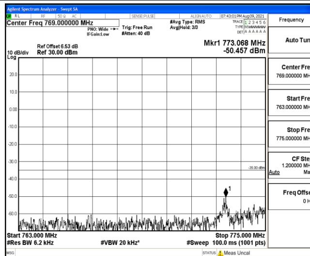
Band13-5MHz-QPSK-23205-1RB#0-Range6:793~805MHz
