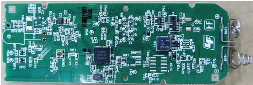
PCB (L2)
