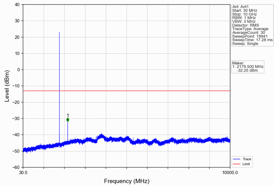
Band66_1.4MHz_16QAM_HCH_1779.3MHz_RB_1_0_NTNV
