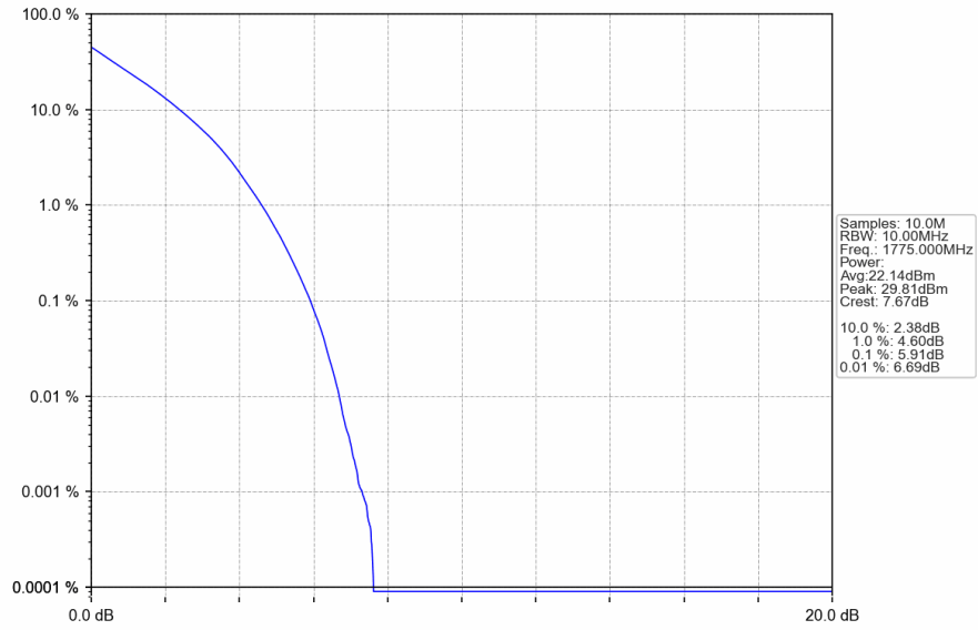
Band66_10MHz_QPSK_HCH_1775MHz_RB_50_0_NTNV
