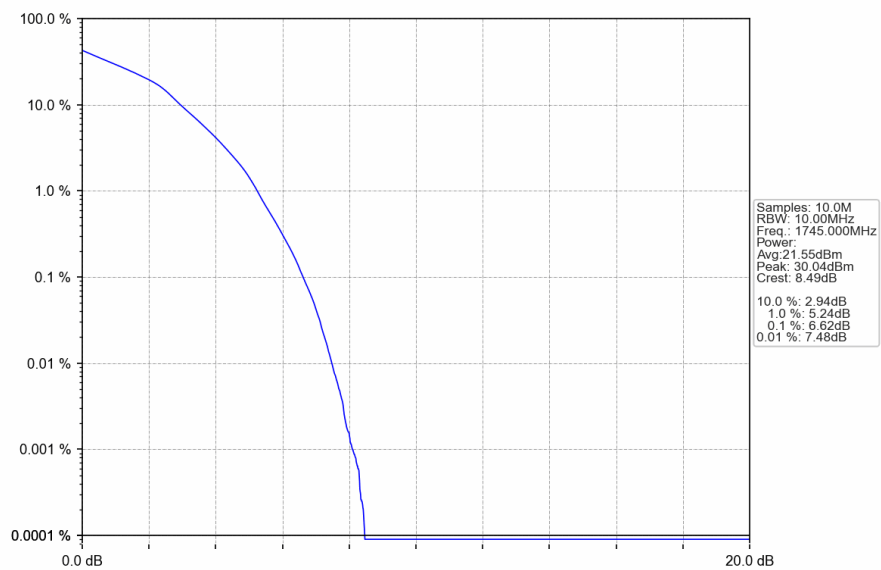
Band66_10MHz_16QAM_MCH_1745MHz_RB_27_0_NTNV
