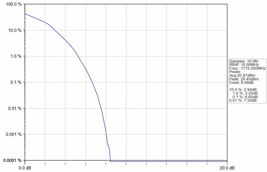
Band66_10MHz_16QAM_LCH_1715MHz_RB_27_0_NTNV
