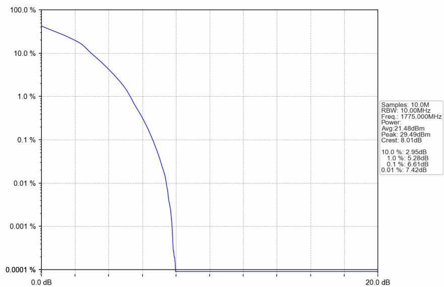
Band66_10MHz_16QAM_HCH_1775MHz_RB_27_23_NTNV
