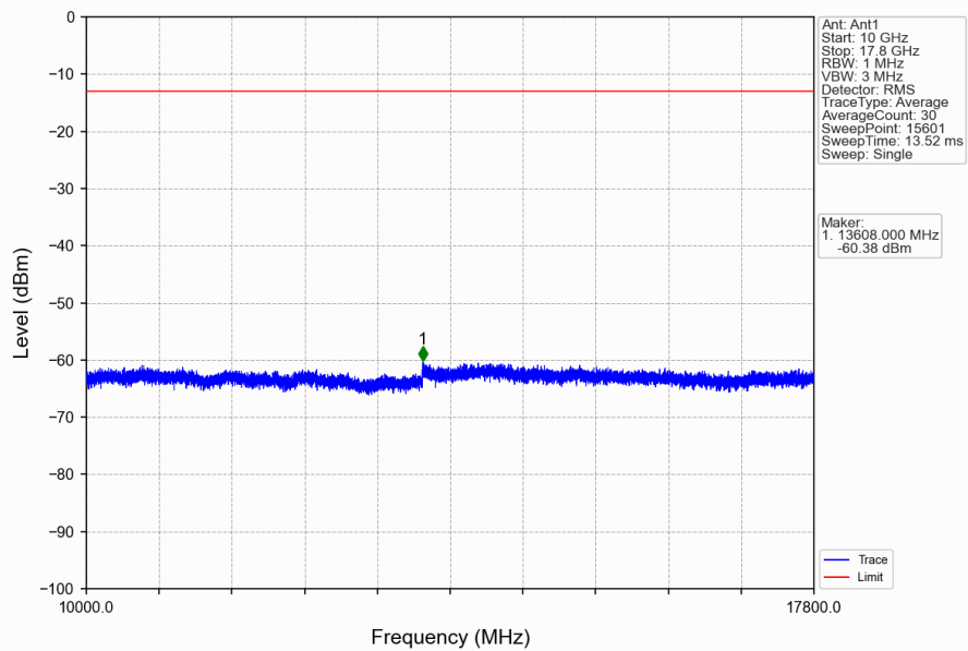
Band66_1.4MHz_16QAM_HCH_1779.3MHz_RB_1_0_NTNV
