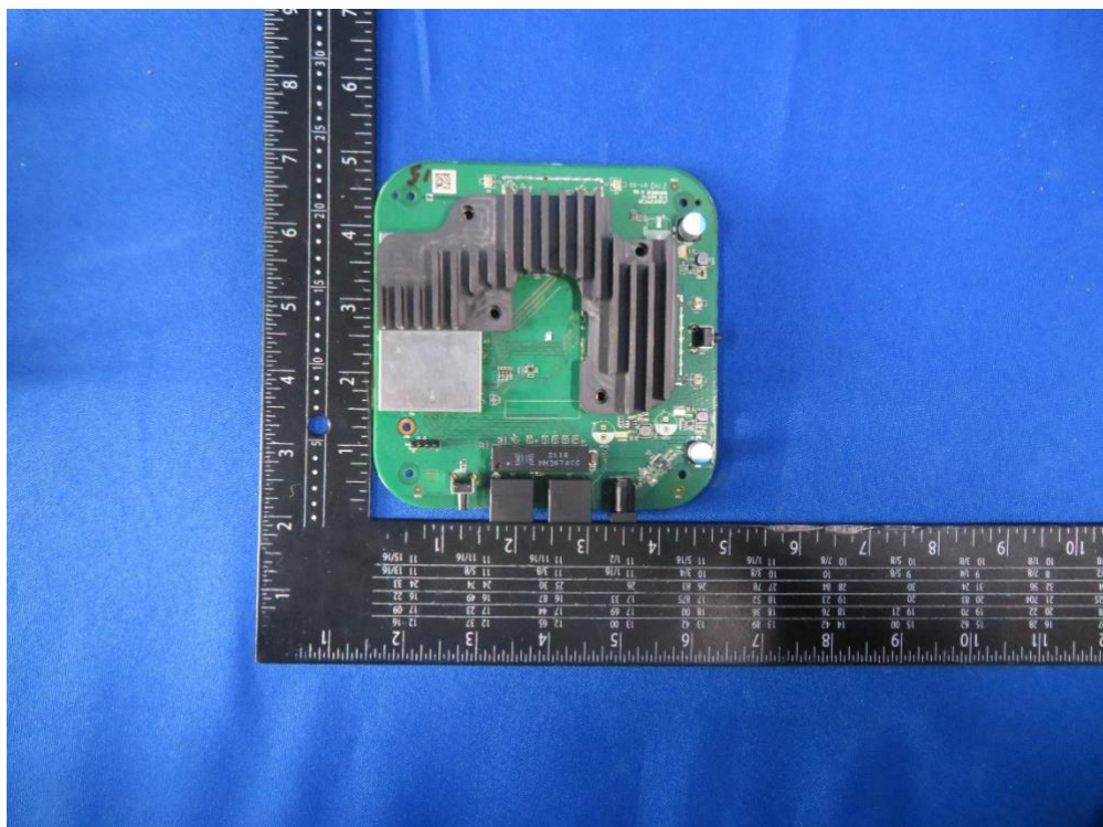
(4) EUT Photo(Type-A Heatsink)
