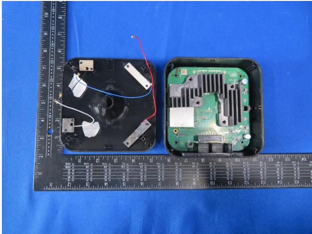
(1) EUT Photo(Type-A Heatsink)
