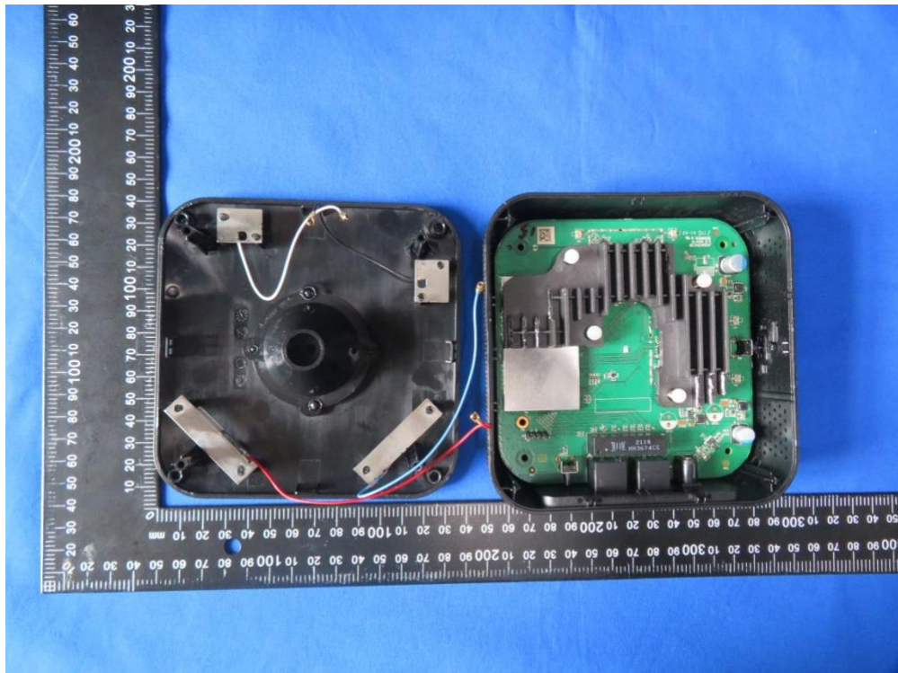
(5) EUT Photo(Type-B Heatsink)
