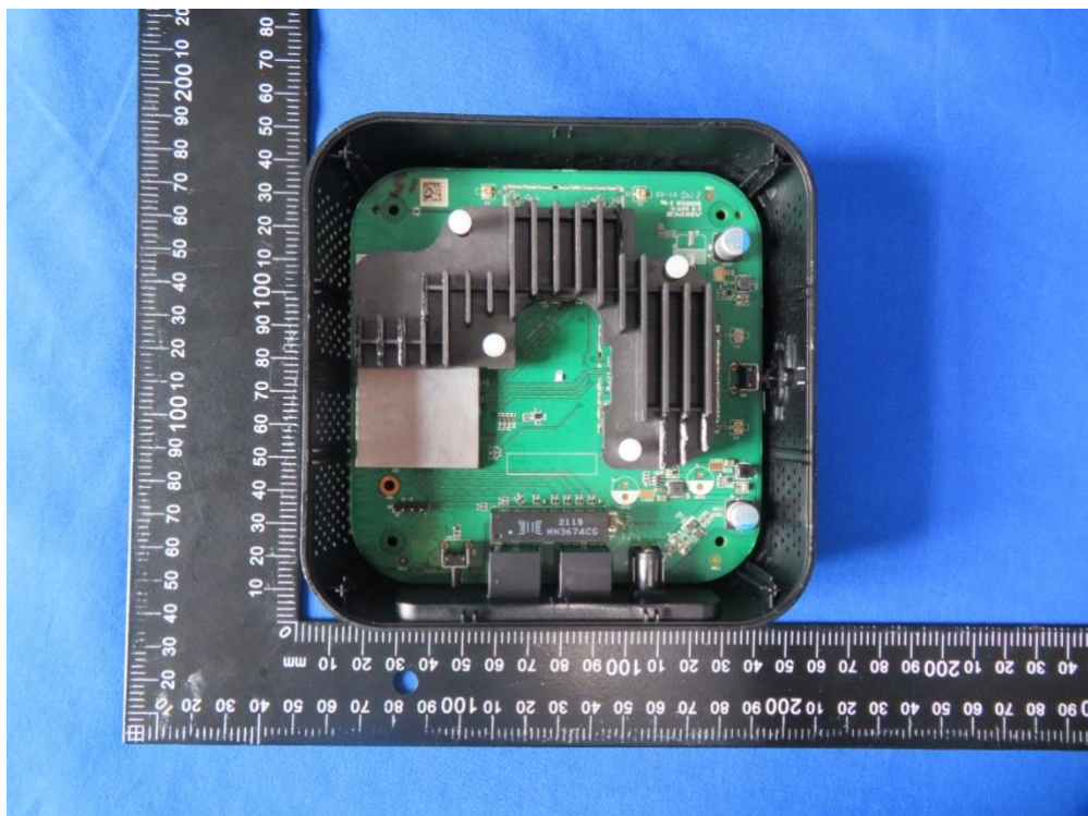
(6) EUT Photo(Type-B Heatsink)
