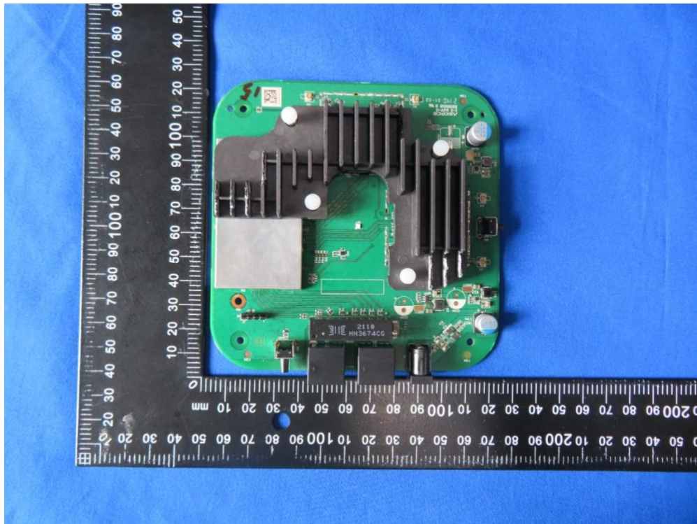
(7) EUT Photo(Type-B Heatsink)
