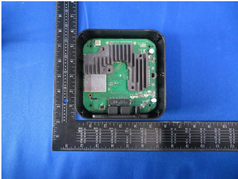
(3) EUT Photo(Type-A Heatsink)
