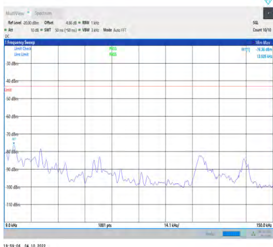
1-N25-PC3-15-40-M-1-DFT-QPSK-Inner_1RB_Left-1 @1-0.009-0.15-Ant1-0.01--76.36--43-PASS
