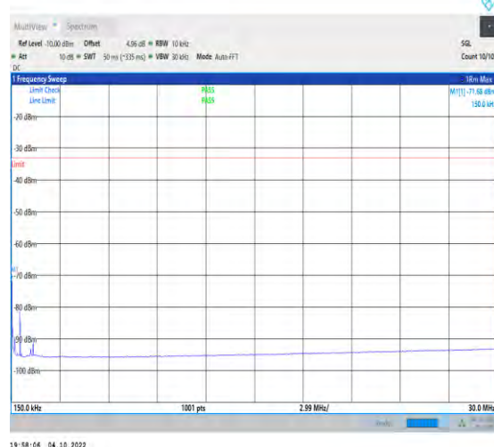
1-N25-PC3-15-40-L-1-DFT-QPSK-Inner_1RB_Left-1 @1-0.15-30-Ant1-0.15--71.68--33-PASS
