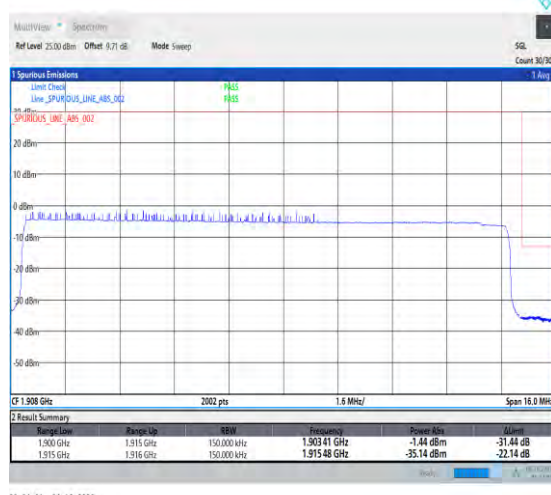
1-N25-PC3-15-15-H-6-CP-QPSK-Outer_Full-79@ 0-Ant1-1-seegraph-PASS-see graph
