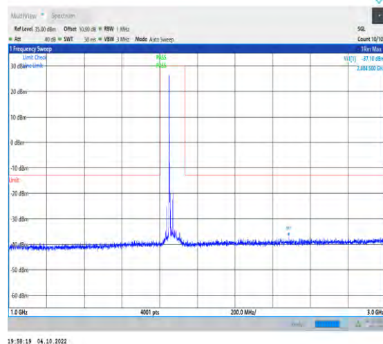
1-N25-PC3-15-40-L-1-DFT-QPSK-Inner_1RB_Left-1 @1-1000-3000-Ant1-2484.50--37.10--13-PASS
