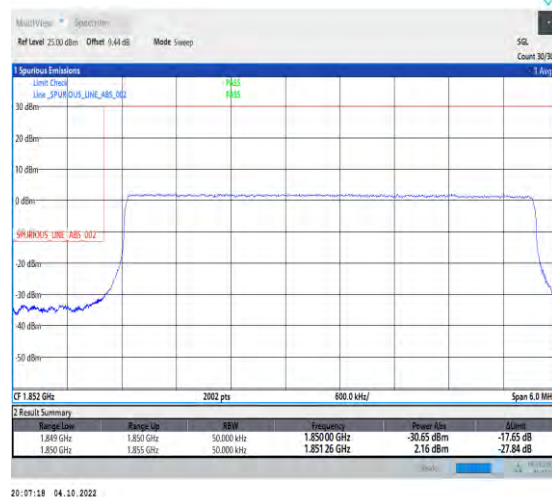
1-N25-PC3-15-5-L-6-CP-QPSK-Outer_Full-25@0- Ant1-1-seegraph-PASS-see graph
