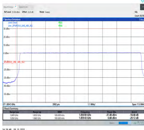
1-N25-PC3-15-10-L-6-CP-QPSK-Outer_Full-52@0-Ant1-1-seegraph-PASS-see graph
