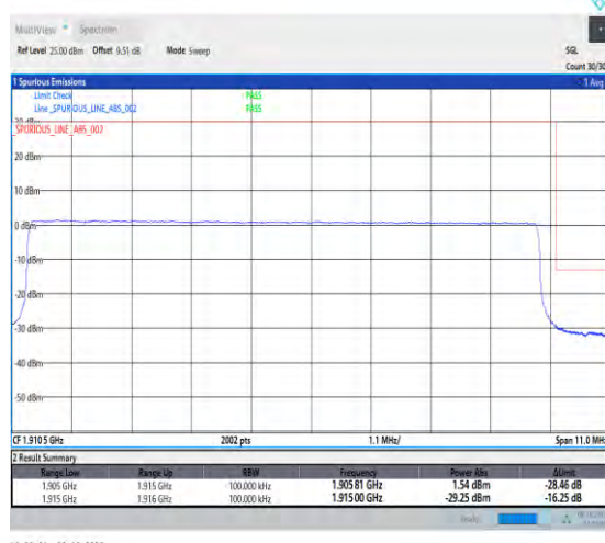
1-N25-PC3-15-10-H-6-CP-QPSK-Outer_Full-52@ 0-Ant1-1-seegraph-PASS-see graph
