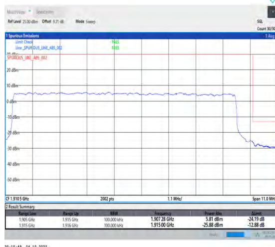
1-N25-PC3-15-10-H-3-DFT-QPSK-Outer_Full-50 @0-Ant1-1-seegraph-PASS-see graph
