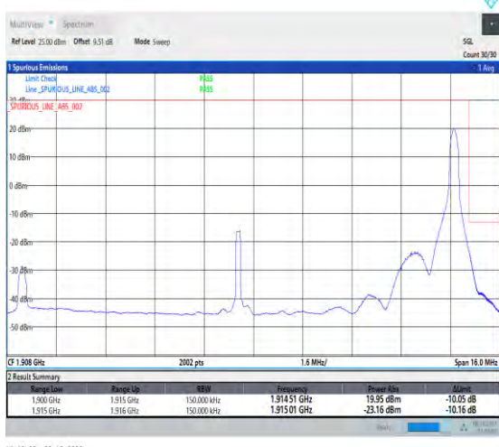
1-N25-PC3-15-15-H-5-CP-QPSK-Edge_1RB_Right-1 @78-Ant1-1-seegraph-PASS-see graph
