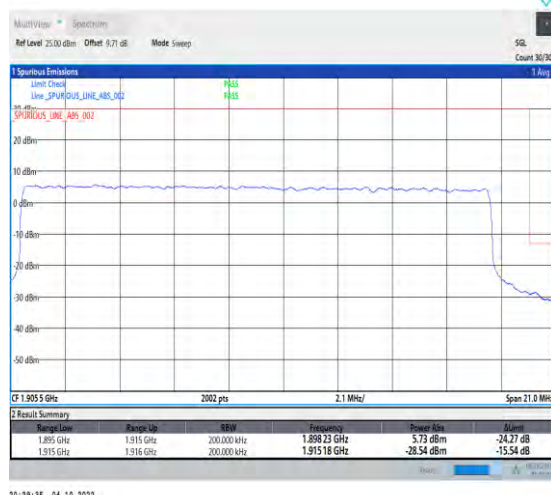
1-N25-PC3-15-20-H-3-DFT-QPSK-Outer_Full-100 @0-Ant1-1-seegraph-PASS-see graph
