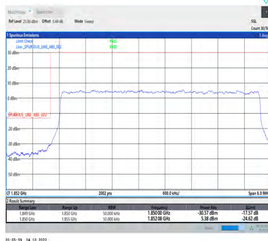
1-N25-PC3-15-5-L-3-DFT-QPSK-Outer_Full-25@0 -Ant1-1-seegraph-PASS-see graph
