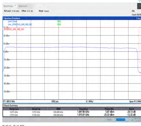
1-N25-PC3-15-40-H-3-DFT-QPSK-Outer_Full-216 @0-Ant1-1-seegraph-PASS-see graph
