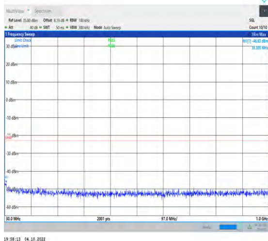
1-N25-PC3-15-40-L-1-DFT-QPSK-Inner_1RB_Left-1 @1-30-1000-Ant1-35.34--46.83--23-PASS
