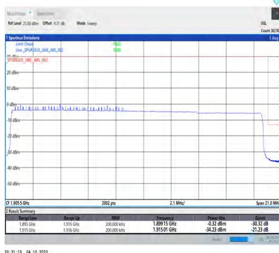
1-N25-PC3-15-20-H-6-CP-QPSK-Outer_Full-106 @0-Ant1-1-seegraph-PASS-see graph
