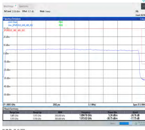
1-N25-PC3-15-30-H-3-DFT-QPSK-Outer_Full-160 @0-Ant1-1-seegraph-PASS-see graph
