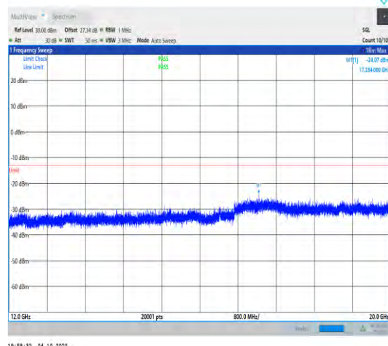
1-N25-PC3-15-40-L-1-DFT-QPSK-Inner_1RB_Left-1 @1-12000-20000-Ant1-17234.00--24.07--13-PASS
