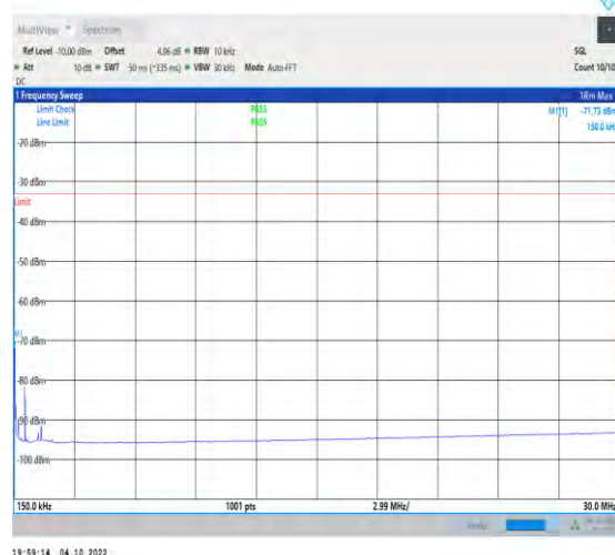
1-N25-PC3-15-40-M-1-DFT-QPSK-Inner_1RB_Left-1 @1-0.15-30-Ant1-0.15--71.73--33-PASS
