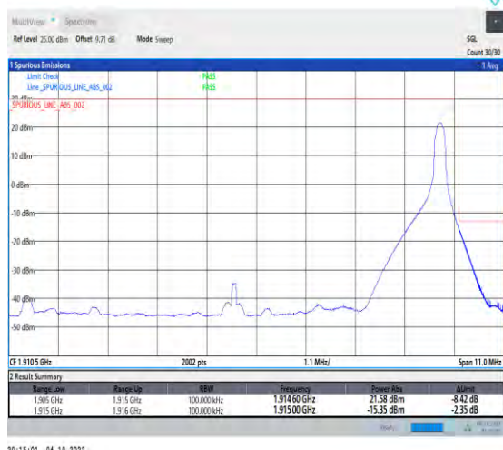
1-N25-PC3-15-10-H-2-DFT-QPSK-Edge_1RB_Right-1 @51-Ant1-1-seegraph-PASS-see graph
