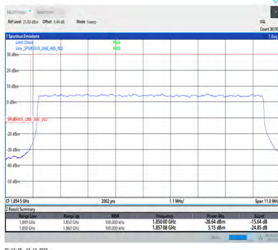
1-N25-PC3-15-10-L-3-DFT-QPSK-Outer_Full-50@0-Ant1-1-seegraph-PASS-see graph
