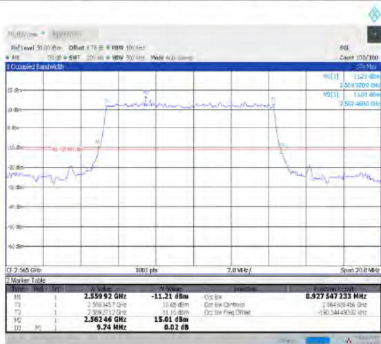
1-N7--15-10-M-9-CP-256QAM-Outer_Full-52@0- Ant1-9.309-10.200-≤10-PASS
