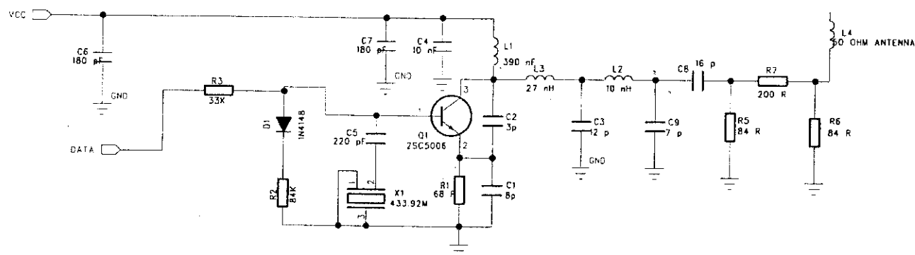
UHF TRANSMITTER
