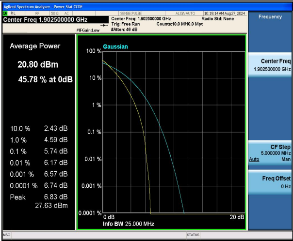
Band2-15MHz-QPSK-19125-75RB#0-PASS
