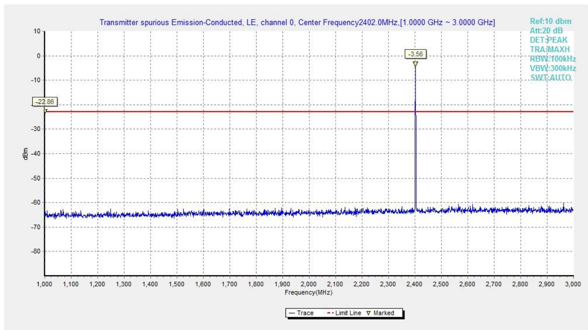
Fig.9 Conducted Spurious Emission (Ch0, 1GHz-3GHz), LE 1M
