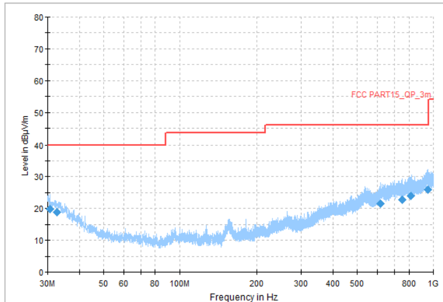
Fig.19 Radiated Spurious Emission (Ch19, 30MHz - 1GHz), 1M
