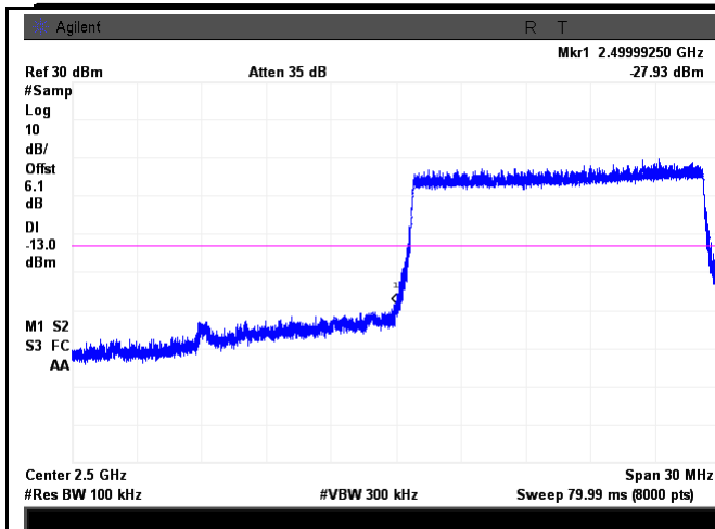
LTE Band 7 - Low Channel QPSK-15
