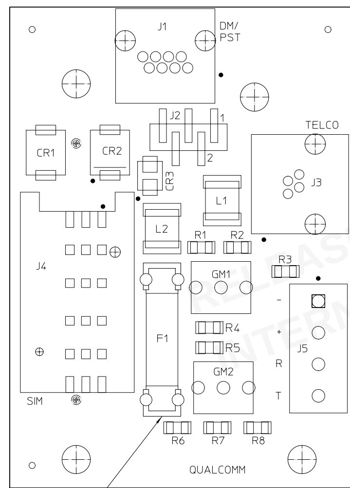
-2 SIDE A
