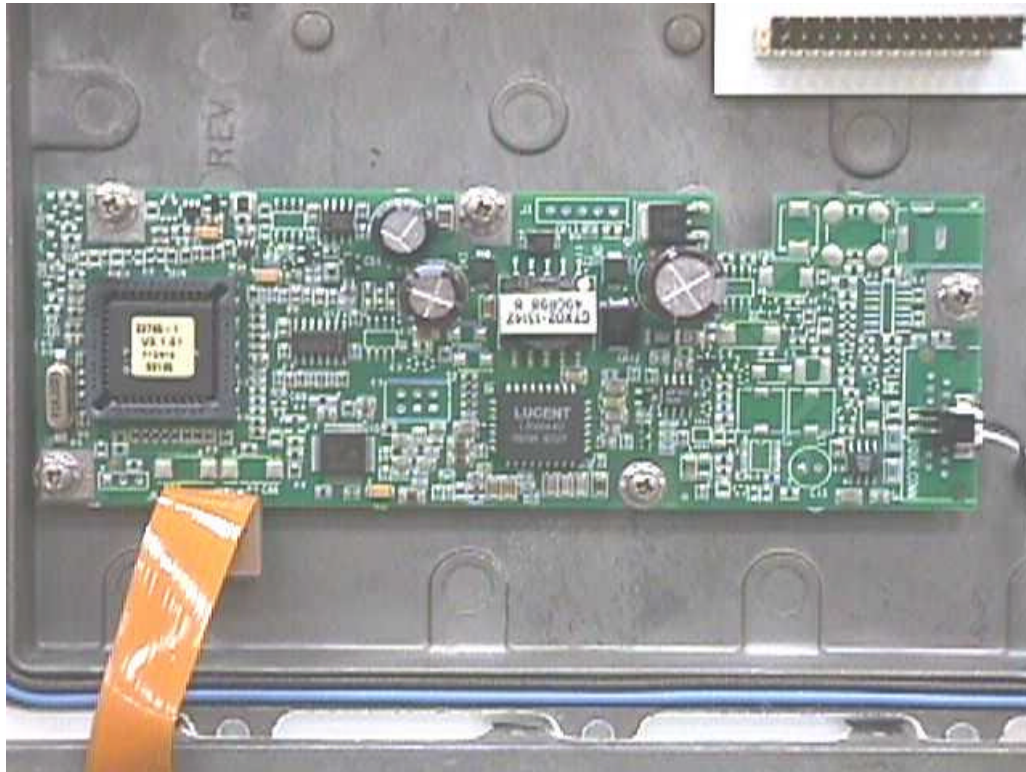
REN Board
