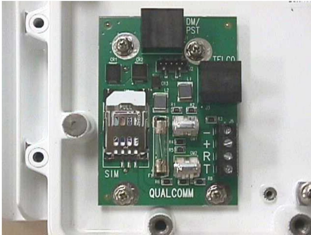
Interface Board
