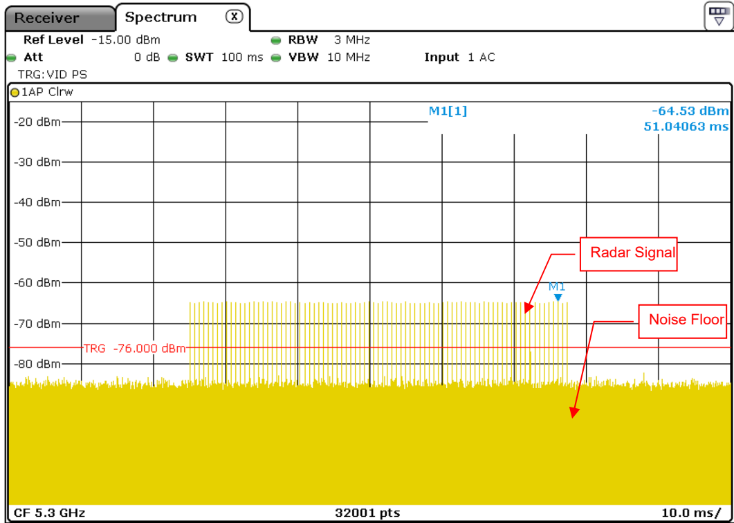
Radar Signal 1 (Test A)
