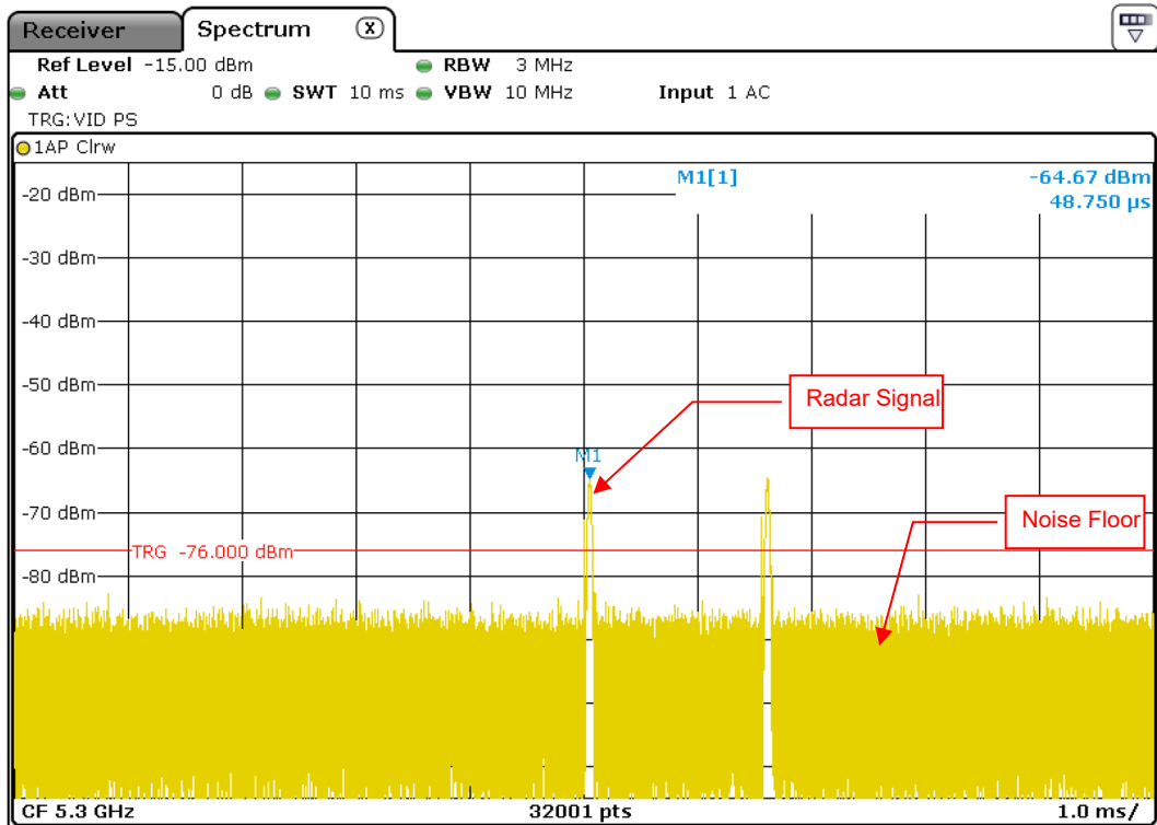
Single Burst of Radar Signal 5
