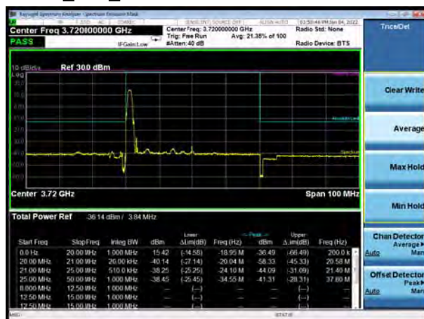
DC_66A_n78 40MHz QPSK 1RB CH-Low
