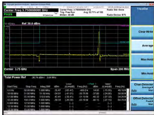
DC_66A_n78 100MHz 64QAM 100%RB CH-High
