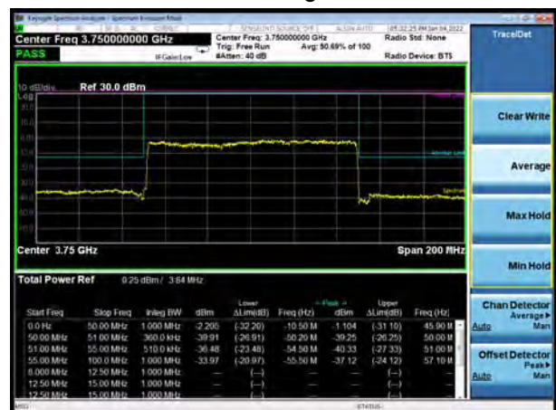
DC_66A_n78 100MHz 16QAM 100%RB CH-High
