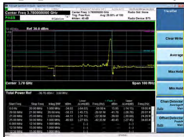
DC_66A_n78 40MHz PI/2 BPSK 100%RB CH-High
