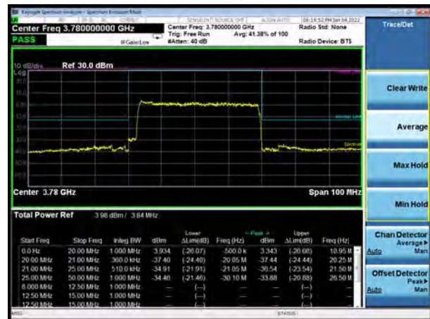
DC_66A_n78 40MHz QPSK 1RB CH-High
