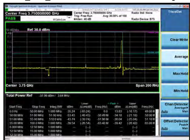
DC_66A_n78 100MHz QPSK 1RB CH-High
