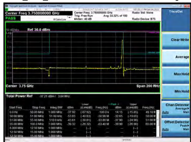
DC_66A_n78 100MHz 16QAM 100%RB CH-High
