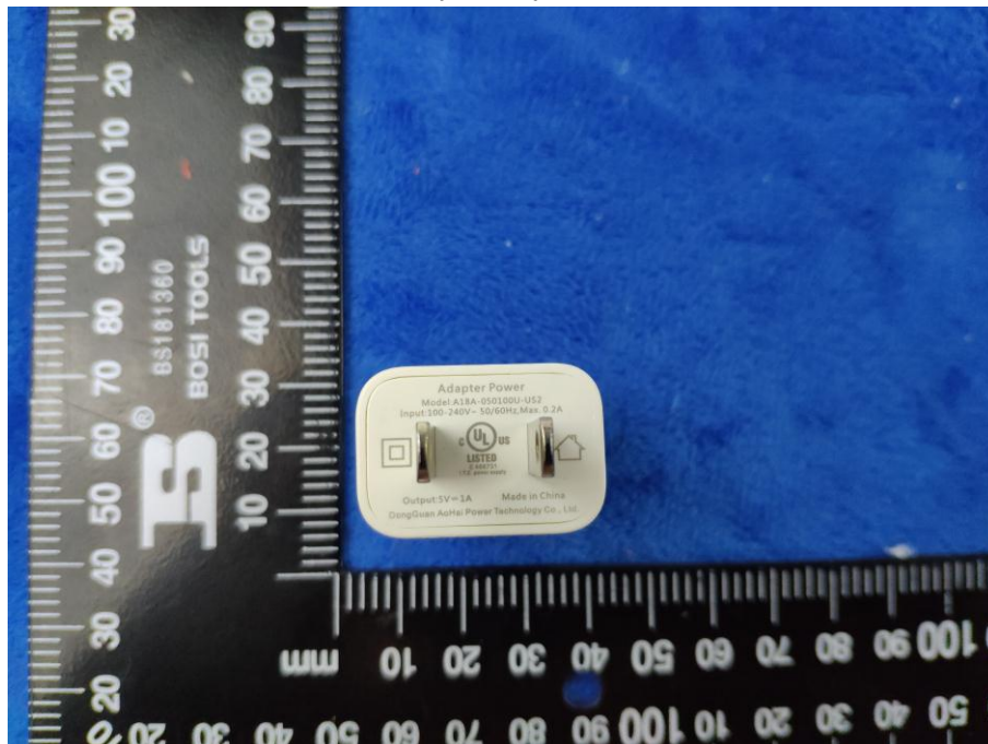
Adapter-Top View
