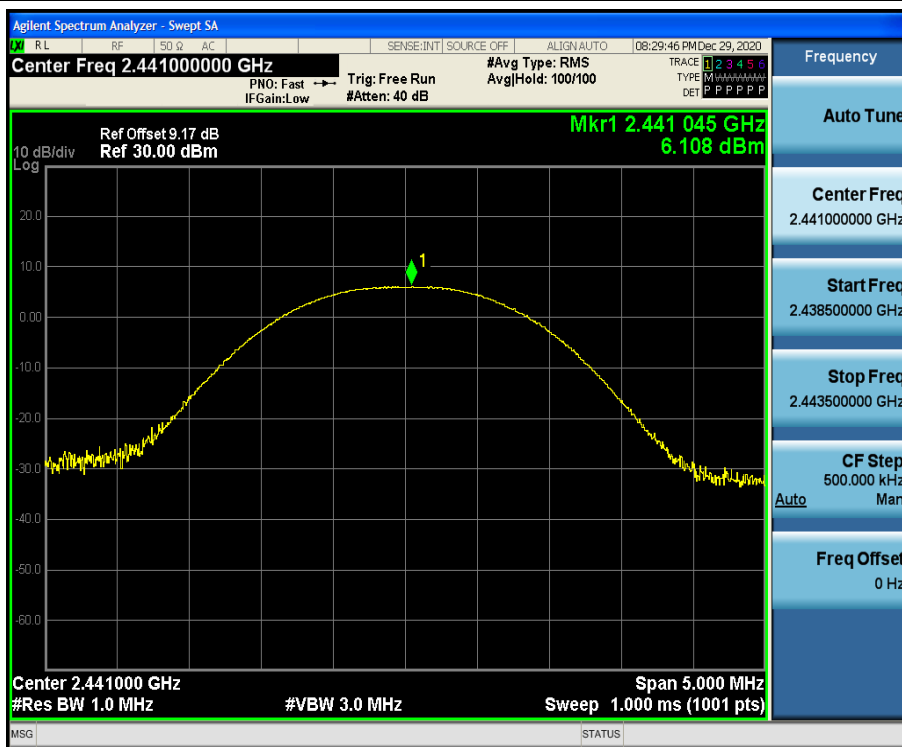
GFSK mode-CH39
