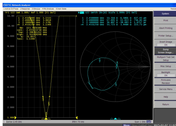
Fig.1 驻波比 VSWR
