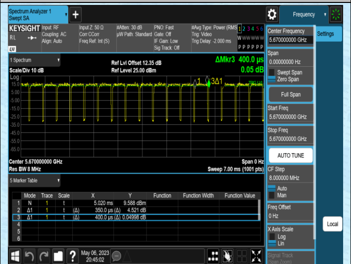
NTNV-11AC40MIMO-Ant2-5670
