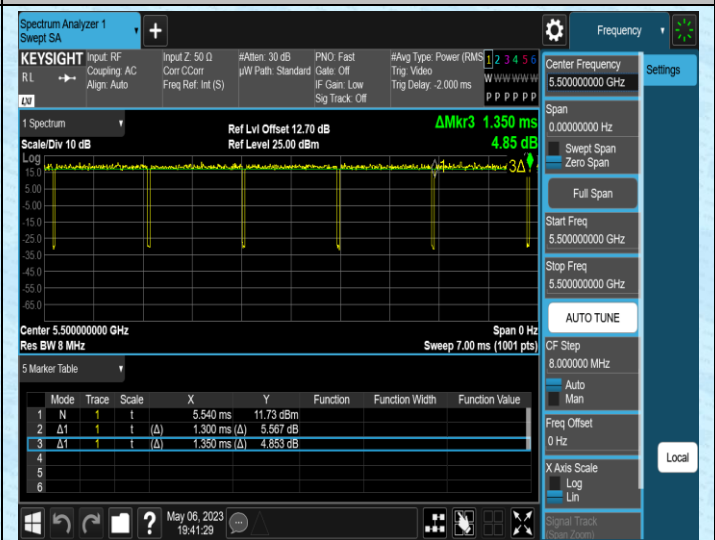
NTNV-11N20MIMO-Ant2-5500
