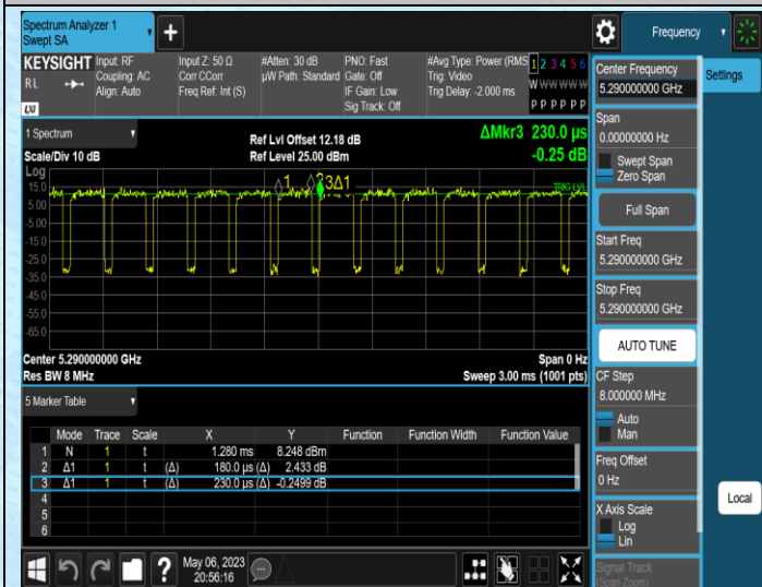
NTNV-11AC80MIMO-Ant1-5290
