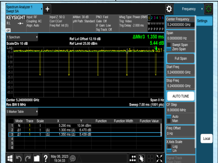
NTNV-11N20MIMO-Ant2-5240
