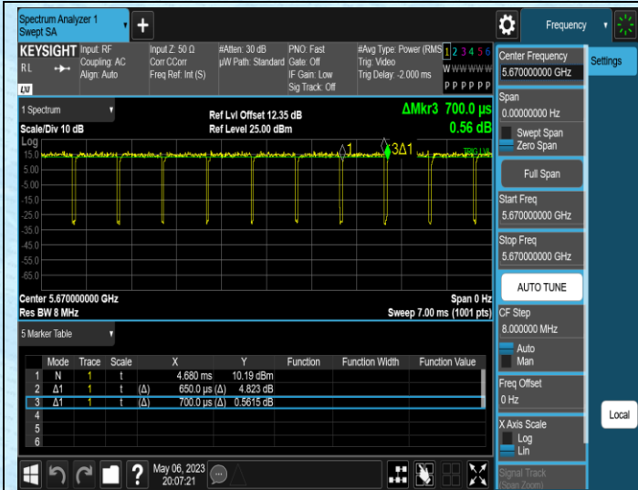
NTNV-11N40MIMO-Ant1-5670
