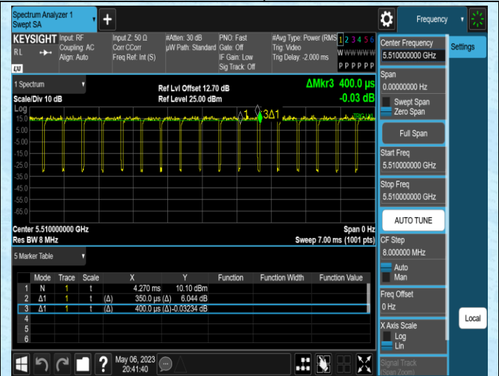
NTNV-11AC40MIMO-Ant2-5510
