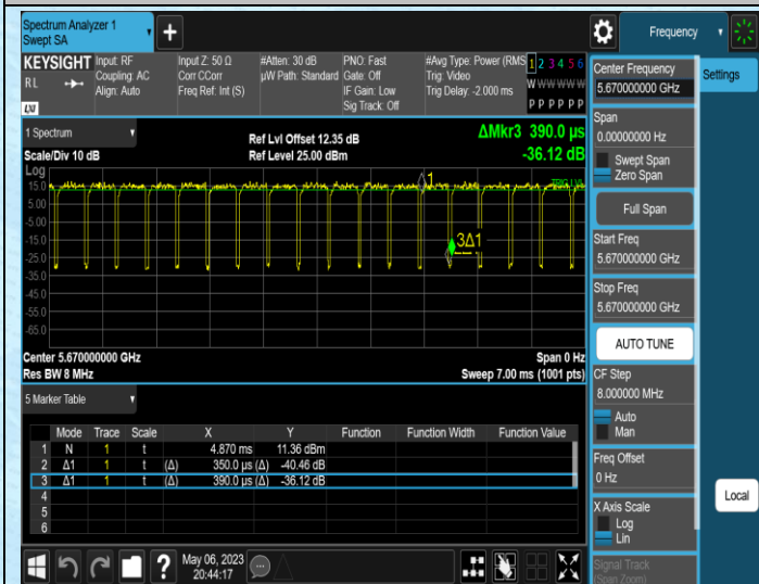
NTNV-11AC40MIMO-Ant1-5670
