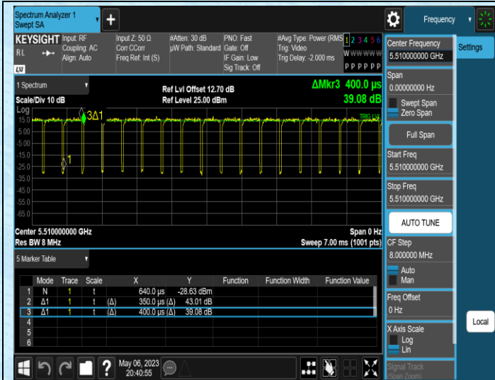
NTNV-11AC40MIMO-Ant1-5510
