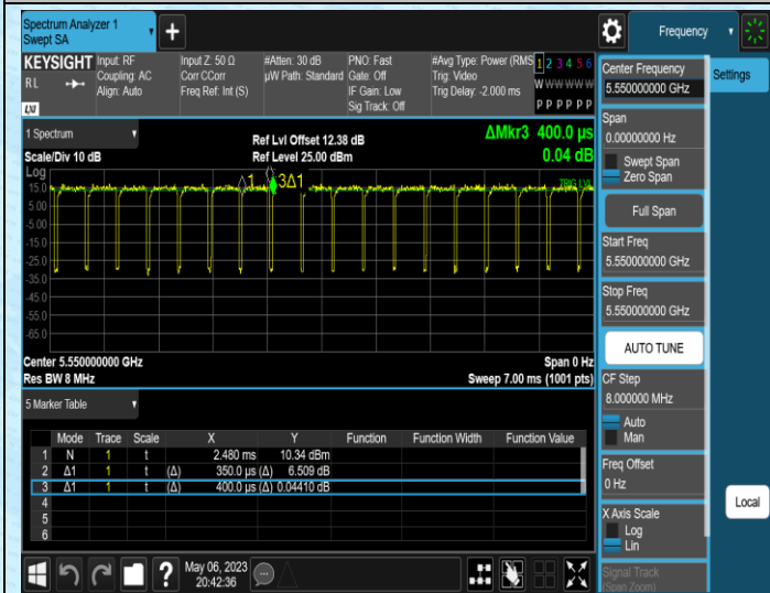
NTNV-11AC40MIMO-Ant1-5550
