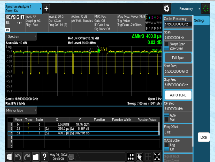
NTNV-11AC40MIMO-Ant2-5550
