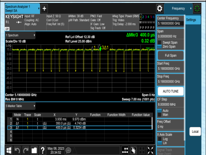
NTNV-11AC40MIMO-Ant2-5190
