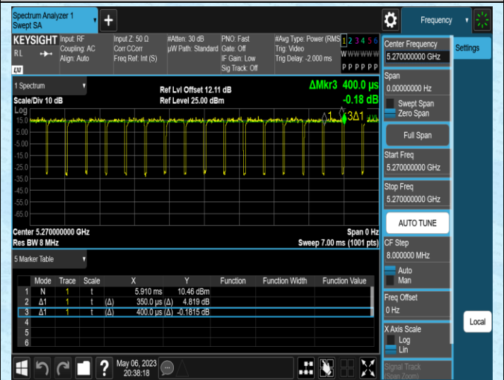
NTNV-11AC40MIMO-Ant2-5270
