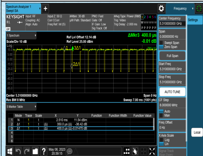
NTNV-11AC40MIMO-Ant1-5310
