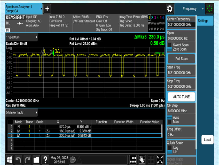
NTNV-11AC80MIMO-Ant2-5210
