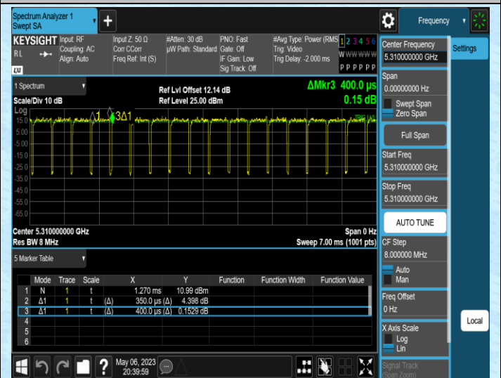
NTNV-11AC40MIMO-Ant2-5310
