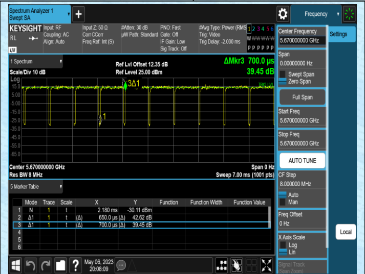
NTNV-11N40MIMO-Ant2-5670
