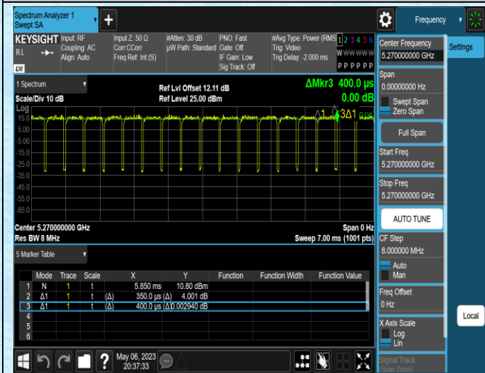
NTNV-11AC40MIMO-Ant1-5270
