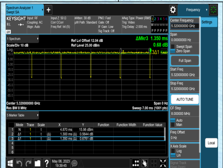
NTNV-11N20MIMO-Ant2-5320
