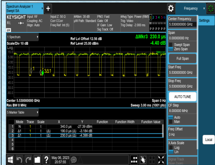
NTNV-11AC80MIMO-Ant1-5530
