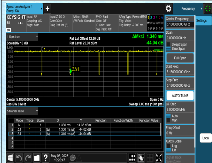
NTNV-11N20MIMO-Ant1-5180
