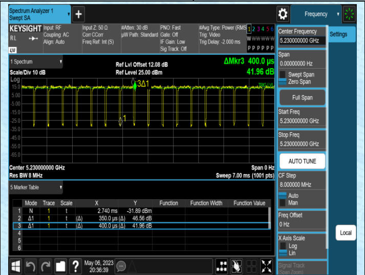
NTNV-11AC40MIMO-Ant2-5230
