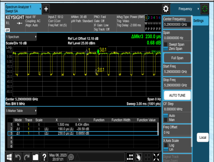
NTNV-11AC80MIMO-Ant2-5290
