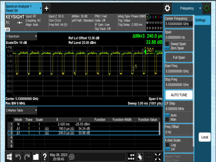
NTNV-11AC80MIMO-Ant2-5530
