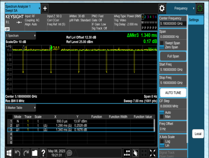
NTNV-11N20MIMO-Ant2-5180
