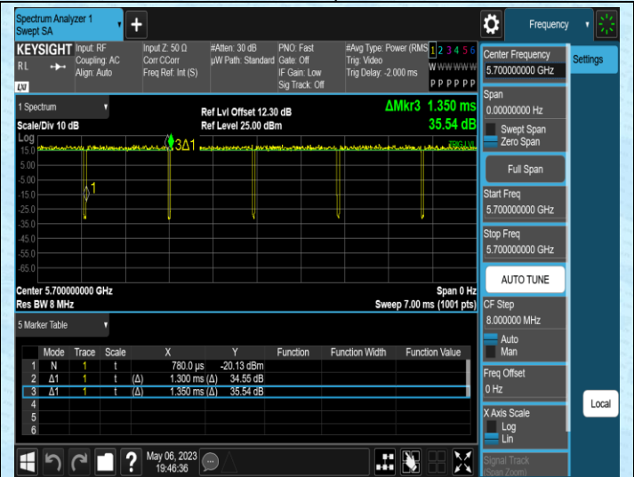
NTNV-11N20MIMO-Ant2-5700
