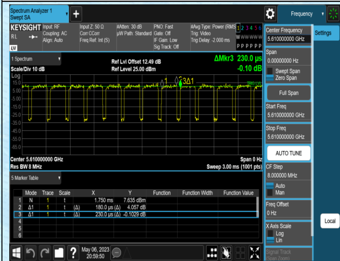
NTNV-11AC80MIMO-Ant1-5610
