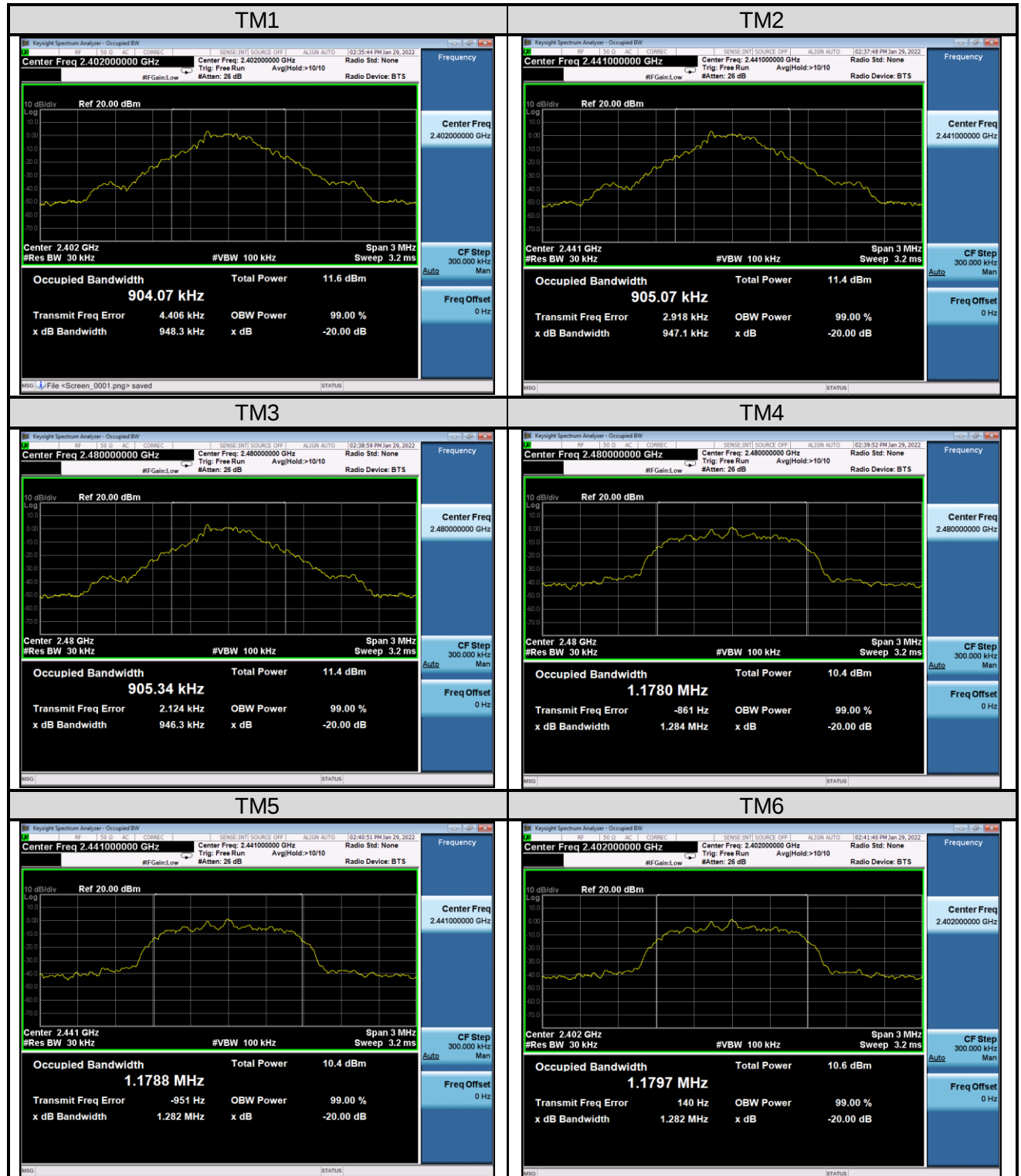
Figure 1: 20dB & 99% Bandwidth
