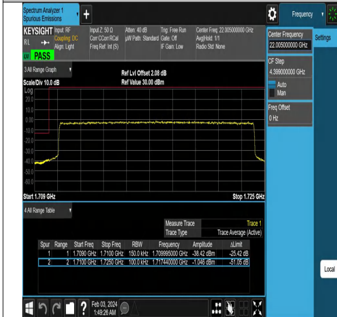
Band4_15MHz_QPSK_20025_75RB#0
