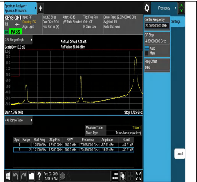
Band4_15MHz_QPSK_20025_1RB#74
