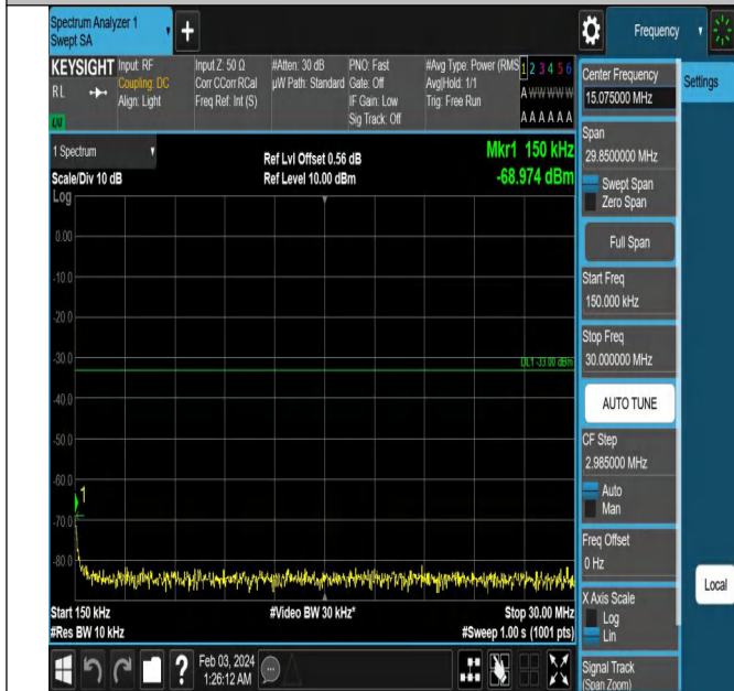
Band4_1.4MHz_QPSK_20175_1RB#0_0.15~30_0.15~30
