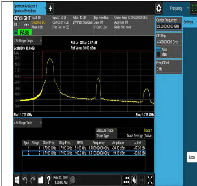
Band4_5MHz_QPSK_19975_1RB#0
