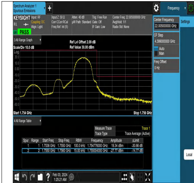
Band4_1.4MHz_QPSK_20393_1RB#5
