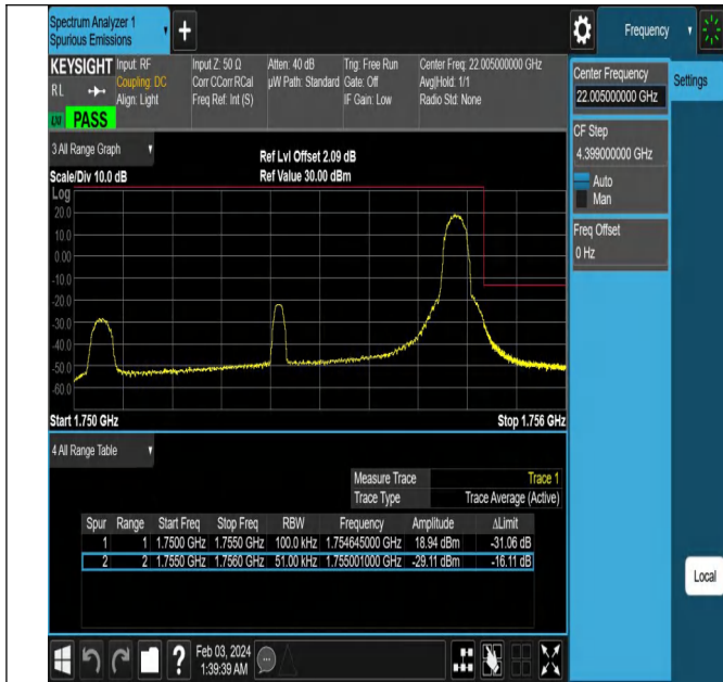
Band4_5MHz_QPSK_20375_1RB#24
