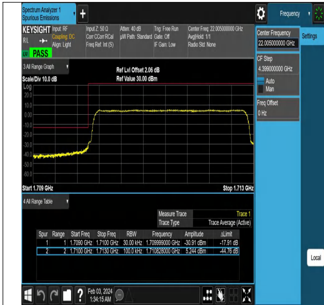
Band4_3MHz_QPSK_19965_15RB#0
