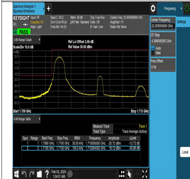
Band4_3MHz_QPSK_19965_1RB#0
