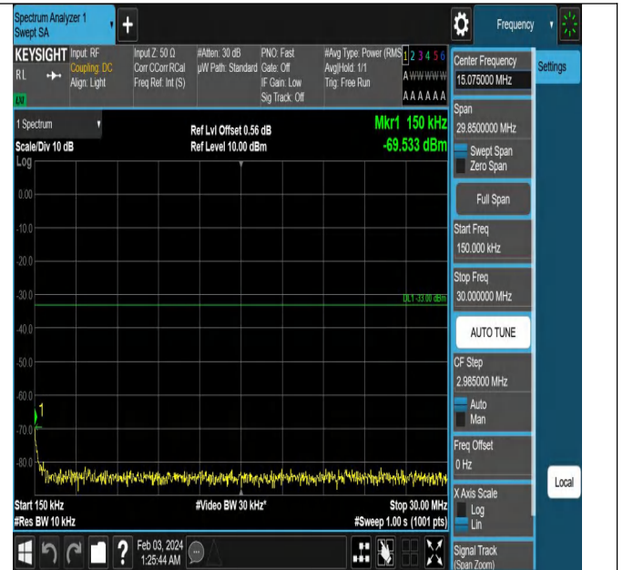
Band4_1.4MHz_QPSK_19957_1RB#0_0.15~30_0.15~30
