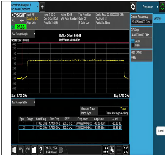
Band4_20MHz_QPSK_20050_100RB#0
