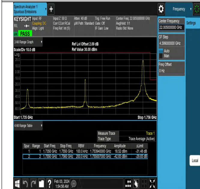
Band4_20MHz_QPSK_20300_1RB#99
