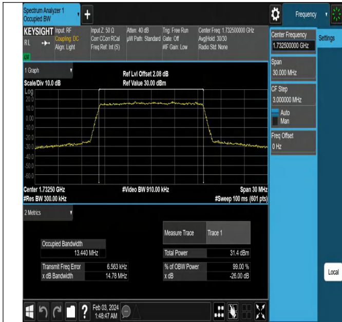
Band4-15MHz-QPSK-20175-75RB#0-PASS
