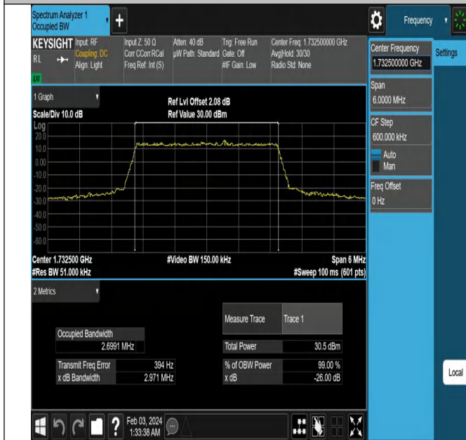
Band4-3MHz-QPSK-20175-15RB#0-PASS
