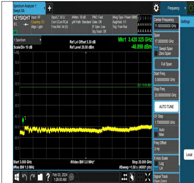
Band4_1.4MHz_QPSK_19957_1RB#0_3000~20000_3000~20000
