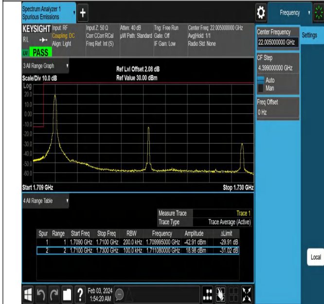
Band4_20MHz_QPSK_20050_1RB#0
