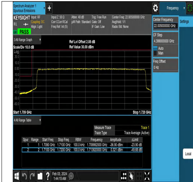
Band4_10MHz_QPSK_20000_50RB#0
