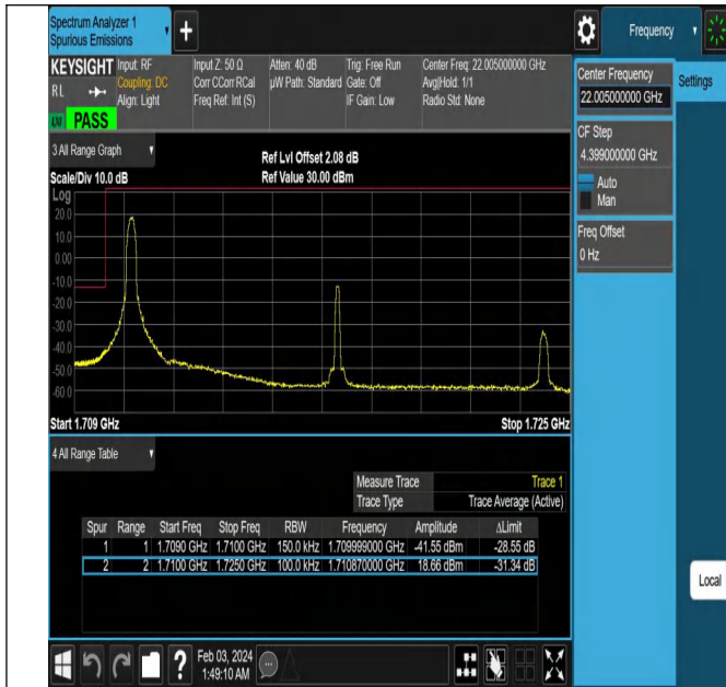
Band4_15MHz_QPSK_20025_1RB#0
