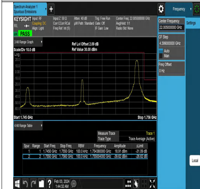
Band4_10MHz_QPSK_20350_1RB#49
