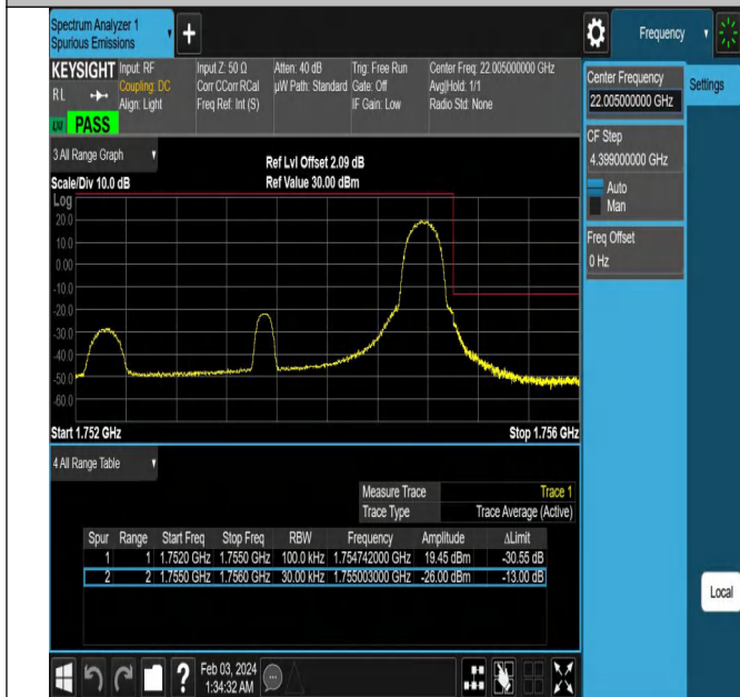
Band4_3MHz_QPSK_20385_1RB#14
