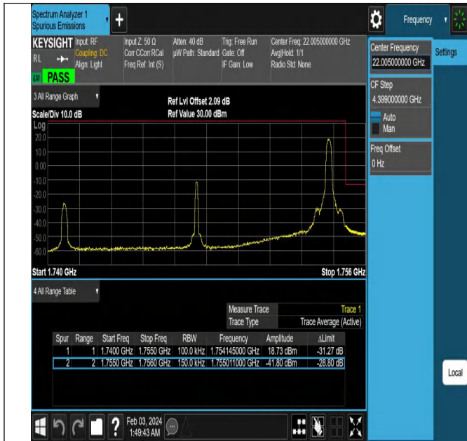
Band4_15MHz_QPSK_20325_1RB#74
