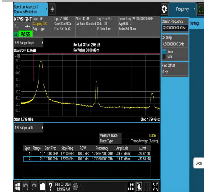
Band4_10MHz_QPSK_20000_1RB#0
