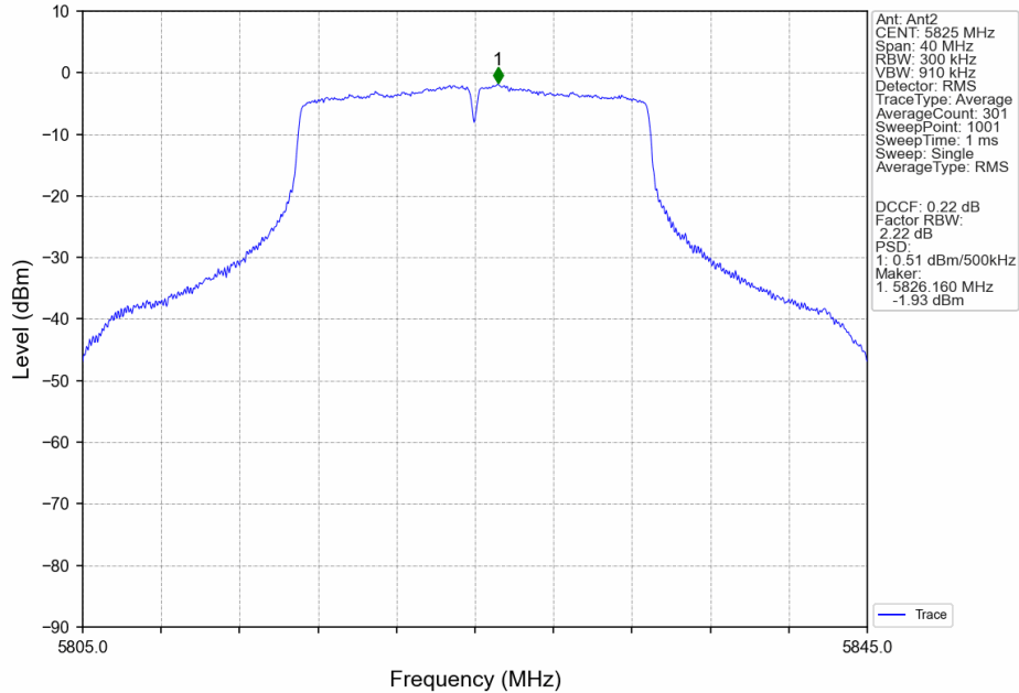
802.11ac(VHT20)_HCH_5825MHz_MIMO_NTNV
