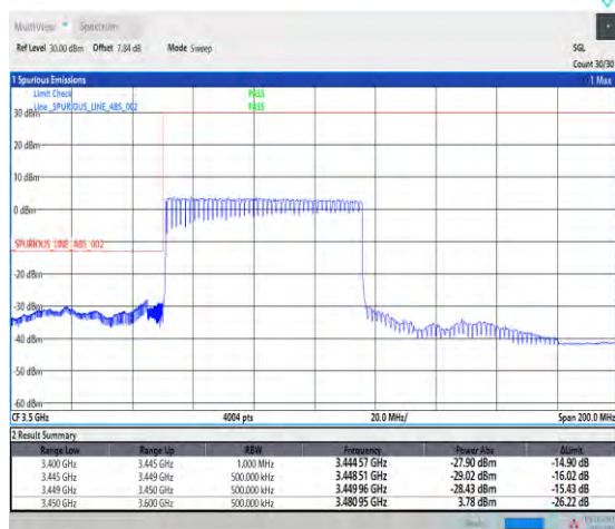
1-N78-3450-3550--30-70-L-3-DFT-PI2BPSK-Outer _Full-180@0-Ant1-1--PASS-see graph
