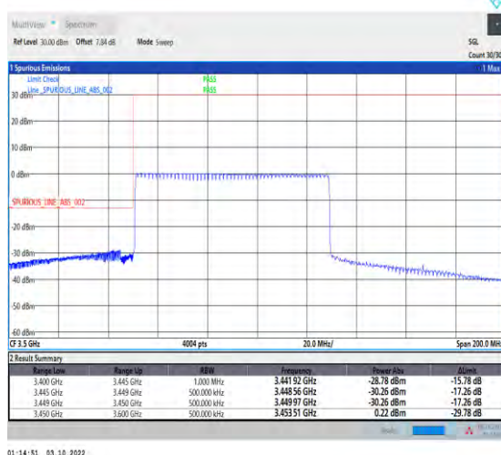
1-N78-3450-3550--30-80-L-6-CP-QPSK-Outer_Ful I-217@0-Ant1-1--PASS-see graph
