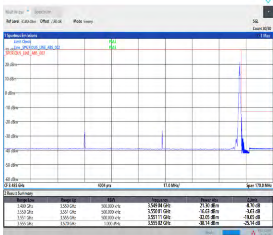
1-N78-3450-3550--30-100-H-2-DFT-PI2BPSK-Edge_1 RB_Right-1@272-Ant1-1--PASS-see graph
