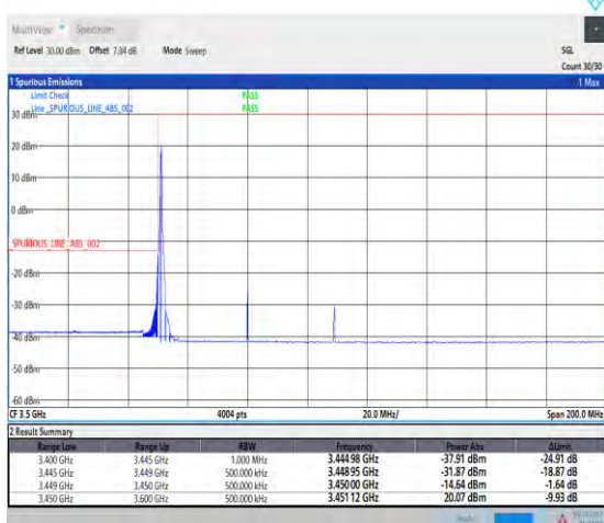
1-N78-3450-3550--30-60-L-4-CP-QPSK-Edge_1RB_L eft-1@0-Ant1-1--PASS-see graph
