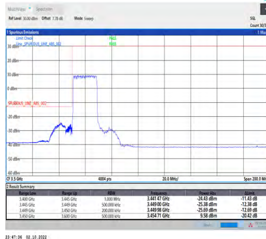
1-N78-3450-3550--30-20-L-3-DFT-PI2BPSK-Outer_Full-50@0-Ant1-1--PASS-see graph
