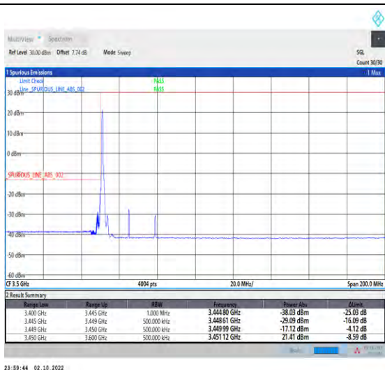
1-N78-3450-3550--30-30-L-1-DFT-PI2BPSK-Edge_1R_B_Left-1@0-Ant1-1--PASS-see graph
