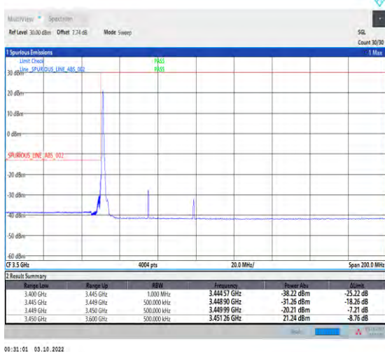
1-N78-3450-3550--30-50-L-4-CP-QPSK-Edge_1RB_L eft-1@0-Ant1-1--PASS-see graph
