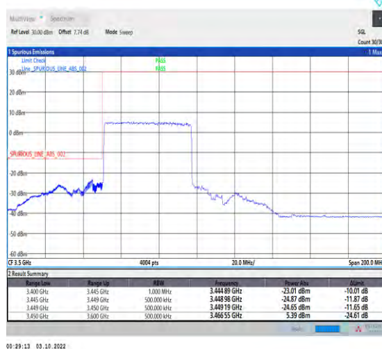
1-N78-3450-3550--30-50-L-6-CP-QPSK-Outer_Ful l-133@0-Ant1-1--PASS-see graph
