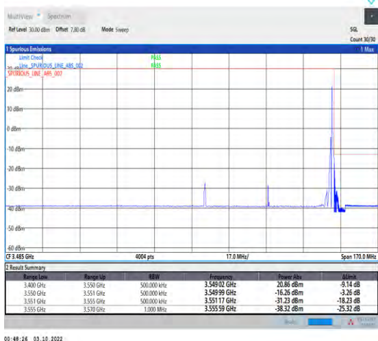
1-N78-3450-3550--30-60-H-2-DFT-PI2BPSK-Edge_1R B_Right-1@161-Ant1-1--PASS-see graph
