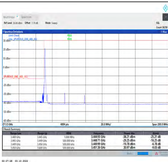
1-N78-3450-3550--30-50-L-1-DFT-PI2BPSK-Edge_1R B_Left-1@0-Ant1-1--PASS-see graph
