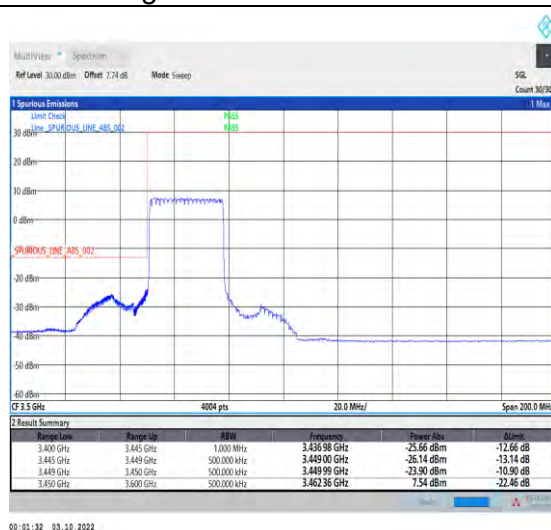
1-N78-3450-3550--30-30-L-3-DFT-PI2BPSK-Outer_Full-75@0-Ant1-1--PASS-see graph
