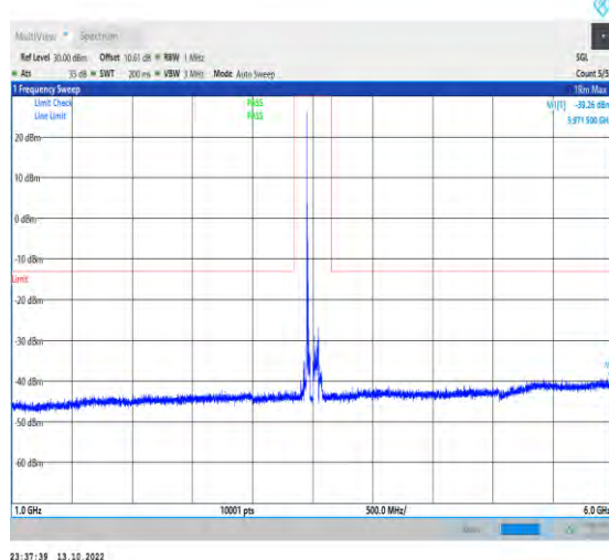
1-N78-3450-3550-PC2-30-100-H-1-DFT-PI2BPSK-In nner_1RB_Left-1@1-1000-6000-Ant1-5979.00--40.15- -13-PASS
