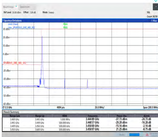
1-N78-3450-3550--30-60-L-1-DFT-PI2BPSK-Edge_1R_B_Left-1@0-Ant1-1--PASS-see graph
