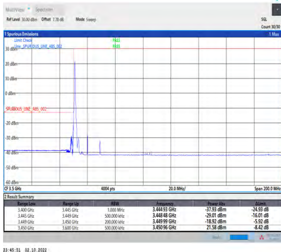
1-N78-3450-3550--30-20-L-1-DFT-PI2BPSK-Edge_1R_B_Left-1@0-Ant1-1--PASS-see graph
