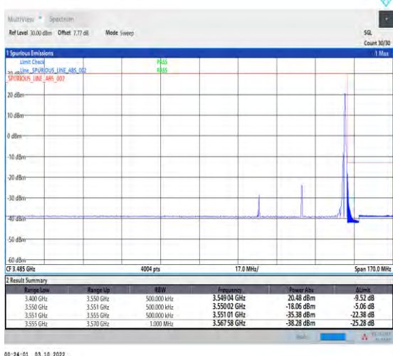
1-N78-3450-3550--30-40-H-5-CP-QPSK-Edge_1RB_R ight-1@105-Ant1-1--PASS-see graph
