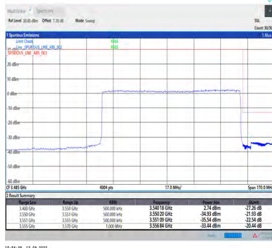
1-N78-3450-3550--30-90-H-3-DFT-PI2BPSK-Outer _Full-240@0-Ant1-1--PASS-see graph
