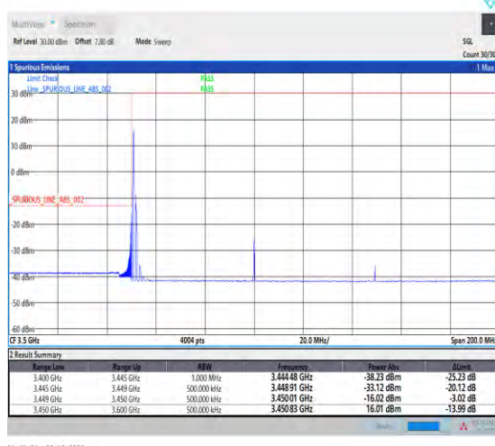
1-N78-3450-3550--30-100-L-4-CP-QPSK-Edge_1RB_ Left-1@0-Ant1-1--PASS-see graph
