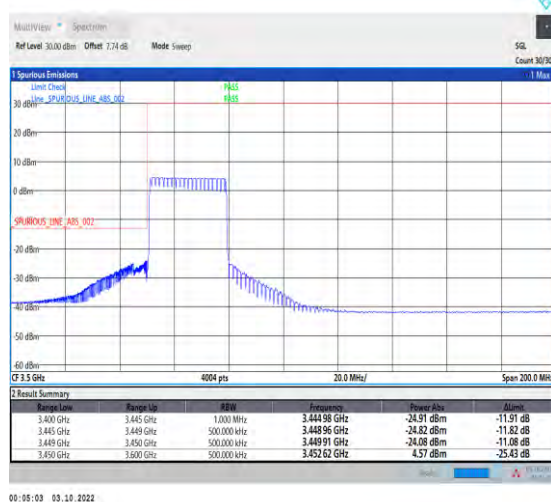
1-N78-3450-3550--30-30-L-6-CP-QPSK-Outer_Ful l-78@0-Ant1-1--PASS-see graph
