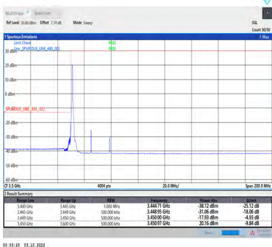
1-N78-3450-3550--30-30-L-4-CP-QPSK-Edge_1RB_L eft-1@0-Ant1-1--PASS-see graph
