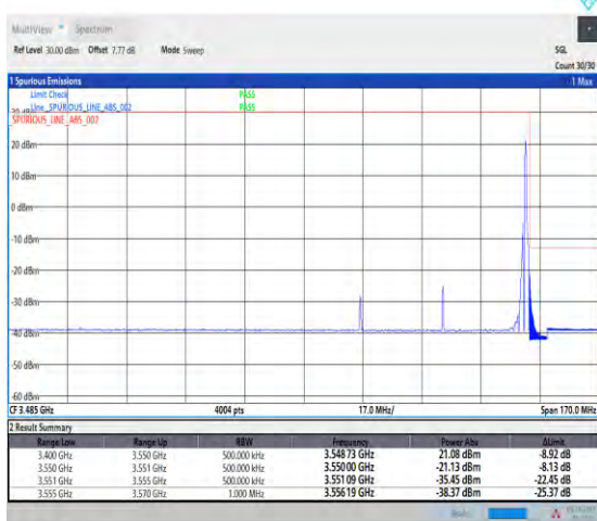
1-N78-3450-3550--30-50-H-5-CP-QPSK-Edge_1RB_R ight-1@132-Ant1-1--PASS-see graph
