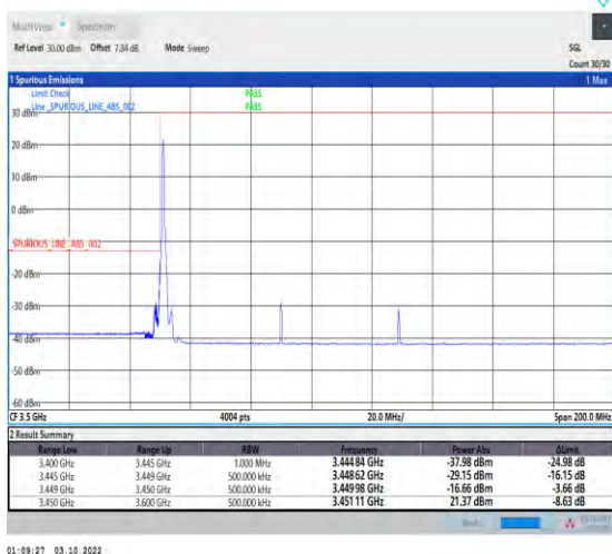
1-N78-3450-3550--30-80-L-1-DFT-PI2BPSK-Edge_1R_B_Left-1@0-Ant1-1--PASS-see graph
