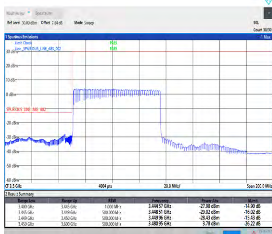
1-N78-3450-3550--30-70-L-6-CP-QPSK-Outer_Ful l-189@0-Ant1-1--PASS-see graph
