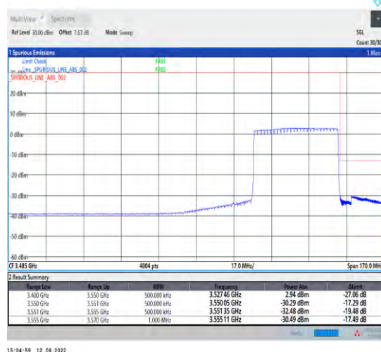
1-N78-3450-3550--30-40-H-6-CP-QPSK-Outer_Ful I-106@0-Ant1-1--PASS-see graph
