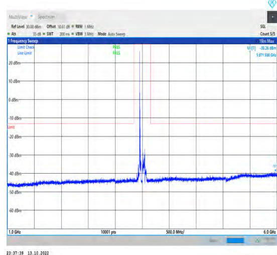
1-N78-3450-3550-PC2-30-100-L-1-DFT-PI2BPSK-Inn er_1RB_Left-1@1-1000-6000-Ant1-5885.00--39.71-- 13-PASS
