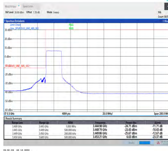
1-N78-3450-3550--30-20-L-6-CP-QPSK-Outer_Ful l-51@0-Ant1-1--PASS-see graph
