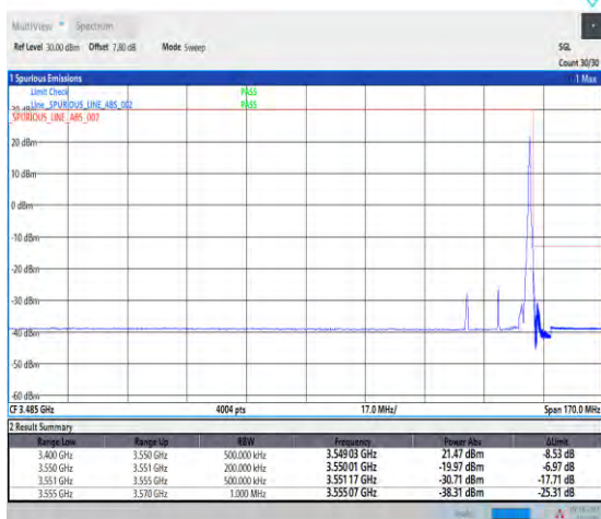
1-N78-3450-3550--30-20-H-2-DFT-PI2BPSK-Edge_1R B_Right-1@50-Ant1-1--PASS-see graph
