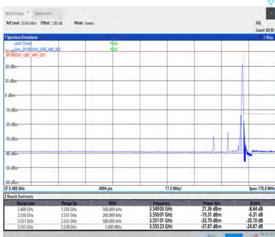
1-N78-3450-3550--30-20-H-5-CP-QPSK-Edge_1RB_R ight-1@50-Ant1-1--PASS-see graph
