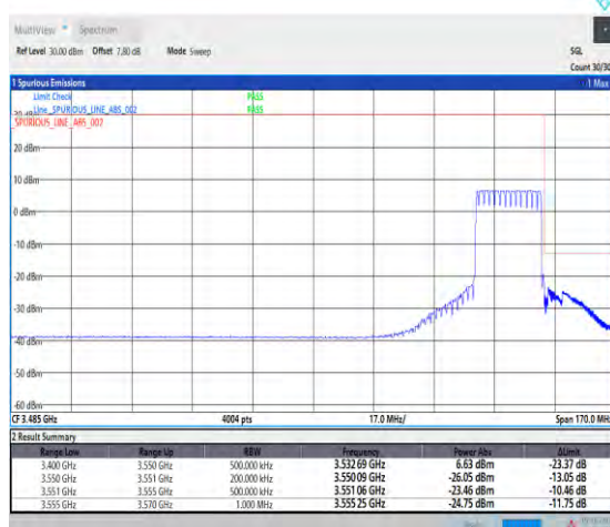
1-N78-3450-3550--30-20-H-6-CP-QPSK-Outer_Ful l-51@0-Ant1-1--PASS-see graph
