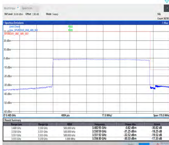
1-N78-3450-3550--30-100-H-6-CP-QPSK-Outer_F ull-273@0-Ant1-1--PASS-see graph
