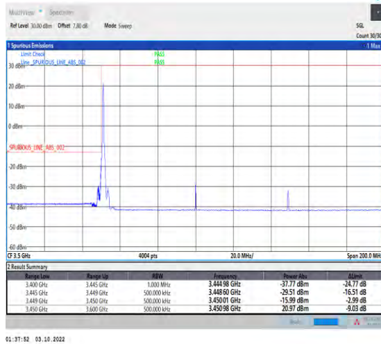
1-N78-3450-3550--30-100-L-1-DFT-PI2BPSK-Edge_1 RB_Left-1@0-Ant1-1--PASS-see graph
