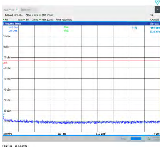
1-N78-3450-3550-PC2-30-100-L-1-DFT-PI2BPSK-In ner_1RB_Left-1@1-30-1000-Ant1-33.40--66.60--13- PASS
