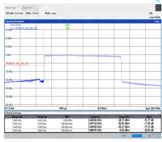
1-N78-3450-3550--30-100-L-6-CP-QPSK-Outer_F ull-273@0-Ant1-1--PASS-see graph
