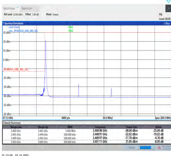
1-N78-3450-3550--30-80-L-4-CP-QPSK-Edge_1RB_L eft-1@0-Ant1-1--PASS-see graph
