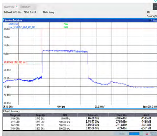
1-N78-3450-3550--30-60-L-3-DFT-PI2BPSK-Outer_Full-162@0-Ant1-1--PASS-see graph
