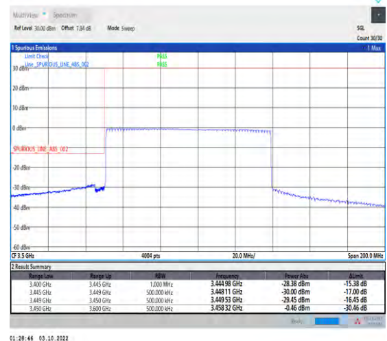
1-N78-3450-3550--30-90-L-6-CP-QPSK-Outer_Ful I-245@0-Ant1-1--PASS-see graph
