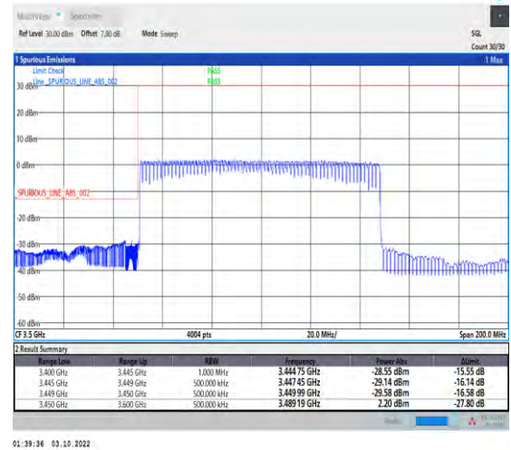
1-N78-3450-3550--30-100-L-3-DFT-PI2BPSK-Oute r_Full-270@0-Ant1-1--PASS-see graph
