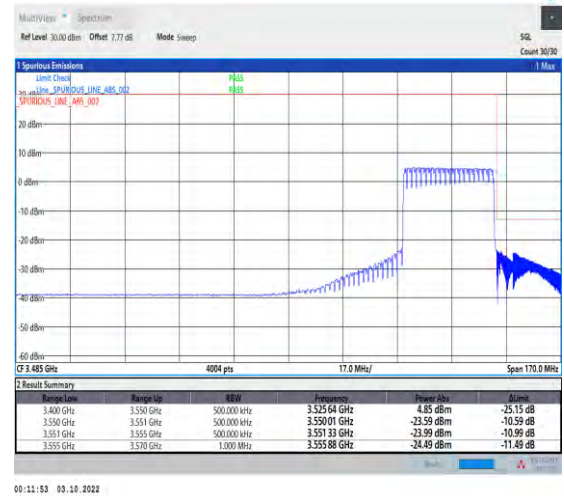
1-N78-3450-3550--30-30-H-3-DFT-PI2BPSK-Outer _Full-75@0-Ant1-1--PASS-see graph
