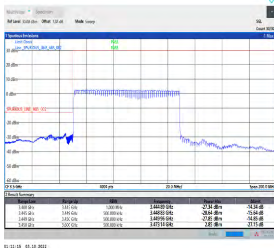
1-N78-3450-3550--30-80-L-3-DFT-PI2BPSK-Outer_Full-216@0-Ant1-1--PASS-see graph
