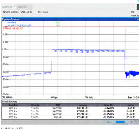
1-N78-3450-3550--30-90-H-6-CP-QPSK-Outer_Ful I-245@0-Ant1-1--PASS-see graph
