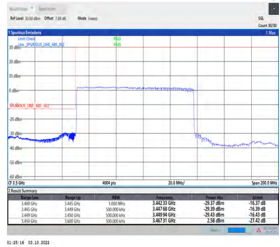
1-N78-3450-3550--30-90-L-3-DFT-PI2BPSK-Outer _Full-240@0-Ant1-1--PASS-see graph
