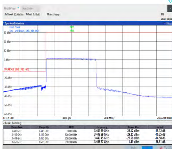
1-N78-3450-3550--30-60-L-6-CP-QPSK-Outer_Ful l-162@0-Ant1-1--PASS-see graph
