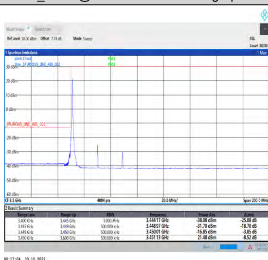
1-N78-3450-3550--30-40-L-4-CP-QPSK-Edge_1RB_L eft-1@0-Ant1-1--PASS-see graph
