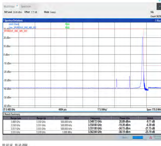
1-N78-3450-3550--30-30-H-5-CP-QPSK-Edge_1RB_R ight-1@77-Ant1-1--PASS-see graph
