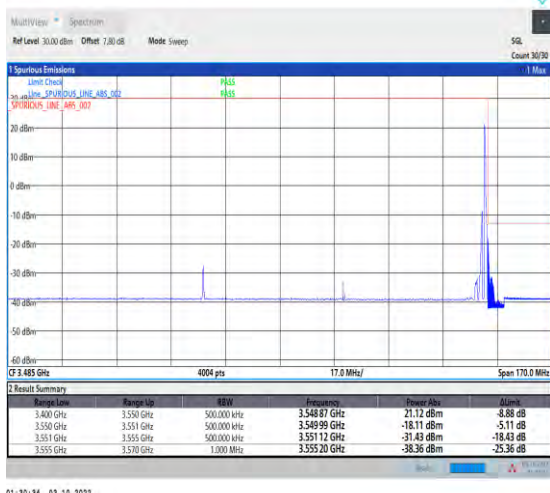
1-N78-3450-3550--30-90-H-2-DFT-PI2BPSK-Edge_1R B_Right-1@244-Ant1-1--PASS-see graph
