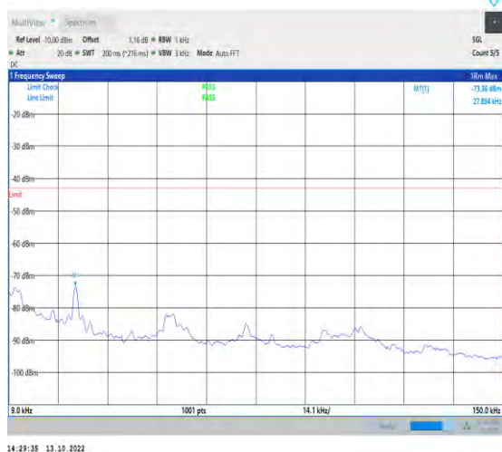
1-N78-3450-3550-PC2-30-100-L-1-DFT-PI2BPSK-In ner_1RB_Left-1@1-0.009-0.15-Ant1-0.03--73.36--4 3-PASS
