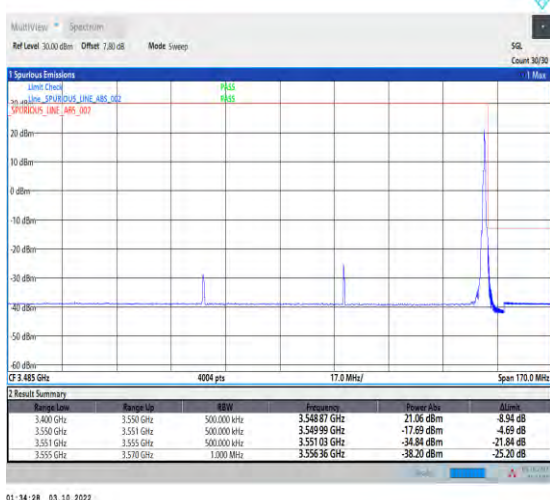
1-N78-3450-3550--30-90-H-5-CP-QPSK-Edge_1RB_R ight-1@244-Ant1-1--PASS-see graph
