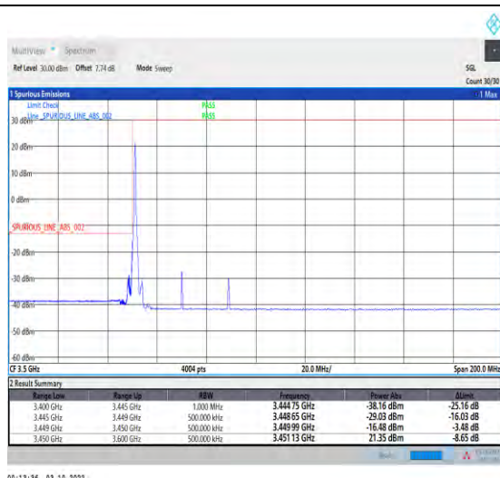
1-N78-3450-3550--30-40-L-1-DFT-PI2BPSK-Edge_1R B_Left-1@0-Ant1-1--PASS-see graph
