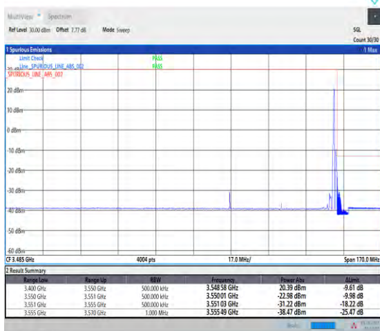
1-N78-3450-3550--30-50-H-2-DFT-PI2BPSK-Edge_1R B_Right-1@132-Ant1-1--PASS-see graph
