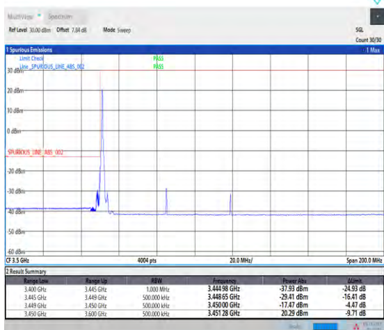
1-N78-3450-3550--30-70-L-1-DFT-PI2BPSK-Edge_1R B_Left-1@0-Ant1-1--PASS-see graph
