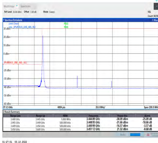
1-N78-3450-3550--30-90-L-4-CP-QPSK-Edge_1RB_L eft-1@0-Ant1-1--PASS-see graph
