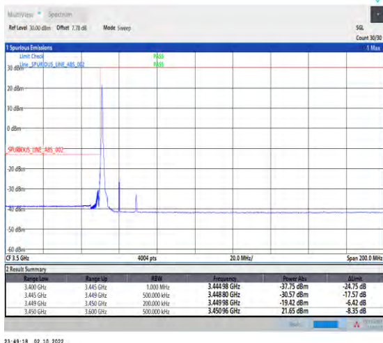
1-N78-3450-3550--30-20-L-4-CP-QPSK-Edge_1RB_L eft-1@0-Ant1-1--PASS-see graph
