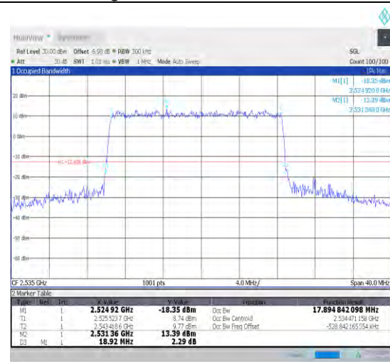
1-N7-15-20-M-3-DFT-16QAM-Outer_Full-100@0-Ant 1-17.895-18.920-≤20-PASS
