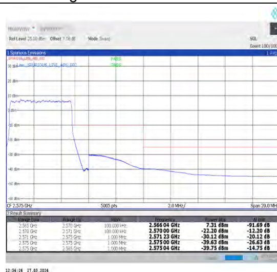
1-N7-15-5-H-3-DFT-PI2BPSK-Outer_Full-25@0-Ant1-1--PASS-see graph
