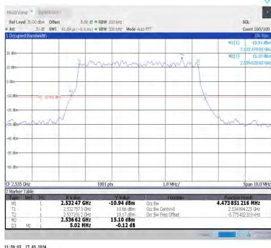
1-N7-15-5-M-1-DFT-QPSK-Outer_Full-25@0-Ant1-4. 474-5.020-≤5-PASS
