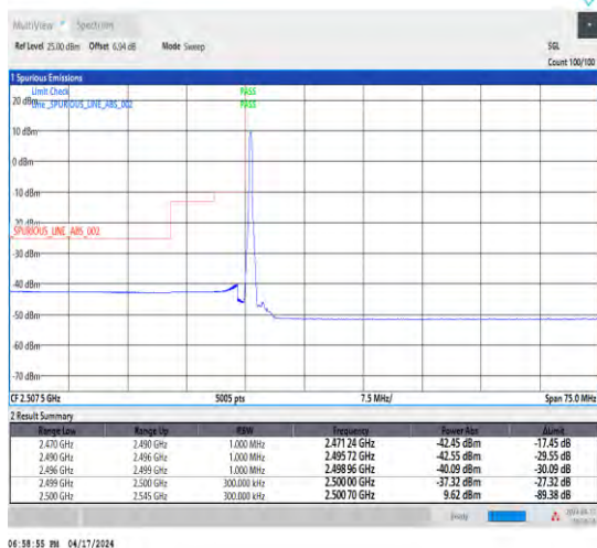
1-N7-15-30-L-1-DFT-PI2BPSK-Edge_1RB_Left-1@0-Ant1-1--PASS-see graph
