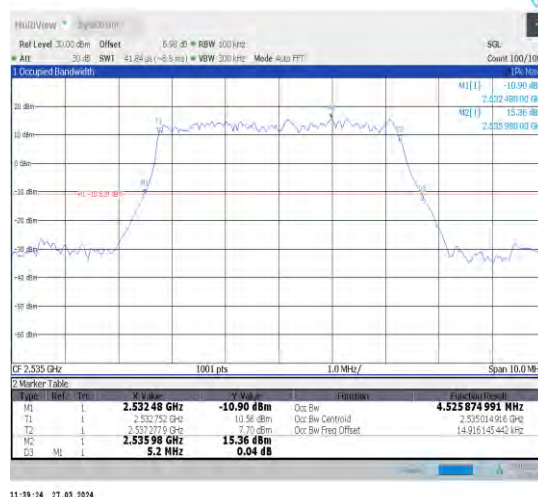
1-N7-15-5-M-2-DFT-PI2BPSK-Outer_Full-25@0-Ant 1-4.526-5.200-≤5-PASS
