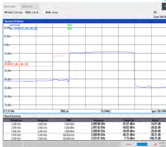
1-N7-15-40-L-3-DFT-PI2BPSK-Outer_Full-216@0-Ant1-1--PASS-see graph
