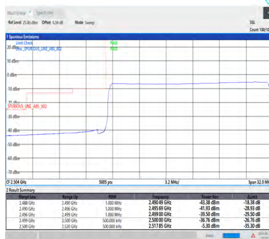
1-N7-15-20-L-6-CP-QPSK-Outer_Full-106@0-Ant1-1--PASS-see graph
