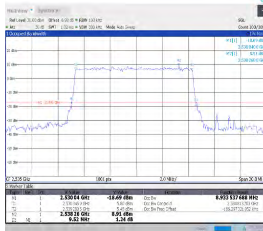
1-N7-15-10-M-5-DFT-256QAM-Outer_Full-50@0-Ant 1-8.934-9.520-≤10-PASS
