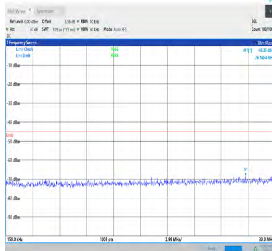
1-N7-15-40-H-1-DFT-PI2BPSK-Inner_1RB_Left-1@ -0.15-30-Ant1-29.79--68.35--45-PASS
