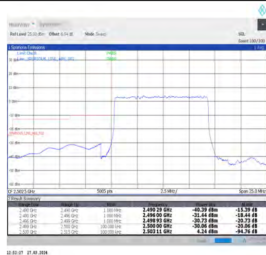
1-N7-15-10-L-3-DFT-PI2BPSK-Outer_Full-50@0-A Ant1-1--PASS-see graph
