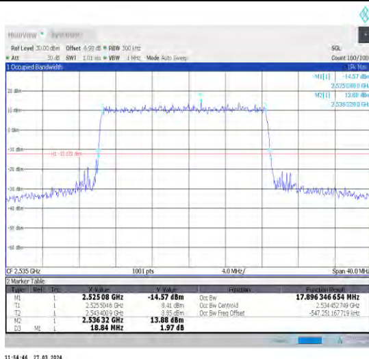
1-N7-15-20-M-4-DFT-64QAM-Outer_Full-100@0-Ant 1-17.896-18.840-≤20-PASS
