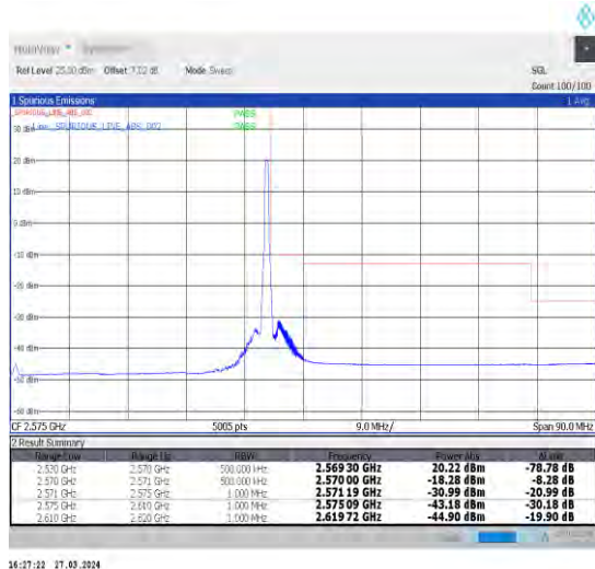
1-N7-15-40-H-5-CP-QPSK-Edge_1RB_Right-1@215-A nt1-1--PASS-see graph
