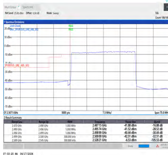
1-N7-15-30-L-3-DFT-PI2BPSK-Outer_Full-160@0-Ant1-1--PASS-see graph
