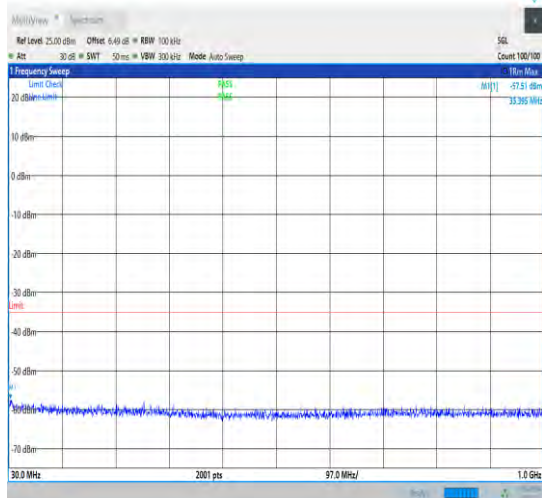
1-N7-15-40-M-1-DFT-PI2BPSK-Inner_1RB_Left-1@ 1-30-1000-Ant1-30.00--57.51--35-PASS
