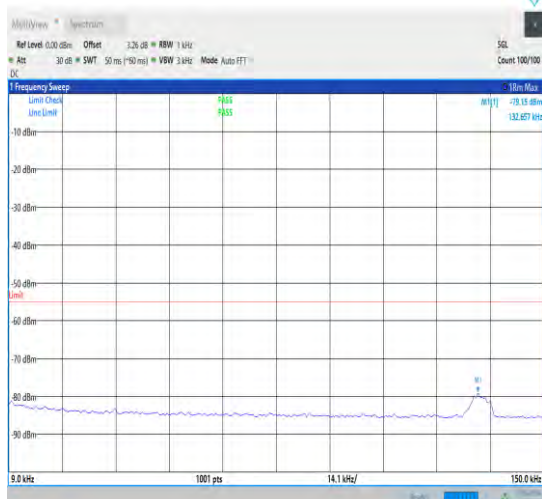
1-N7-15-40-M-1-DFT-PI2BPSK-Inner_1RB_Left-1@ 1-0.009-0.15-Ant1-0.13--79.15--55-PASS
