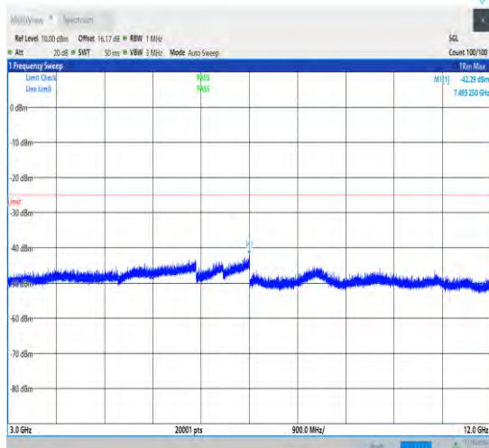
1-N7-15-40-M-1-DFT-PI2BPSK-Inner_1RB_Left-1@ 1-3000-12000-Ant1-7449.60--42.29--25-PASS
