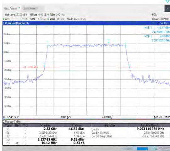
1-N7-15-10-M-6-CP-QPSK-Outer_Full-52@0-Ant1-9. 293-10.120-≤10-PASS
