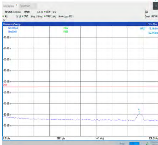
1-N7-15-40-H-1-DFT-PI2BPSK-Inner_1RB_Left-1@ 1-0.009-0.15-Ant1-0.13--79.16--55-PASS
