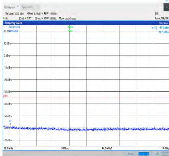
1-N7-15-40-L-1-DFT-PI2BPSK-Inner_1RB_Left-1@ 1-30-1000-Ant1-33.40--57.78--35-PASS
