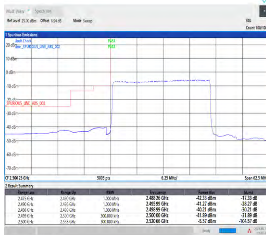
1-N7-15-25-L-3-DFT-PI2BPSK-Outer_Full-128@0-Ant1-1--PASS-see graph
