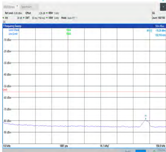
1-N7-15-40-M-1-DFT-PI2BPSK-Inner_1RB_Left-1@ 1-0.009-0.15-Ant1-0.13--79.28--55-PASS
