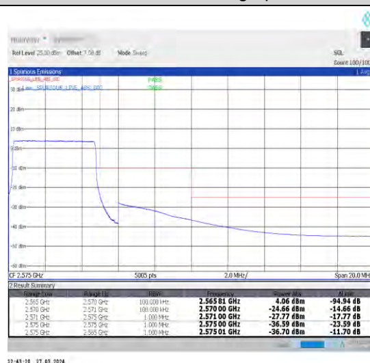
1-N7-15-5-H-6-CP-QPSK-Outer_Full-25@0-Ant1-1--PASS-see graph
