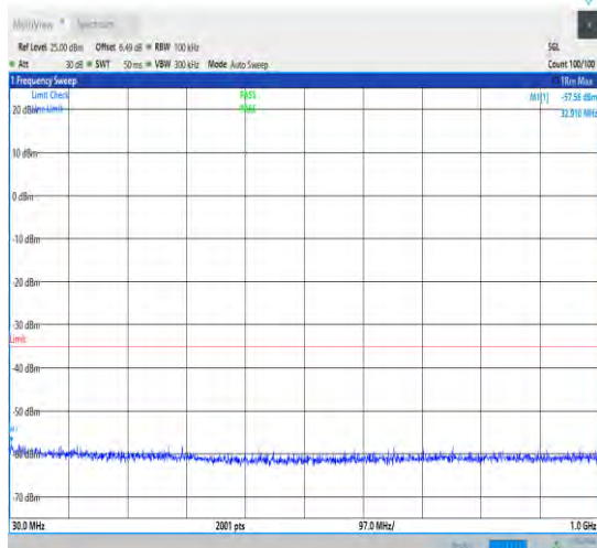
1-N7-15-40-H-1-DFT-PI2BPSK-Inner_1RB_Left-1@ 1-30-1000-Ant1-33.40--57.58--35-PASS
