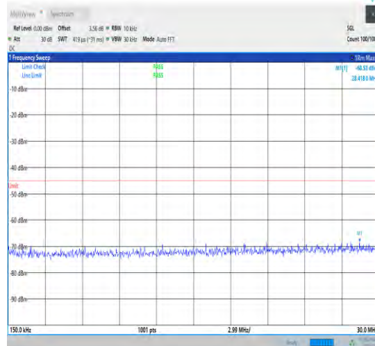
1-N7-15-40-H-1-DFT-PI2BPSK-Inner_1RB_Left-1@ -0.15-30-Ant1-29.79--68.53--45-PASS
