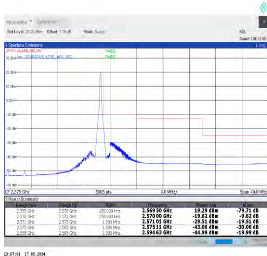
1-N7-15-15-H-5-CP-QPSK-Edge_1RB_Right-1@78-An t1-1--PASS-see graph
