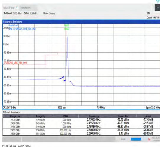
1-N7-15-30-L-4-CP-QPSK-Edge_1RB_Left-1@0-Ant1-1--PASS-see graph
