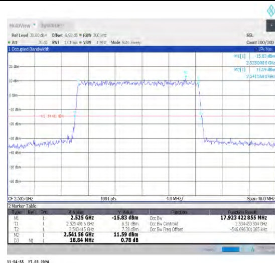
1-N7-15-20-M-5-DFT-256QAM-Outer_Full-100@0-A nt1-17.923-18.840-≤20-PASS
