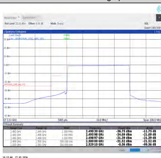
1-N7-15-40-L-6-CP-QPSK-Outer_Full-216@0-Ant1-1--PASS-see graph
