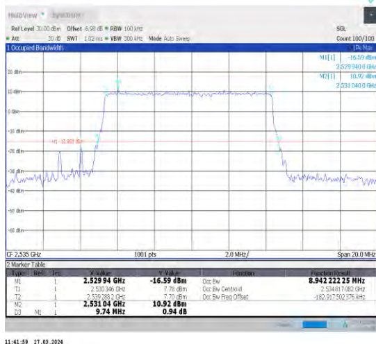
1-N7-15-10-M-4-DFT-64QAM-Outer_Full-50@0-Ant1 -8.942-9.740-≤10-PASS
