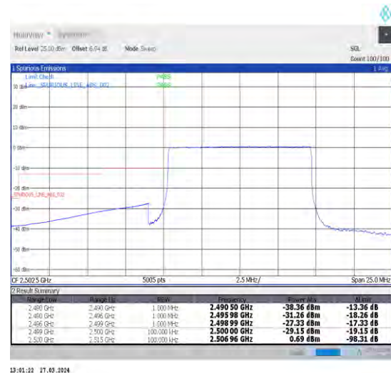
1-N7-15-10-L-6-CP-QPSK-Outer_Full-52@0-A nt1-1--PASS-see graph
