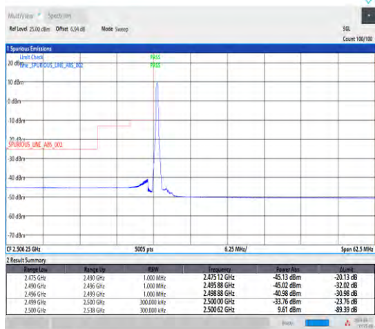
1-N7-15-25-L-1-DFT-PI2BPSK-Edge_1RB_Left-1@0-Ant1-1--PASS-see graph
