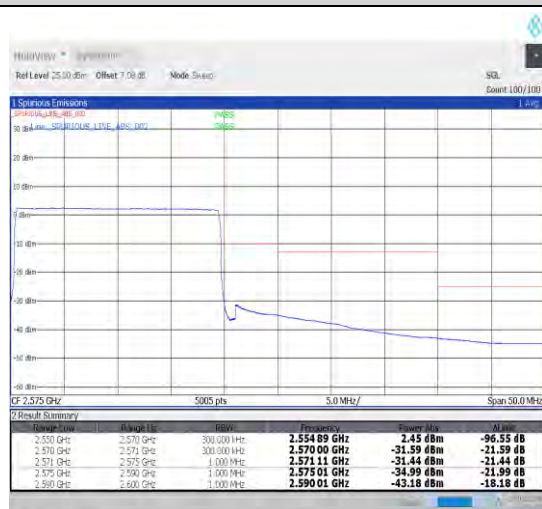
1-N7-15-20-H-3-DFT-PI2BPSK-Outer_Full-100@0 -Ant1-1--PASS-see graph
