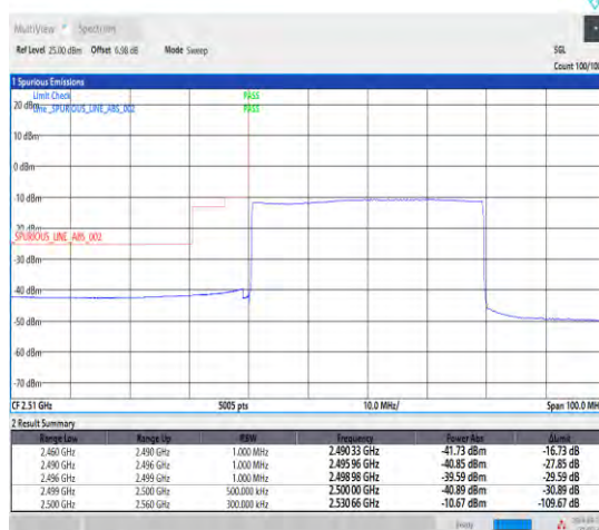
1-N7-15-40-L-6-CP-QPSK-Outer_Full-216@0-Ant1-1--PASS-see graph
