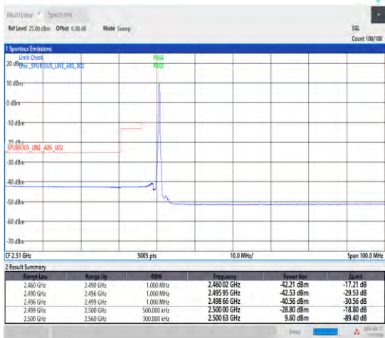
1-N7-15-40-L-1-DFT-PI2BPSK-Edge_1RB_Left-1@0-Ant1-1--PASS-see graph
