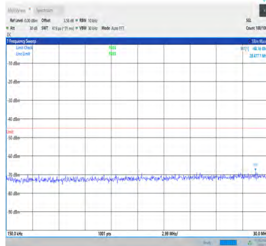
1-N7-15-40-L-1-DFT-PI2BPSK-Inner_1RB_Left-1@1- 0.15-30-Ant1-29.73--68.16--45-PASS
