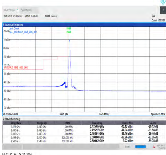
1-N7-15-25-L-4-CP-QPSK-Edge_1RB_Left-1@0-Ant1-1--PASS-see graph
