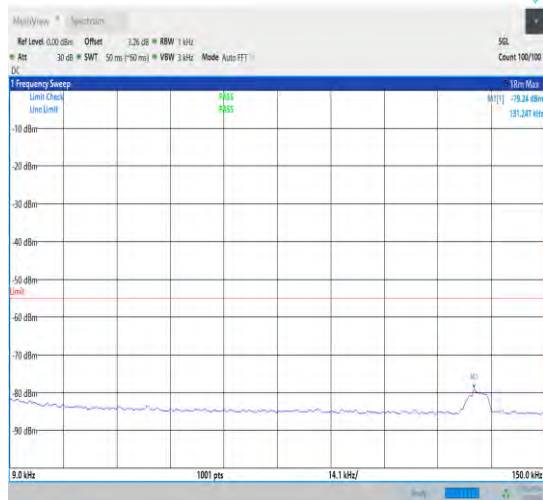
1-N7-15-40-L-1-DFT-PI2BPSK-Inner_1RB_Left-1@ 1-0.009-0.15-Ant1-0.13--79.24--55-PASS
