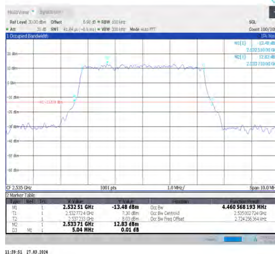
1-N7-15-5-M-4-DFT-64QAM-Outer_Full-25@0-Ant1- 4.461-5.040-≤5-PASS
