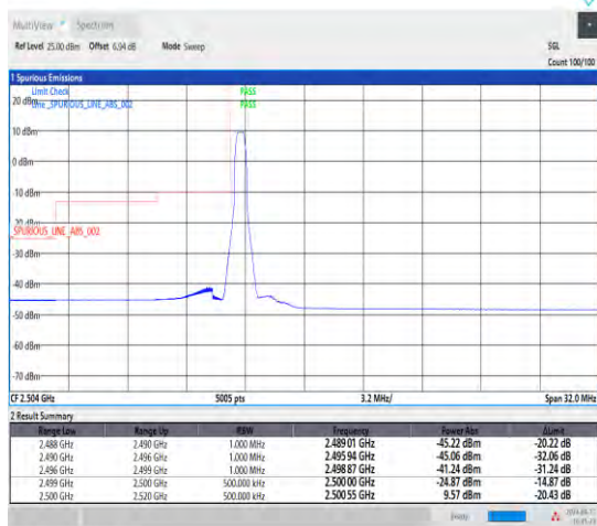
1-N7-15-20-L-1-DFT-PI2BPSK-Edge_1RB_Left-1@0-Ant1-1--PASS-see graph
