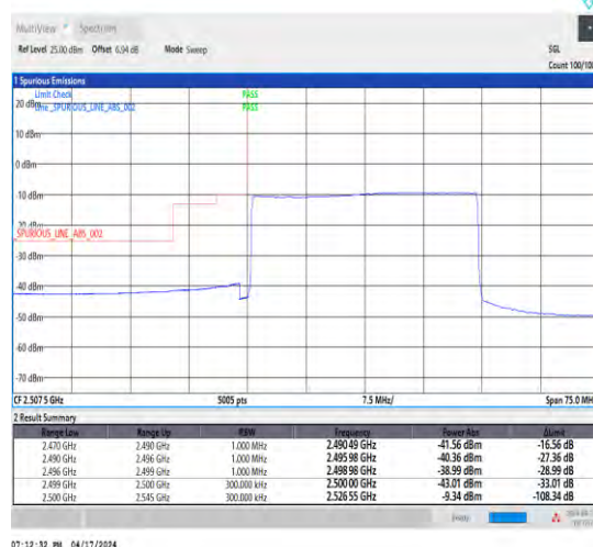
1-N7-15-30-L-6-CP-QPSK-Outer_Full-160@0-Ant1-1--PASS-see graph
