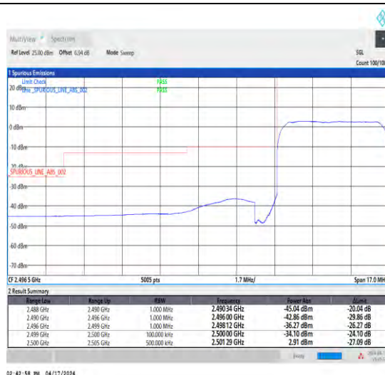
1-N7-15-5-L-3-DFT-PI2BPSK-Outer_Full-25@0-Ant1-1--PASS-see graph
