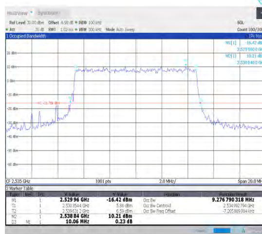
1-N7-15-10-M-7-CP-16QAM-Outer_Full-52@0-Ant1-9. 9.277-10.060-≤10-PASS
