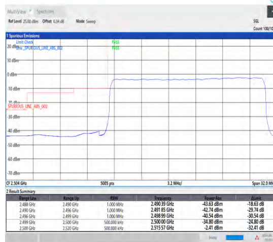
1-N7-15-20-L-3-DFT-PI2BPSK-Outer_Full-100@0-Ant1-1--PASS-see graph
