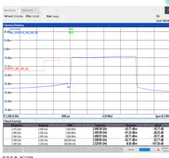
1-N7-15-25-L-6-CP-QPSK-Outer_Full-133@0-Ant1-1--PASS-see graph
