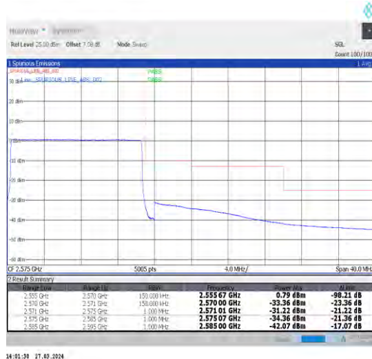
1-N7-15-15-H-6-CP-QPSK-Outer_Full-79@0-Ant1 -1--PASS-see graph
