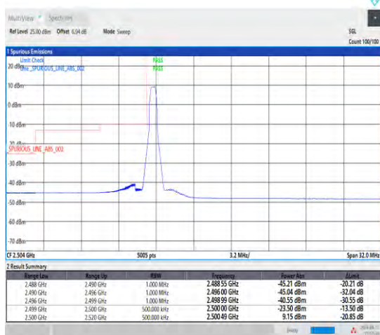
1-N7-15-20-L-4-CP-QPSK-Edge_1RB_Left-1@0-Ant1-1--PASS-see graph
