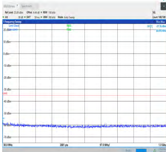
1-N7-15-40-M-1-DFT-PI2BPSK-Inner_1RB_Left-1@ 1-30-1000-Ant1-30.00--57.76--35-PASS
