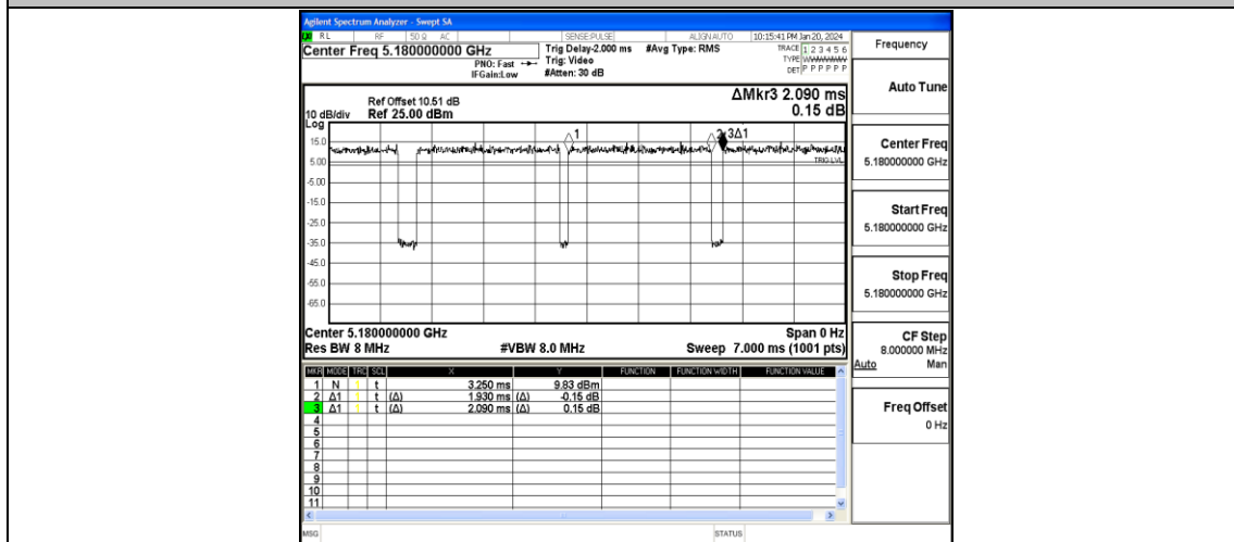
NTNV-11AC20MIMO-Ant2-5180
