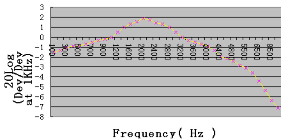
Audio Frequency Response - CH 03
