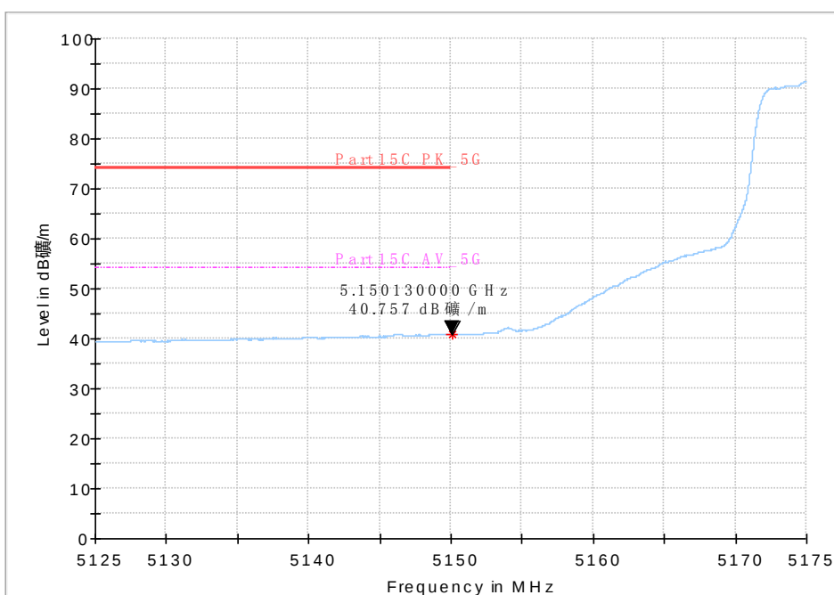
Fig. 45 Band Edges (802.11a, 5180MHz)
