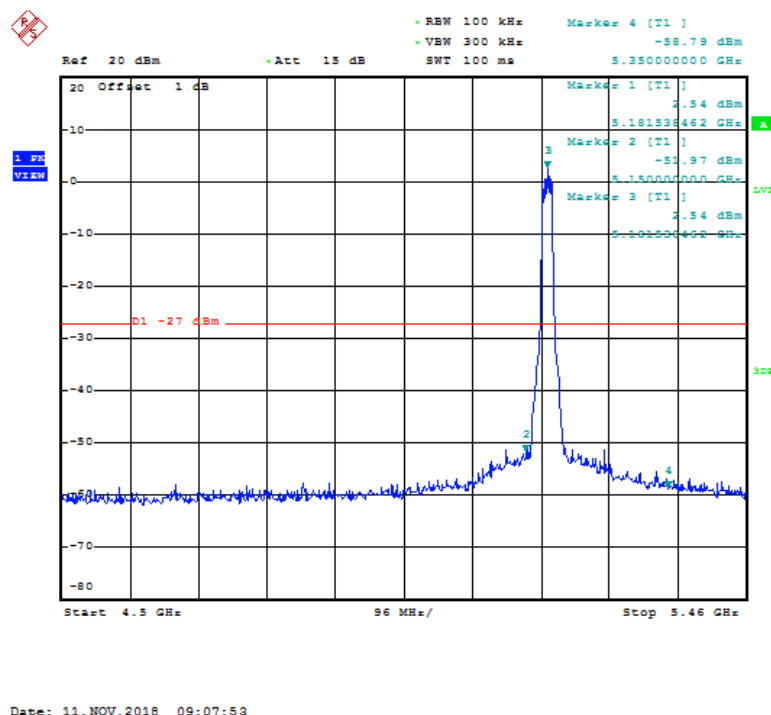
Fig. 37 Band Edges (802.11a, 5180MHz)
