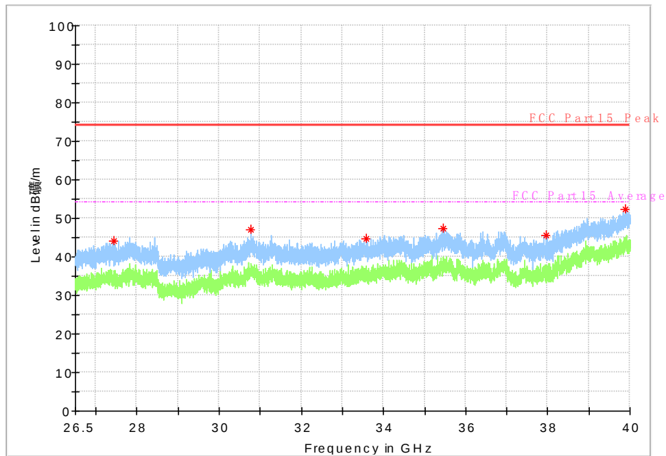
Fig. 61 Radiated Spurious Emission (802.11a, ch36, 26.5 GHz-40 GHz)
