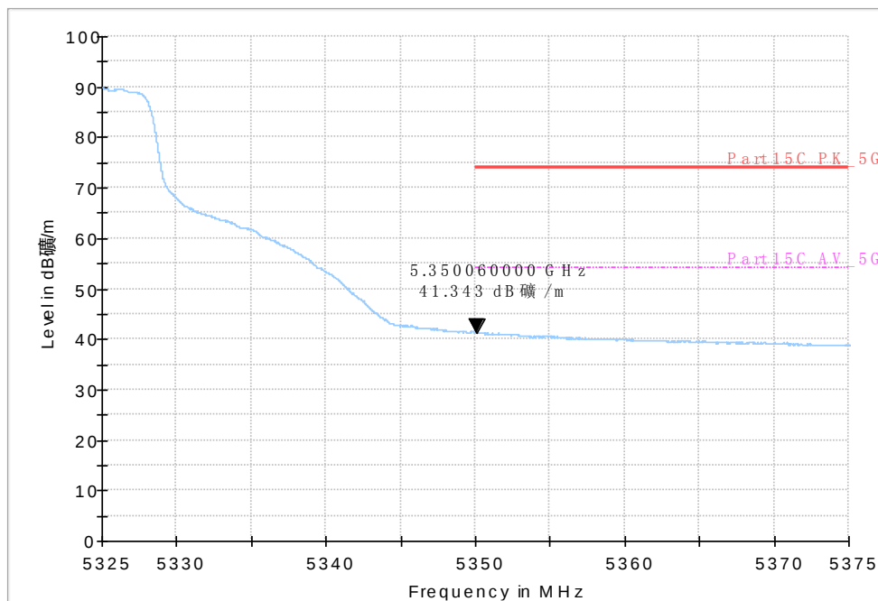
Fig. 46 Band Edges (802.11a, 5320MHz)
