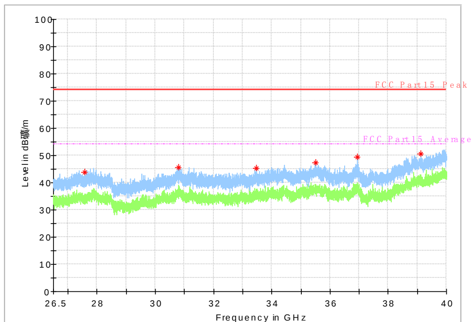
Fig. 56 Radiated Spurious Emission (802.11n-HT20, ch36, 26.5 GHz-40 GHz)
