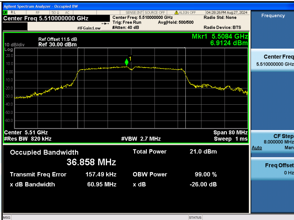
11AC40MIMO-Ant3-5510
