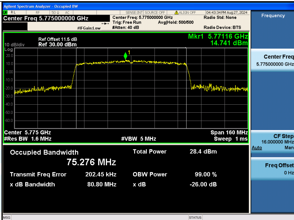
11AC80MIMO-Ant3-5775
