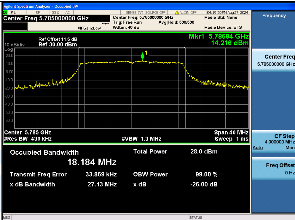
11AC20MIMO-Ant3-5785
