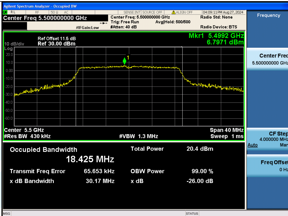
11AC20MIMO-Ant3-5500
