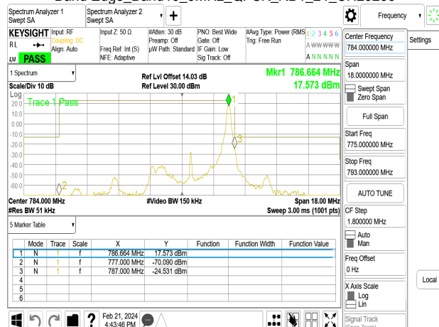
Band Edge_Band13_5MHz_QPSK_RB25_0_CH23205
