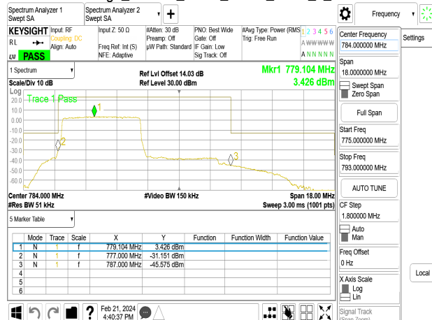
Band Edge_Band13_5MHz_QPSK_RB25_0_CH23255
