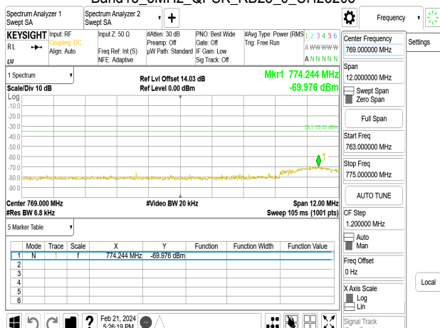
Band13_5MHz_QPSK_RB25_0_CH23205
