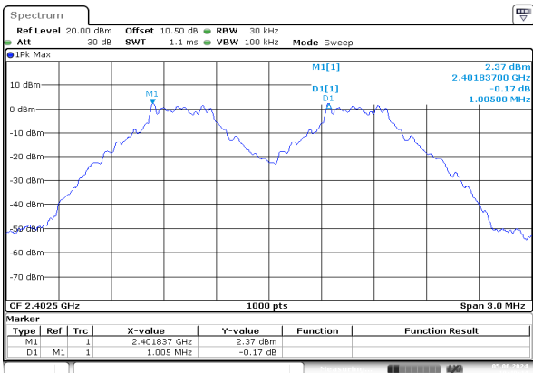
GFSK_Low
