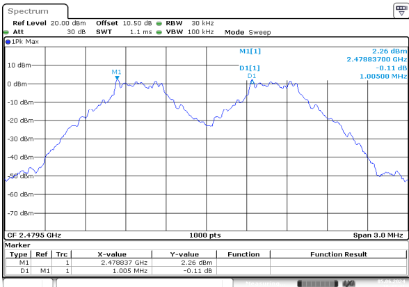
GFSK_High
