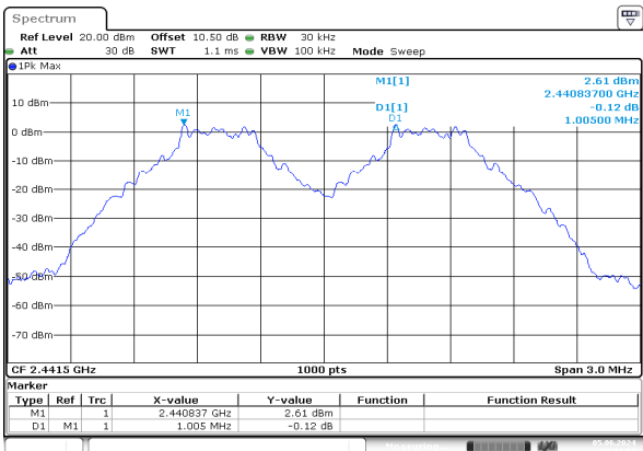
GFSK_Middle
