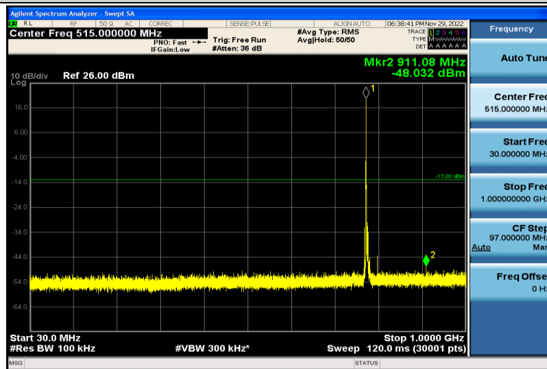
Band13-5MHz-64QAM-23205-1RB#0-30~1000MHz
