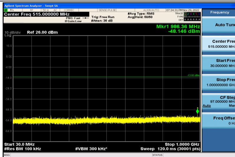
Band66-10MHz-64QAM-132022-1RB#0-30~1000MHz
