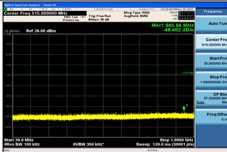
Band66-3MHz-QPSK-132657-1RB#0-30~1000MHz
