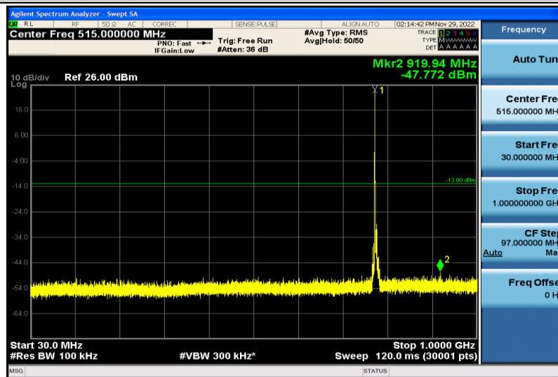
Band13-5MHz-16QAM-23205-1RB#0-30~1000MHz
