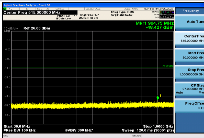
Band66-5MHz-16QAM-131997-1RB#0-30~1000MHz
