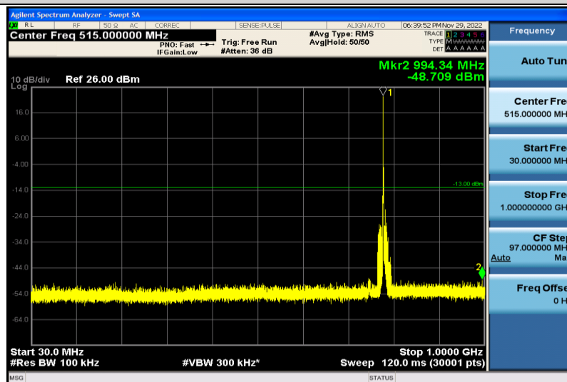
Band13-5MHz-64QAM-23255-1RB#0-30~1000MHz
