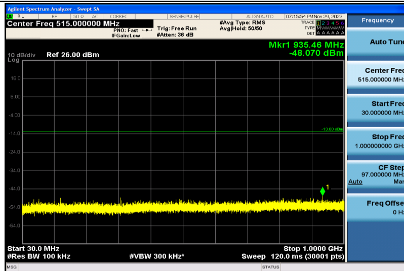
Band66-3MHz-64QAM-132657-1RB#0-30~1000MHz
