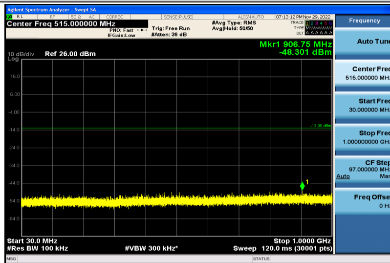
Band66-3MHz-64QAM-131987-1RB#0-30~1000MHz
