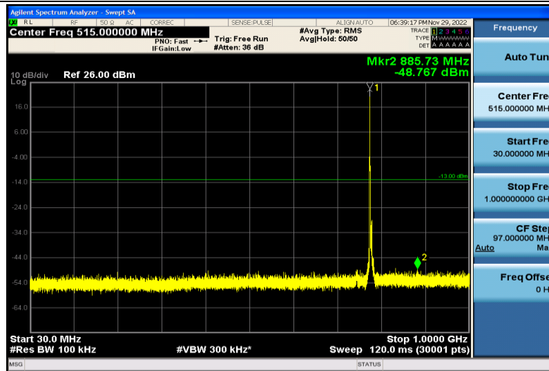
Band13-5MHz-64QAM-23230-1RB#0-30~1000MHz
