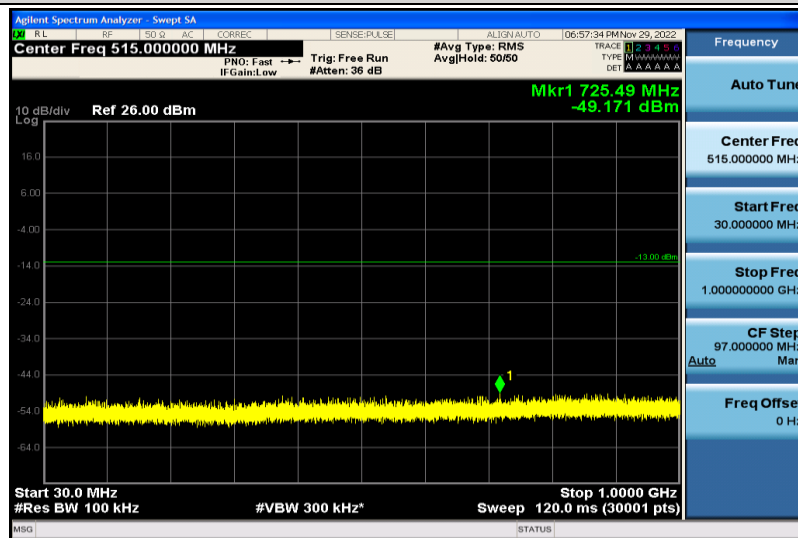
Band66-1.4MHz-64QAM-131979-1RB#0-30~1000MHz
