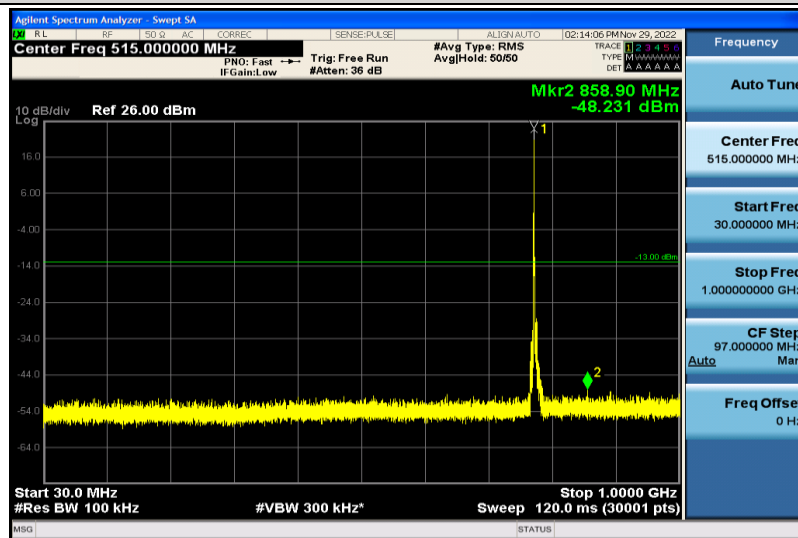
Band13-5MHz-QPSK-23205-1RB#0-30~1000MHz
