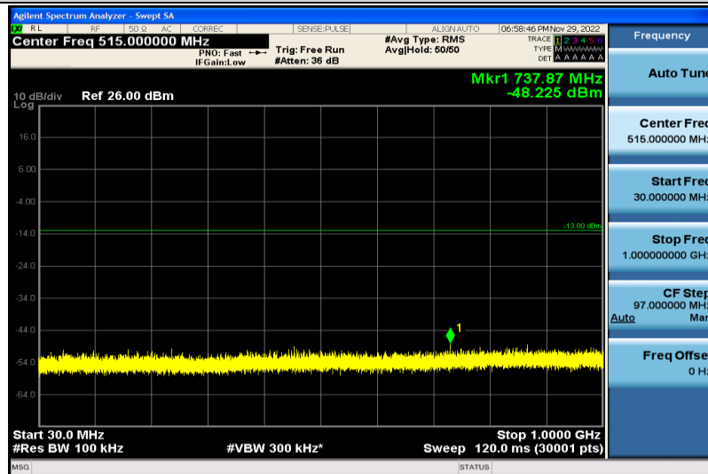
Band66-1.4MHz-64QAM-132665-1RB#0-30~1000MHz
