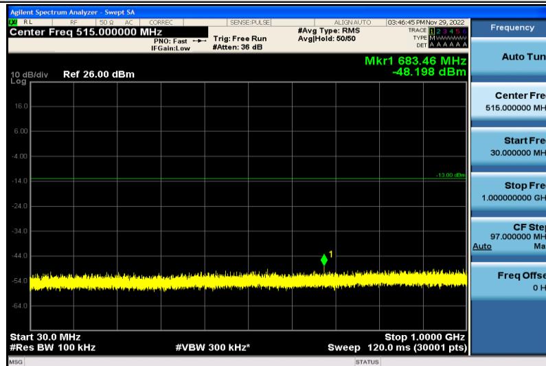
Band66-5MHz-QPSK-132647-1RB#0-30~1000MHz
