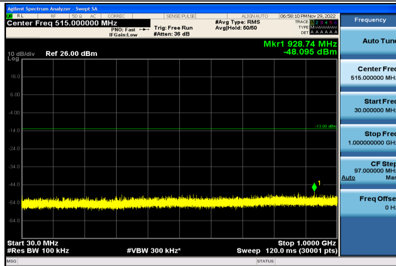
Band66-1.4MHz-64QAM-132322-1RB#0-30~1000MHz
