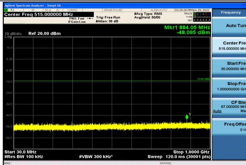
Band66-3MHz-16QAM-132657-1RB#0-30~1000MHz
