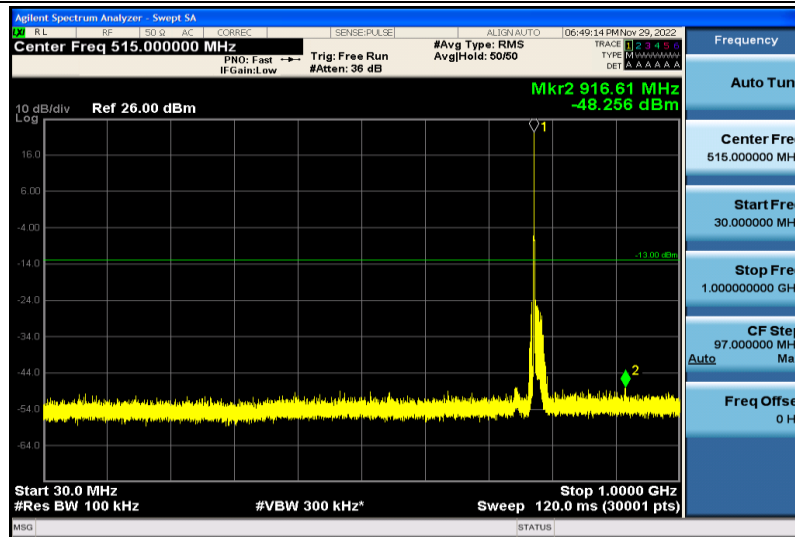
Band13-10MHz-64QAM-23230-1RB#0-30~1000MHz
