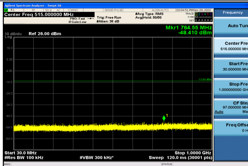
Band66-1.4MHz-QPSK-132665-1RB#0-30~1000MHz
