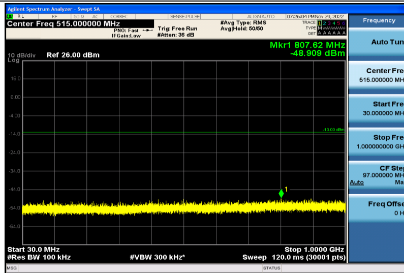
Band66-5MHz-64QAM-132322-1RB#0-30~1000MHz
