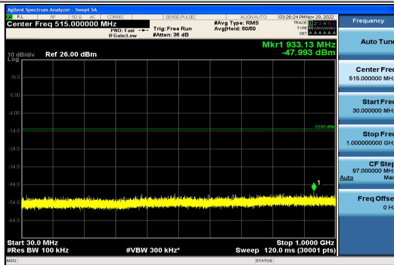
Band66-3MHz-QPSK-131987-1RB#0-30~1000MHz
