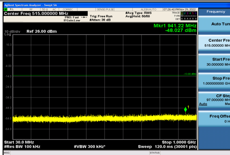
Band66-5MHz-64QAM-132647-1RB#0-30~1000MHz
