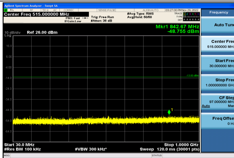
Band66-3MHz-16QAM-131987-1RB#0-30~1000MHz
