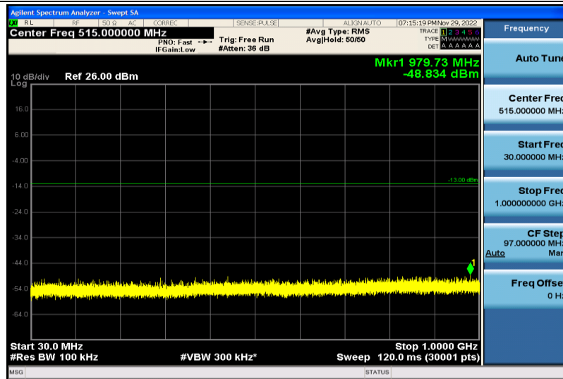
Band66-3MHz-64QAM-132322-1RB#0-30~1000MHz
