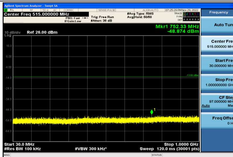
Band66-5MHz-64QAM-131997-1RB#0-30~1000MHz
