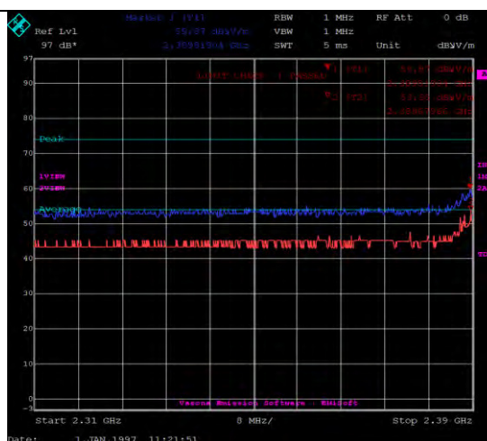
802.11n40 2422M-Restricted Band 2310-2390MHz
