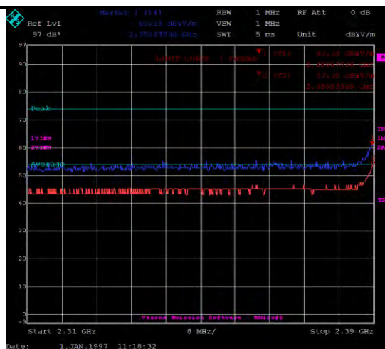
802.11n20 2412M-Restricted Band 2310-2390MHz
