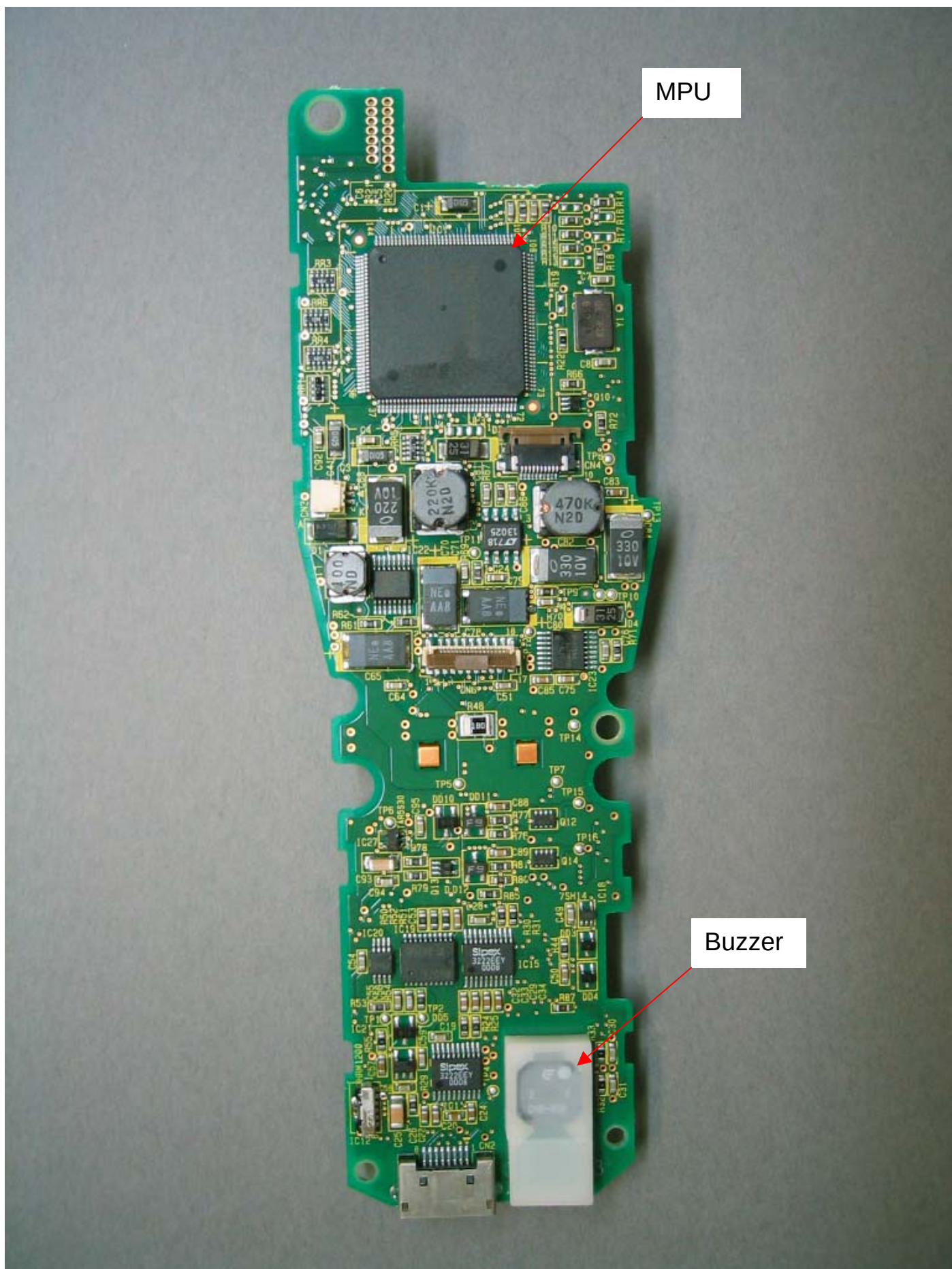
Back side of Main Unit
