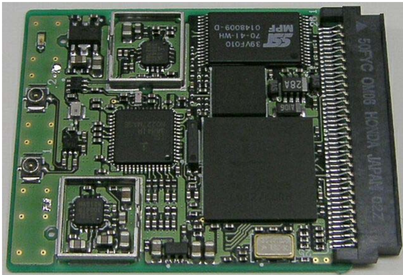
Without shield
