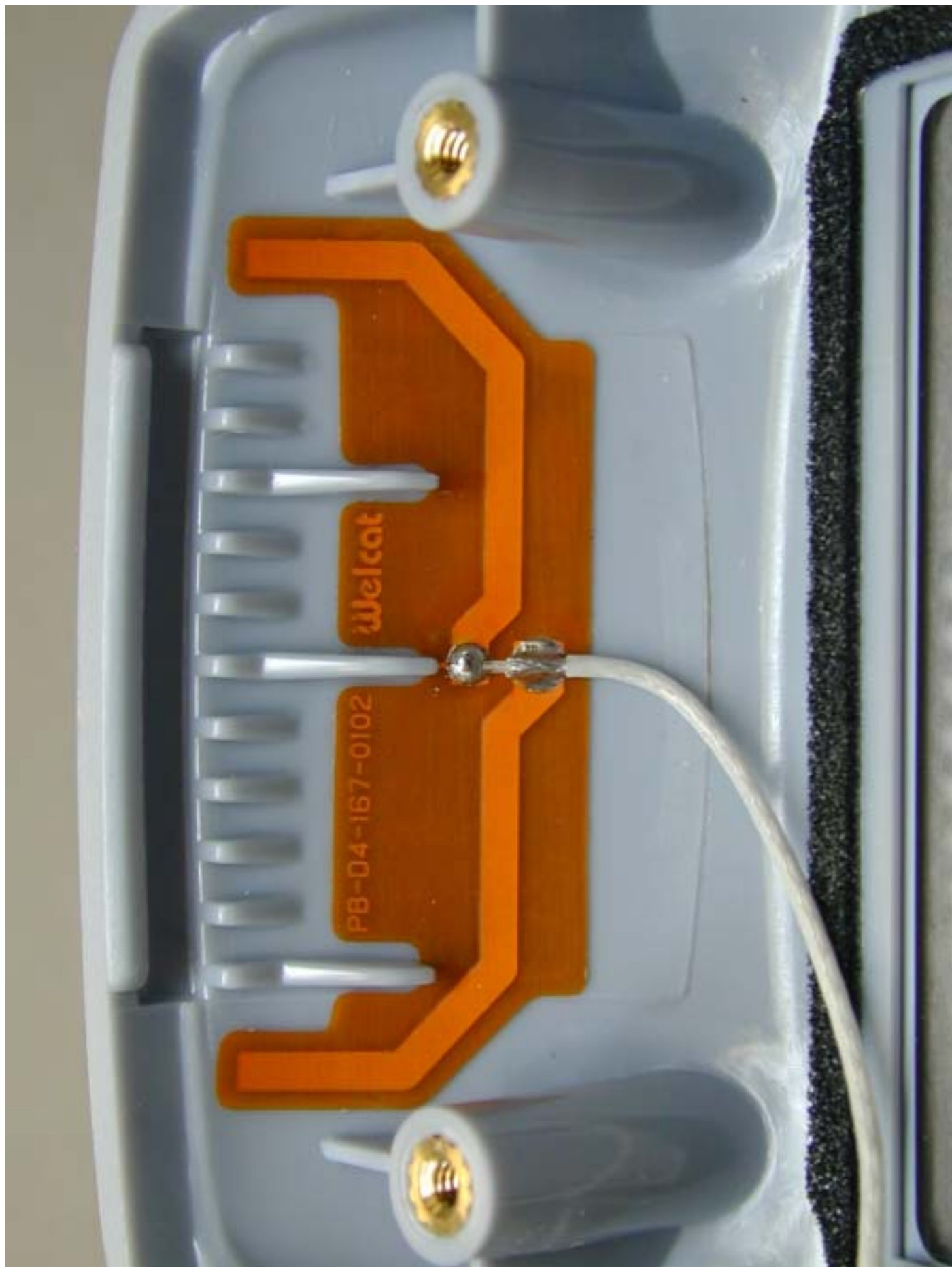
Flexible Antenna
