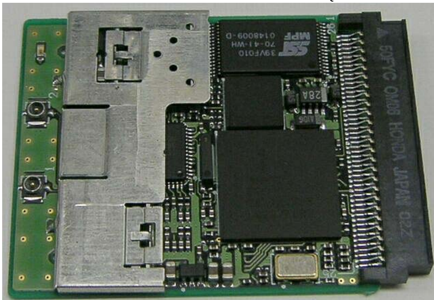
With shield
