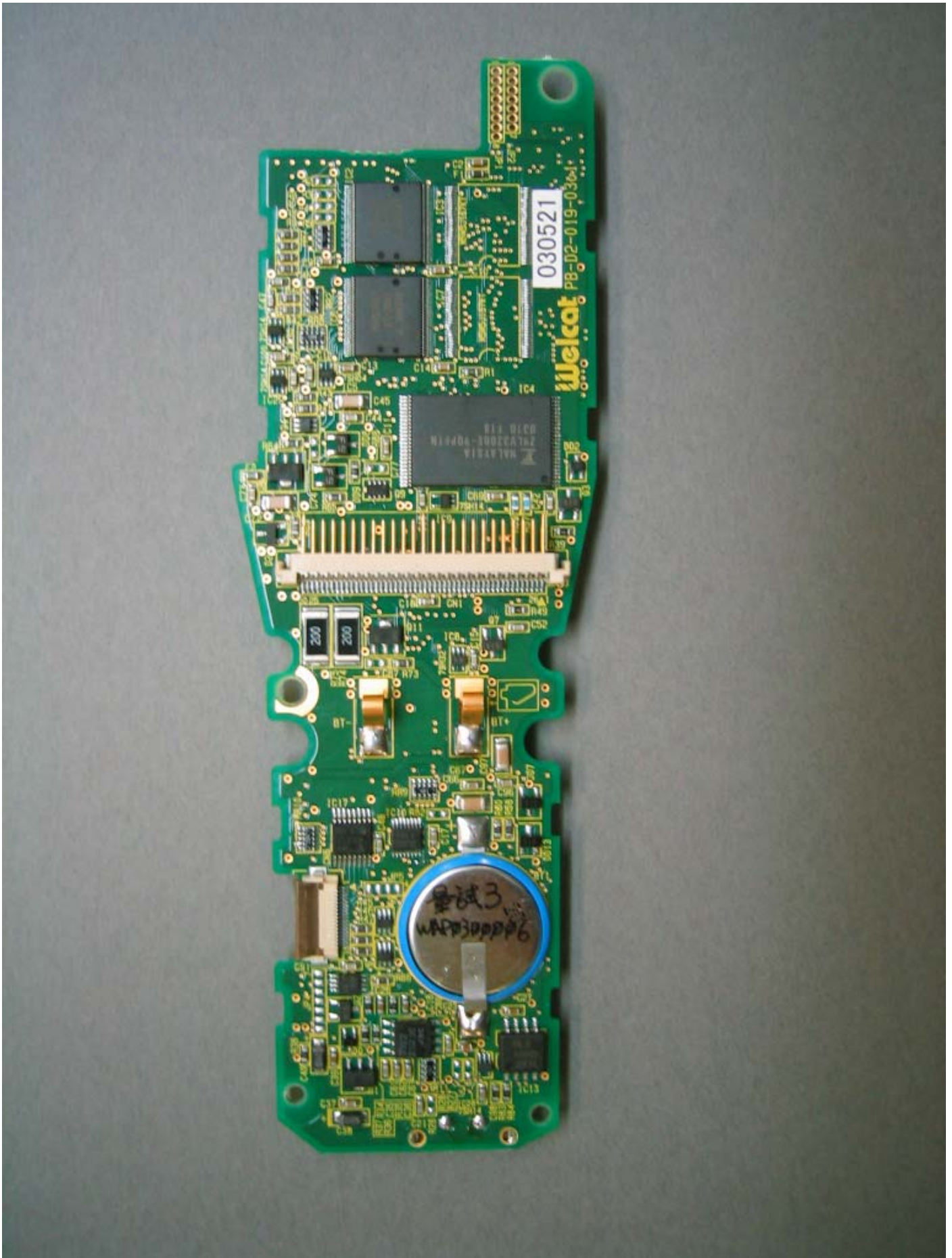
Front side of Main Unit
