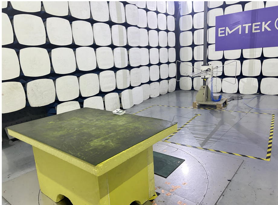
Spurious Emission Test Setup (Below 1GHz)
