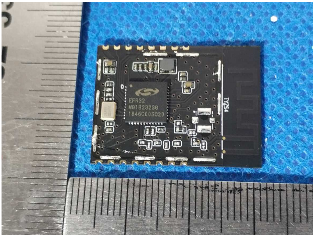
Photo 3. Top view remove the shielding can of Model TYZS4
