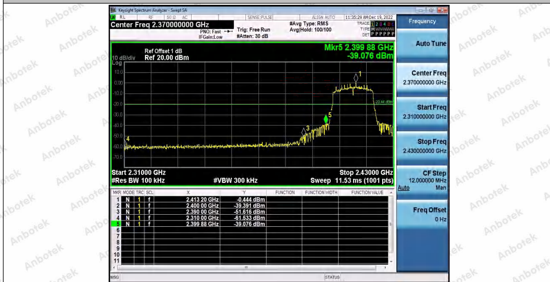
11N20_Ant1_High_2462
