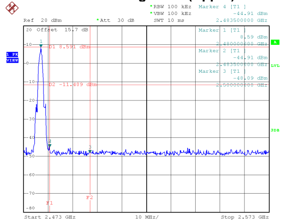
BandedgeCH39(Upper)
