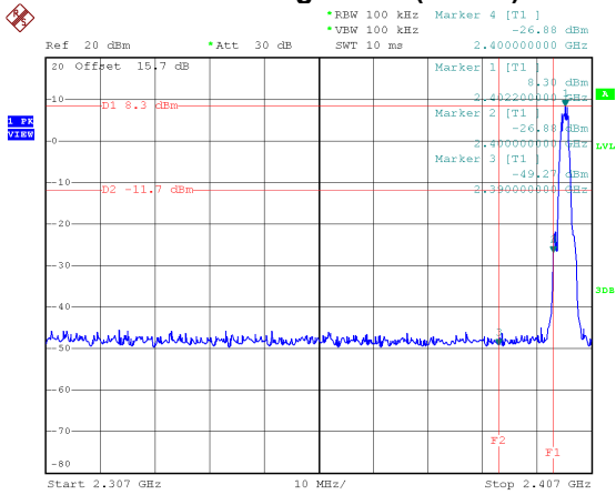
BandedgeCH00 (Lower)
