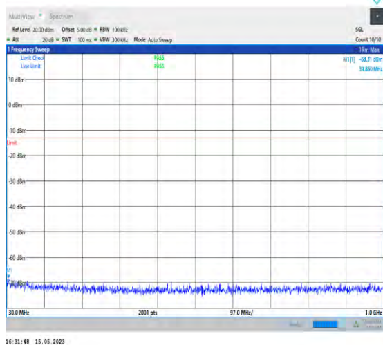
1-N77-3700-3980-PC1-30-100-L-1-DFT-PI2BPSK-In ner_1RB_Left-1@1-30-1000-Ant0-34.85--68.31--13-PASS
