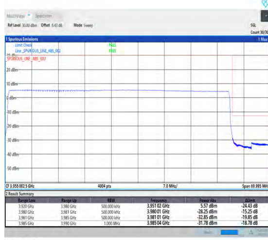
1-N77-3700-3980-PC1-30-60-H-6-CP-QPSK-Outer_Full-162@0-Ant0-1--PASS-see graph
