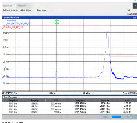
1-N77-3700-3980-PC1-30-40-H-2-DFT-PI2BPSK-Edge_1RB_Right-1@105-Ant0-1--PASS-see graph
