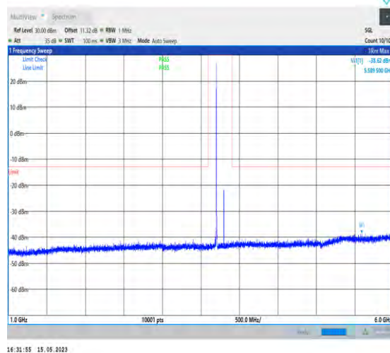
1-N77-3700-3980-PC1-30-100-L-1-DFT-PI2BPSK-In ner_1RB_Left-1@1-1000-6000-Ant0-5589.50--38.62--13-PASS
