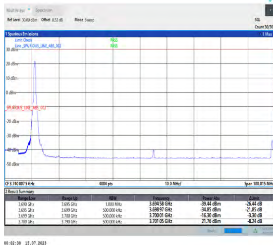
1-N77-3700-3980-PC1-30-90-L-1-DFT-PI2BPSK-Edg e_1RB_Left-1@0-Ant0-1--PASS-see graph
