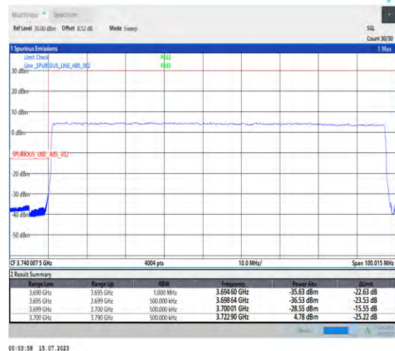
1-N77-3700-3980-PC1-30-90-L-3-DFT-PI2BPSK-O uter_Full-240@0-Ant0-1--PASS-see graph
