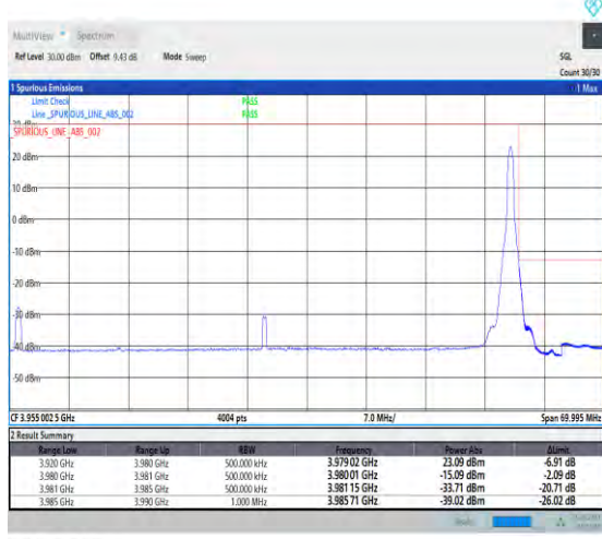
1-N77-3700-3980-PC1-30-60-H-5-CP-QPSK-Edge_1RB_Right-1@161-Ant0-1--PASS-see graph
