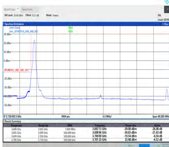
1-N77-3700-3980-PC1-30-50-L-4-CP-QPSK-Edge_1 RB_Left-1@0-Ant0-1--PASS-see graph
