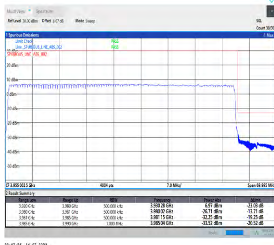
1-N77-3700-3980-PC1-30-60-H-3-DFT-PI2BPSK-Outer_Full-162@0-Ant0-1--PASS-see graph
