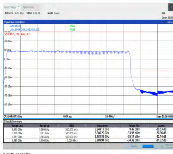
1-N77-3700-3980-PC1-30-40-H-3-DFT-PI2BPSK-Outer_Full-100@0-Ant0-1--PASS-see graph
