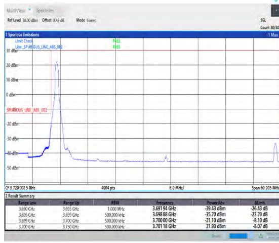
1-N77-3700-3980-PC1-30-50-L-1-DFT-PI2BPSK-Edg e_1RB_Left-1@0-Ant0-1--PASS-see graph
