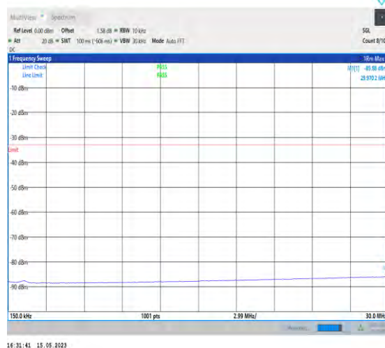
1-N77-3700-3980-PC1-30-100-L-1-DFT-PI2BPSK-In ner_1RB_Left-1@1-0.15-30-Ant0-29.97--85.88--33-P ASS
