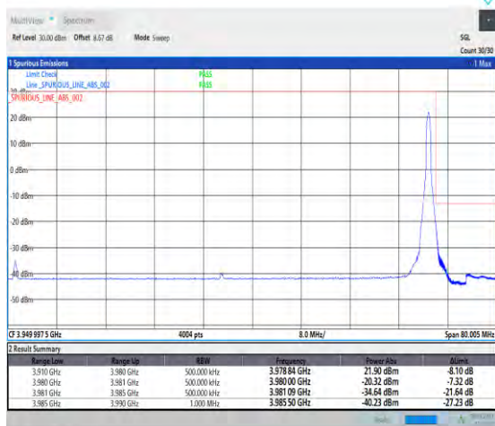
1-N77-3700-3980-PC1-30-70-H-2-DFT-PI2BPSK-Edge_1RB_Right-1@188-Ant0-1--PASS-see graph
