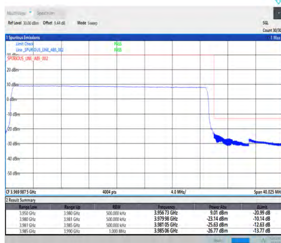
1-N77-3700-3980-PC1-30-30-H-6-CP-QPSK-Outer_Full-78@0-Ant0-1--PASS-see graph
