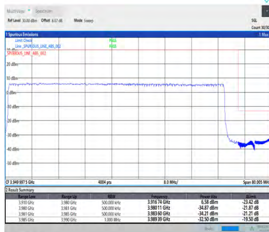
1-N77-3700-3980-PC1-30-70-H-3-DFT-PI2BPSK-Outer_Full-180@0-Ant0-1--PASS-see graph
