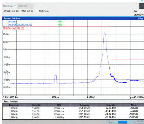
1-N77-3700-3980-PC1-30-30-H-2-DFT-PI2BPSK-Edge_1RB_Right-1@77-Ant0-1--PASS-see graph
