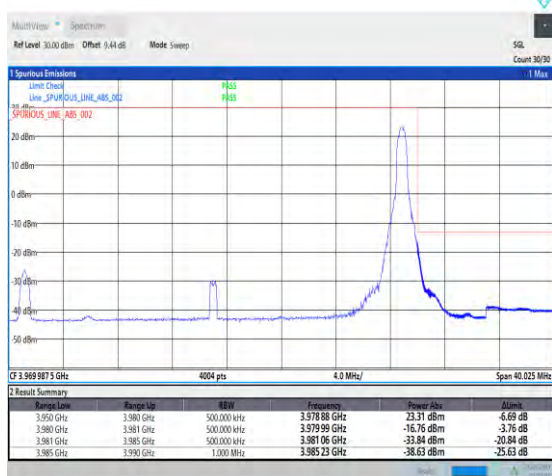
1-N77-3700-3980-PC1-30-30-H-5-CP-QPSK-Edge_1RB_Right-1@77-Ant0-1--PASS-see graph
