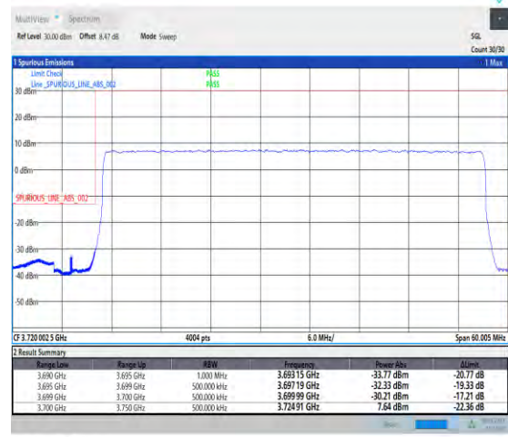
1-N77-3700-3980-PC1-30-50-L-3-DFT-PI2BPSK-O uter_Full-128@0-Ant0-1--PASS-see graph
