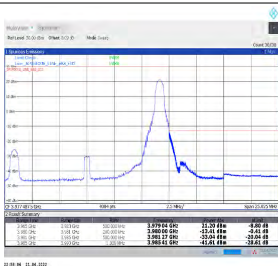
1-N77-3700-3980--30-15-H-2-DFT-PI2BPSK-Edge_1R B_Right-1@37-Ant0-PASS-see graph
