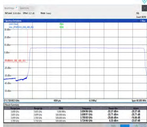
1-N77-3700-3980-PC1-30-50-L-6-CP-QPSK-Outer_ Full-133@0-Ant0-1--PASS-see graph
