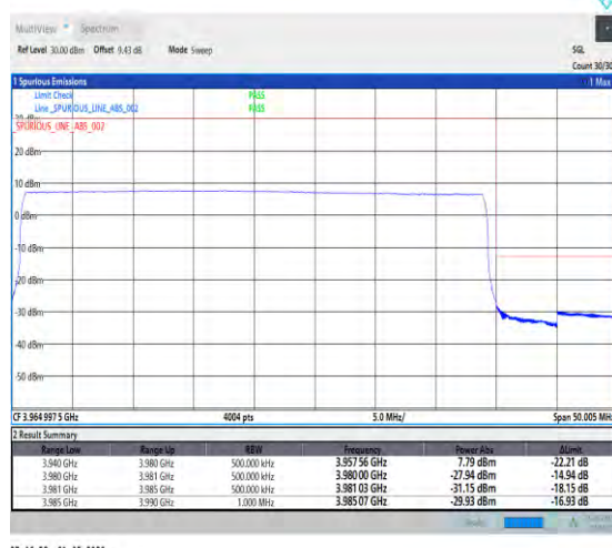
1-N77-3700-3980-PC1-30-40-H-6-CP-QPSK-Outer_Full-106@0-Ant0-1--PASS-see graph
