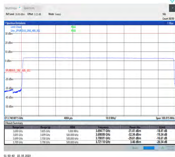
1-N77-3700-3980-PC1-30-90-L-6-CP-QPSK-Outer_ Full-245@0-Ant0-1--PASS-see graph
