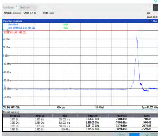
1-N77-3700-3980-PC1-30-70-H-5-CP-QPSK-Edge_1RB_Right-1@188-Ant0-1--PASS-see graph
