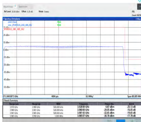
1-N77-3700-3980-PC1-30-70-H-6-CP-QPSK-Outer_Full-189@0-Ant0-1--PASS-see graph
