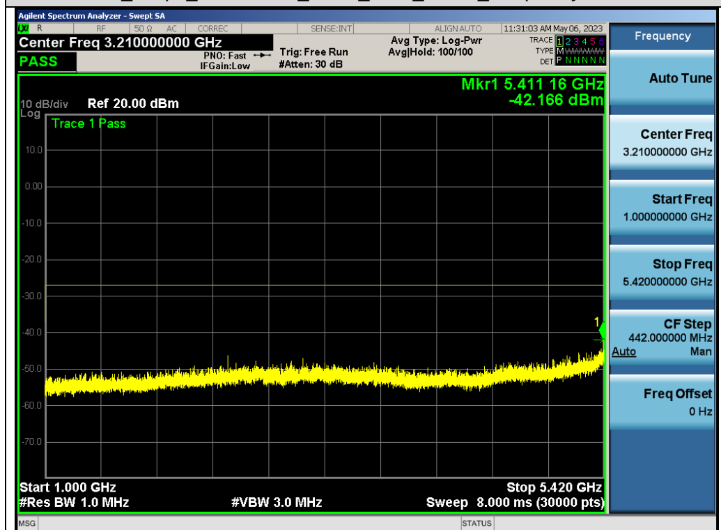
Test_Graph_802.11ac80_ANT2_5530_MCS0_Frequency Band 2
