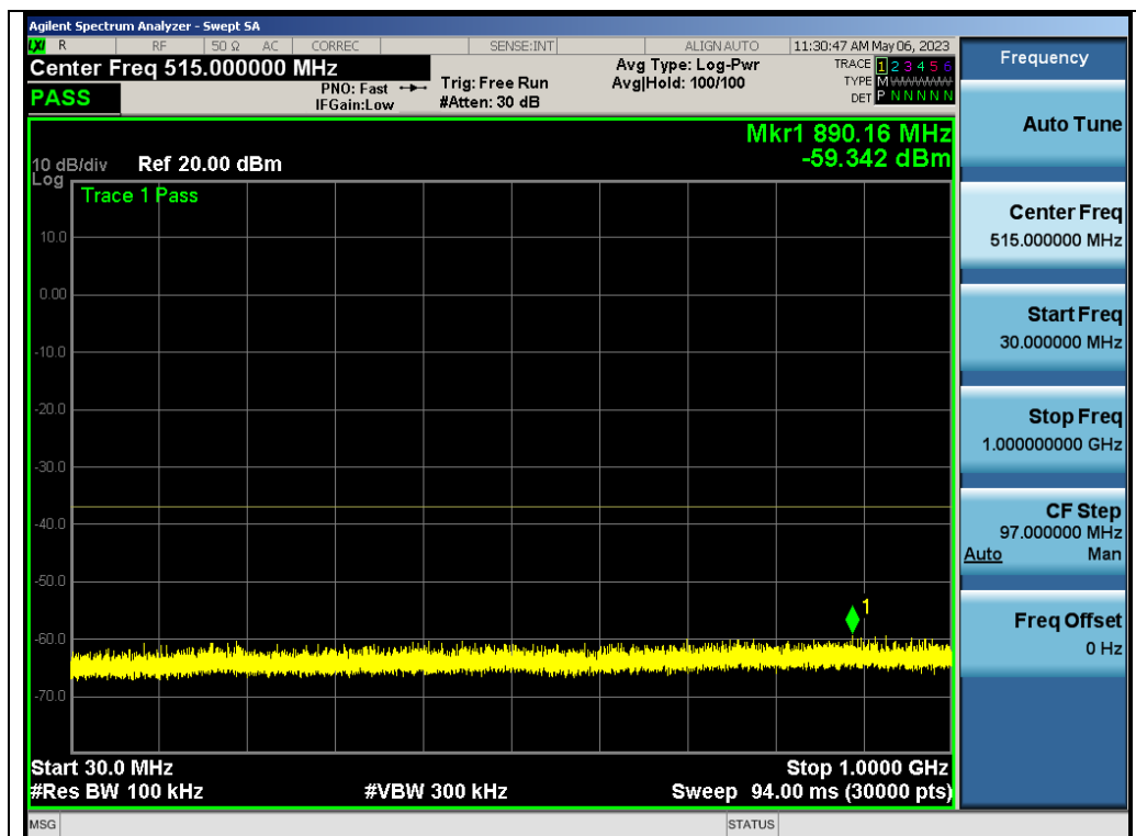
Test_Graph_802.11ac80_ANT2_5530_MCS0_Frequency Band 1
