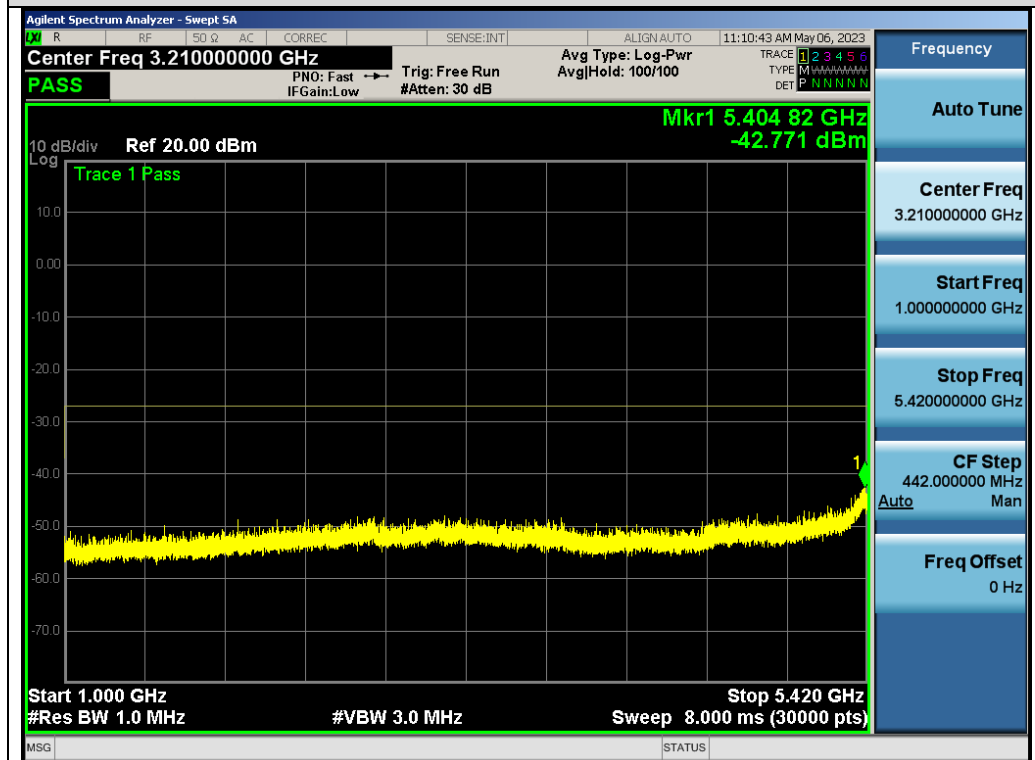
Test_Graph_802.11n40_ANT2_5510_MCS0_Frequency Band 2
