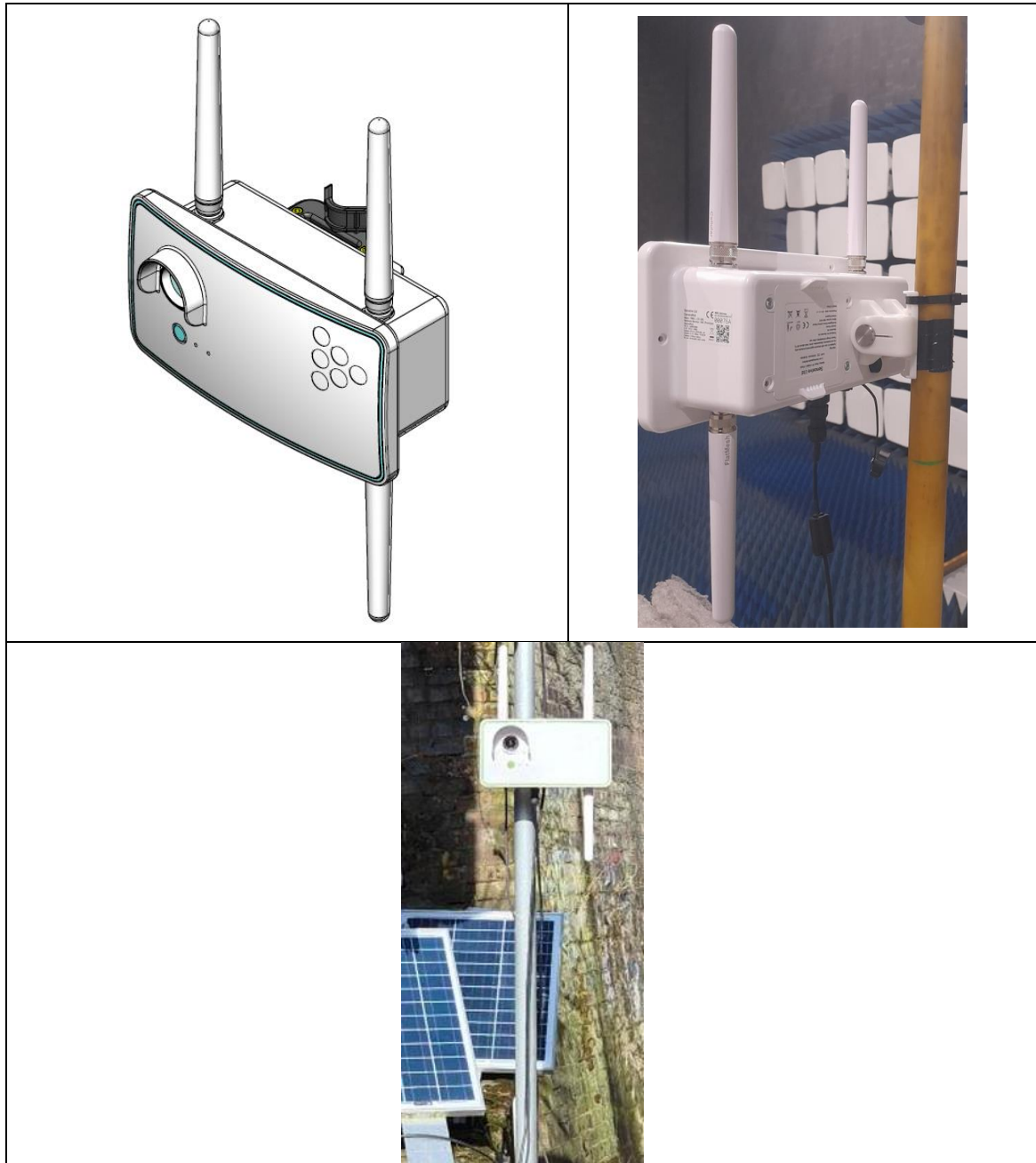
Figure 2.2: Camera Hubs with rear bracket and Pole Mounted.
