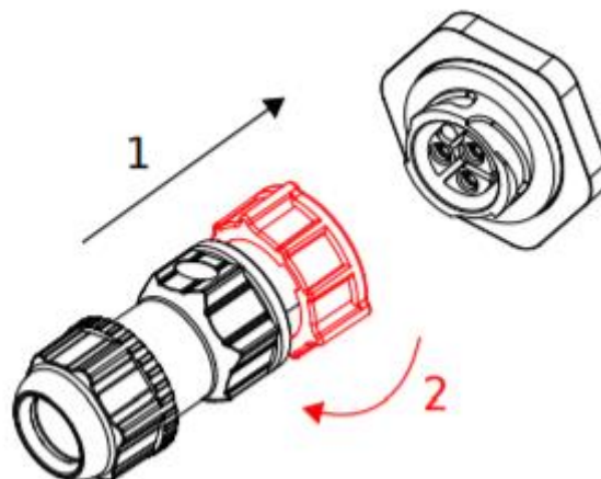
Figure 2.4: Image of the Camera Hub Power Connector
