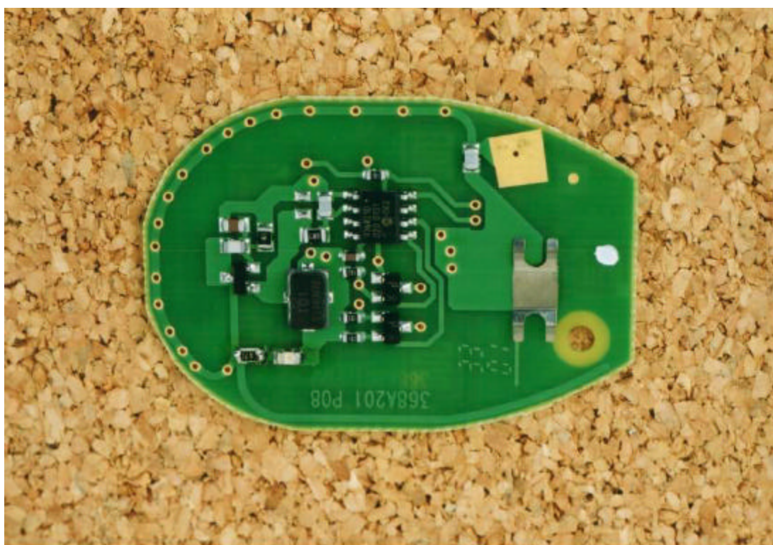
PCB, top
