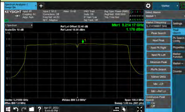
Channel 42 (5210MHz)
