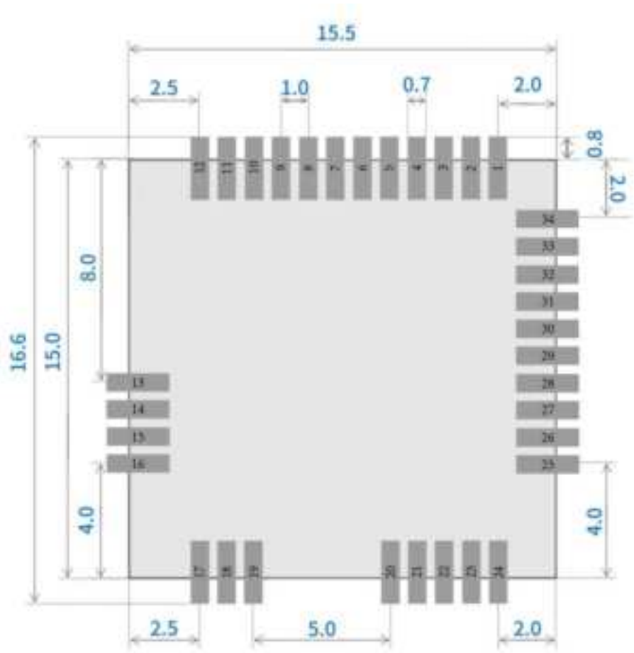
Figure 4: RAK11720 Layout
